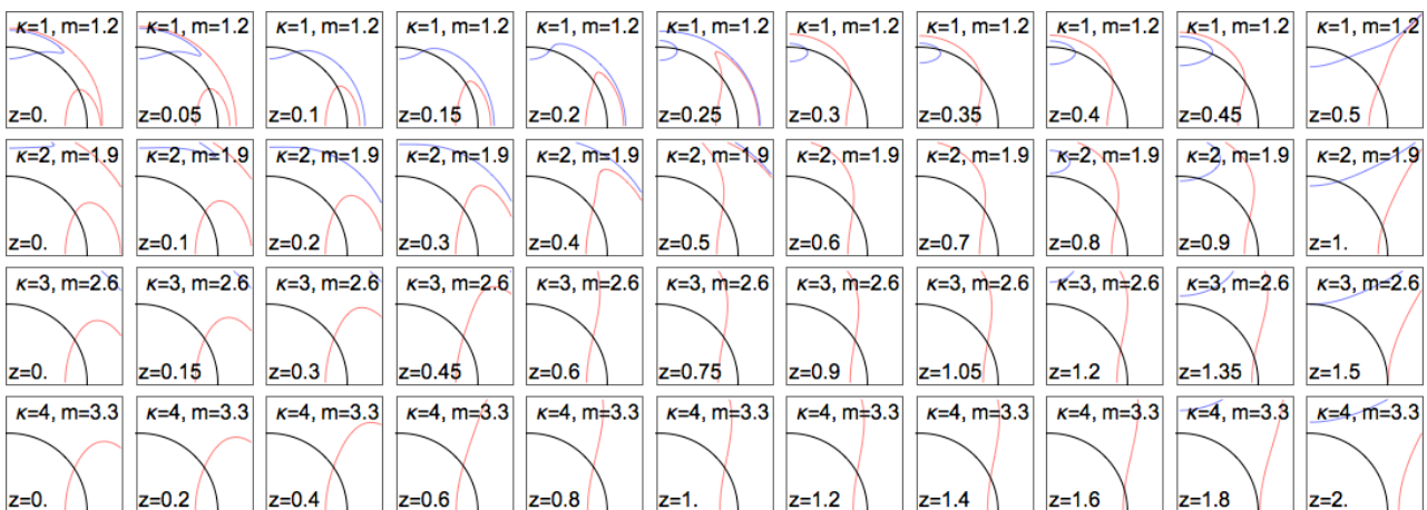
Figure 8: Vane cross sections along z axis for typical parameters Lc/a(=k) and m .
