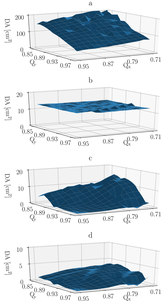
Figure 4: Comparison of DA for helions at |G\gamma| = 7.5 with: a) snakes off, no limiting aperture; b) snakes off with limiting aperture; c) snakes on, no limiting aperture; d) snakes on, with limiting aperture.
