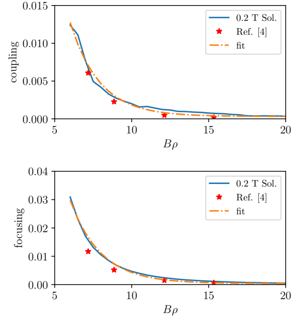
Figure 1: Coupling and focusing from the AGS cold snake as a function of B\rho and comparison to an exponential function.
