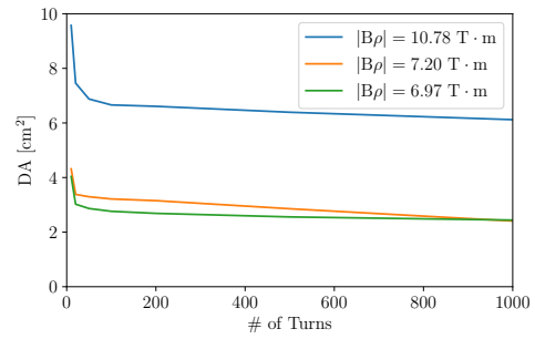
Figure 6: Comparison of DAs for the three configurations at [Q_x, Q_y] = [0.75, 0.91] and an increasing number of turns.
