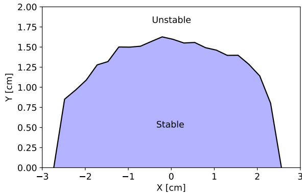
Figure 3: Example dynamic aperture in the AGS with \nu_x = 8.77 and \nu_y = 8.88 .
