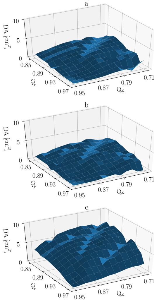
Figure 5: Dynamic aperture of AGS sorted by rigidity: a) helions at |G\gamma| = 7.5 , B\rho = 6.968 Tm; b) protons at |G\gamma| = 4.5 , helions B\rho = 7.203 Tm; c) |G\gamma| = 10.5 , B\rho = 10.780 Tm.
