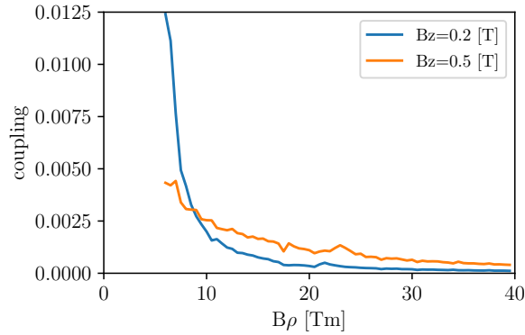
Figure 2: Figure showing the coupling error of the cold snake with a 0.2 T and a 0.5 T solenoid field with respect to B\rho .
