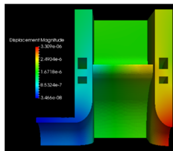
Figure 6: Displacement distribution at steady state.
