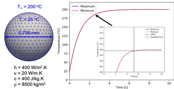
Figure 2: (Left) Simulation model and material properties; (Right) Maximum and minimum temperatures in sphere as a function of time, with insert showing agreement with analytical solution at a time step.
