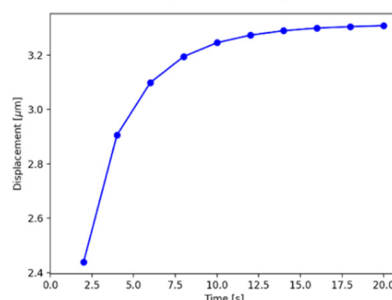
Figure 5: Evolution of maximum displacement of cavity.
