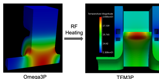
Figure 1: Temperature distribution in cavity enclosure due to rf fields of the cavity accelerating mode.
