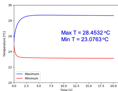
Figure 3: Evolution of minimum and maximum temperatures inside rf gun cavity.
