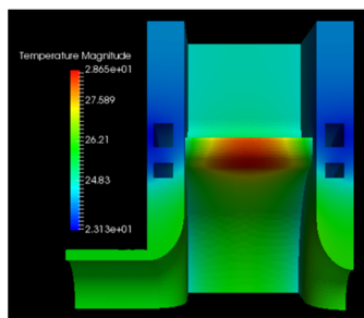
Figure 4: Temperature distribution at steady state.
