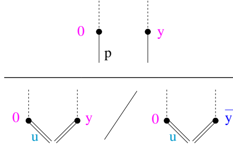
Fig. 10. Matrix element with subtractive regularization.
