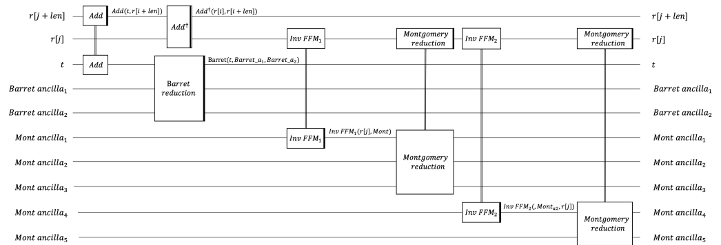
Figure 3. Process for the inverse NTT quantum circuit; \dagger indicates reversible gates.
