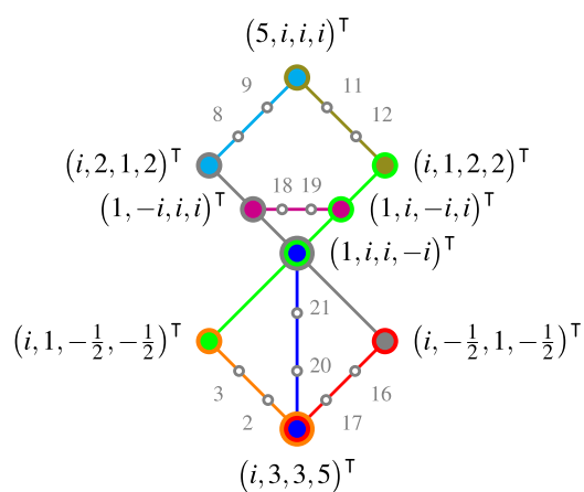
Figure 3. ‘Incomplete’ faithful orthogonal representation (aka coordinatization) of the orthogonality hypergraph of the Hardy gadget, as quoted from figure 1 and the last row of table I CC BY 4. Reproduced from [5]. CC BY 4.0.
