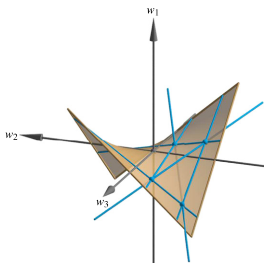
Figure 2. Tetrahedron arising from the basis (26).
