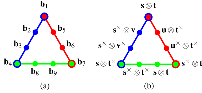
Figure 4. (a) Subgraph of the triangle hypergraph depicted in figure 3 with a faithful orthogonal representation by decomposable vectors \mathbf{b}_2, \mathbf{b}_3, \dots, \mathbf{b}_6 and arbitrary vectors \mathbf{b}_1, \mathbf{b}_7, \mathbf{b}_8, \mathbf{b}_9 . Even though it turns out that \mathbf{b}_1 and \mathbf{b}_7 must be decomposable, the remaining vectors \mathbf{b}_8 and \mathbf{b}_9 have to be indecomposable. (b) An explicit example of a non-faithful orthogonal representation of the triangle hypergraph with only decomposable vectors resulting in the multiple occurrence of \mathbf{s} \otimes \mathbf{t} .
