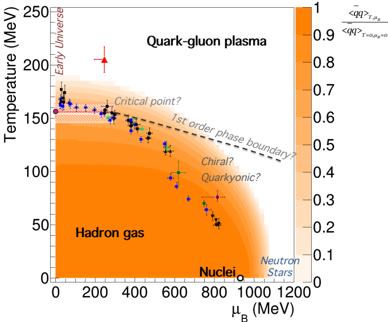
Fig. 1. (Colour on-line) Sketch of the phase diagram of QCD matter [1] including freeze-out data points in T and \mu_B describing the final-state hadron abundances in a statistical hadronization model (blue squares and pink circle from [6, 7], light green squares from [8], black solid symbols from [9], dark blue stars from [10], green circles [11], lila diamond [12], as well as the Lattice QCD results from [5] (white curve) and [4] (red curve)). The red triangle is extracted from the measured invariant-mass slope of dimuons in the mass range of 1.2 < M_{\mu\mu} < 2 GeV/ c^2 in the dimuon measurement in In+In collisions at \sqrt{s_{NN}} = 17.2 GeV [13]. The expectation value of the chiral condensate relative to the vacuum is depicted as shaded gray/orange region [2].
