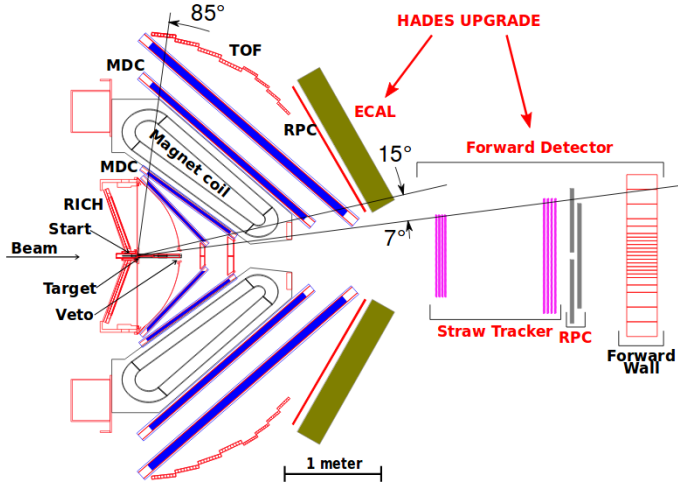
Fig. 2. Schematic side view of the HADES detector showing its compact design. The detectors are symmetrically arranged in the azimuthal angle around the beam axis. The distance to the target of the forward wall is typically 6 m.
