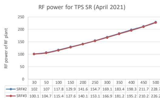
Figure 1: The measured RF power requirement versus of beam current of 2 RF plants for TPS storage ring in April 2021.
