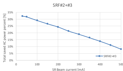
Figure 8: The saved AC power percentage of sum of both RF system as a function of storage beam current.
