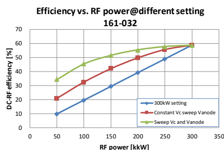
Figure 4: DC-RF efficiency of klystron by three different setting method: 1 sweeping both cathode and anode voltage, 2 sweeping anode voltage only, 3 constant 300 kW setting.
