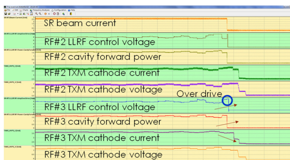
Figure 6: Both RF plants in power saving operation controlling both cathode and anode voltage would cause RF power racing in between and lead to system protection trip.
