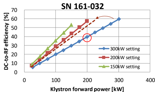
Figure 2: The DC-to-RF conversion efficiency as a function of klystron output power in 3 parameters settings of one klystron.
