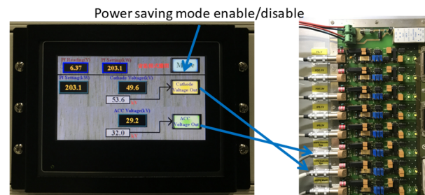
Figure 5: The man-machine interface touch panel can display the read klystron RF forward power and the output analogue signals which control the operation high voltages of klystron.
