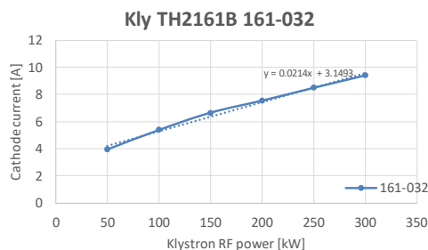
Figure 3: The maximum available RF power versus cathode current.
