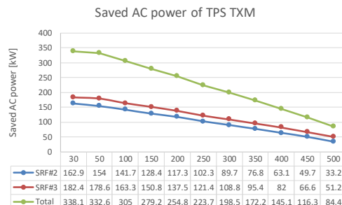
Figure 7: The saved AC power of both RF plants as a function of storage ring beam current.
