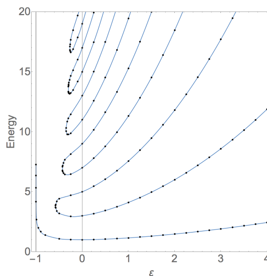
Figure 1. Energy levels of the parametric family of Hamiltonians H = p^2 + x^2(ix)^\varepsilon . Note that when \varepsilon \geq 0 , the eigenvalues are all real and positive, and they increase with increasing \varepsilon . When \varepsilon decreases below 0, the eigenvalues disappear into the complex plane as complex conjugate pairs. Eventually, only one real eigenvalue remains when \varepsilon is less than about -0.57 , and as \varepsilon approaches -1 from above, this eigenvalue becomes infinite. The region \varepsilon \geq 0 in which the eigenvalues are all real is called the region of unbroken \mathcal{PT} symmetry and the region \varepsilon < 0 in which some of the eigenvalues are complex is called the region of broken \mathcal{PT} symmetry . The transition point between these two regions is called the \mathcal{PT} phase transition , and this transition has been observed in many published laboratory experiments.
