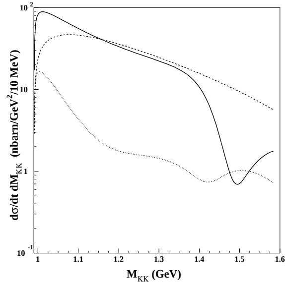
Fig. 2. S -wave K^+K^- invariant mass distribution. The dotted line represents the result with no \pi\pi coupling, for description of other lines see Fig. 1.
