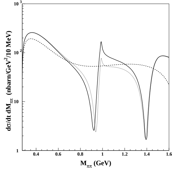
Fig. 1. S -wave \pi^+\pi^- invariant mass distribution. The solid line shows the full FSI result (on-shell and off-shell) with both \pi\pi and K\bar{K} intermediate channels, the dotted line represents the result with no K\bar{K} coupling and the dashed line corresponds to the Born cross section.
