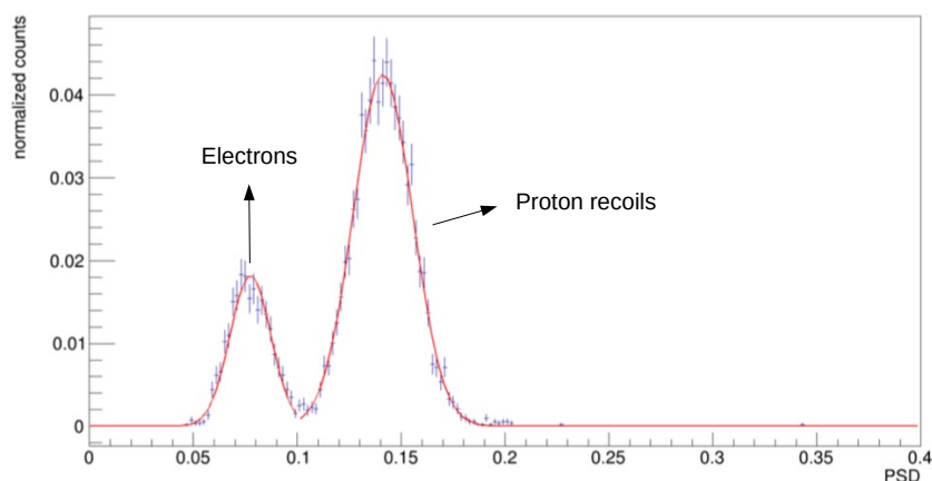
Figure 3. Distribution of the PSD parameter for a LS standard (LAB, PPO and POPOP) with a FoM_{\max} of 1.18.
