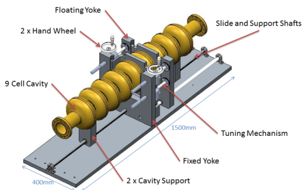
Figure 5: Mechanical cavity tuning fixture.
