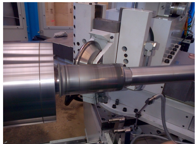
Figure 1: Niobium beam-pipe spinning.
