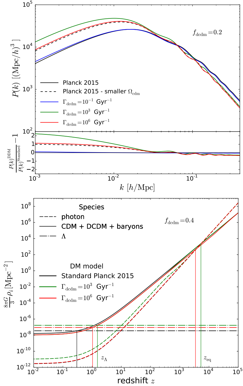
Figure 39: Top panel – Comparison of the matter power spectrum for several decaying DM lifetimes and a fixed abundance f_{\text{dcdm}} = 0.2 . Bottom panel – Evolution of the background densities for two different models of DM with f_{\text{dcdm}} = 0.4 , compared to the standard \Lambda CDM model. The vertical lines indicate the value of the matter-radiation and matter- \Lambda equalities in each model. Note that matter-radiation equality happens at the same redshift in the standard \Lambda CDM and the DCDM model with \Gamma_{\text{dcdm}} = 10^3 \text{ Gyr}^{-1} , therefore lines are superimposed.
