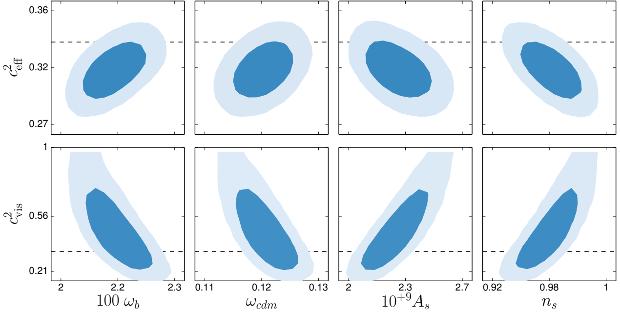
Figure 81: Degeneracies between the parameters (c_{\text{vis}}^2, c_{\text{eff}}^2) and the parameters \omega_b , \omega_{cdm} , A_s and n_s . A combination of CMB+lensing data is used for this plot, in which a \Lambda\text{CDM}+c_{\text{vis}}^2+c_{\text{eff}}^2 model is assumed. Dashed lines correspond to the standard values (c_{\text{eff}}^2, c_{\text{vis}}^2) = (1/3, 1/3) .
