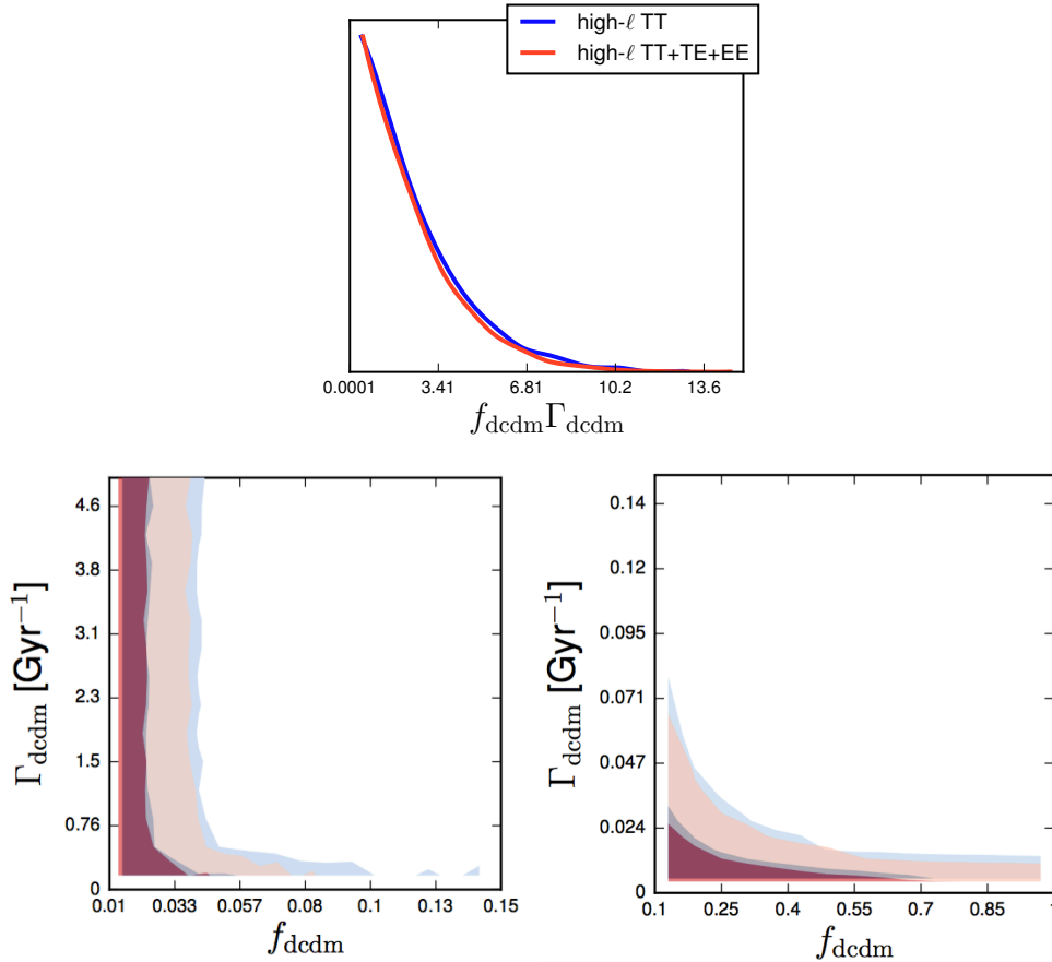
Figure 41: Constraints on the decaying dark matter fraction f_{\text{ddm}} as a function of the lifetime \Gamma_{\text{ddm}} in the long-lived and intermediate regime. All datasets also include CMB low- \ell data from each spectrum and the lensing reconstruction. Blue (red) lines and contours refer to the case without (with) high- \ell polarization data. Inner and outer coloured regions denote 1\sigma and 2\sigma contours, respectively.
