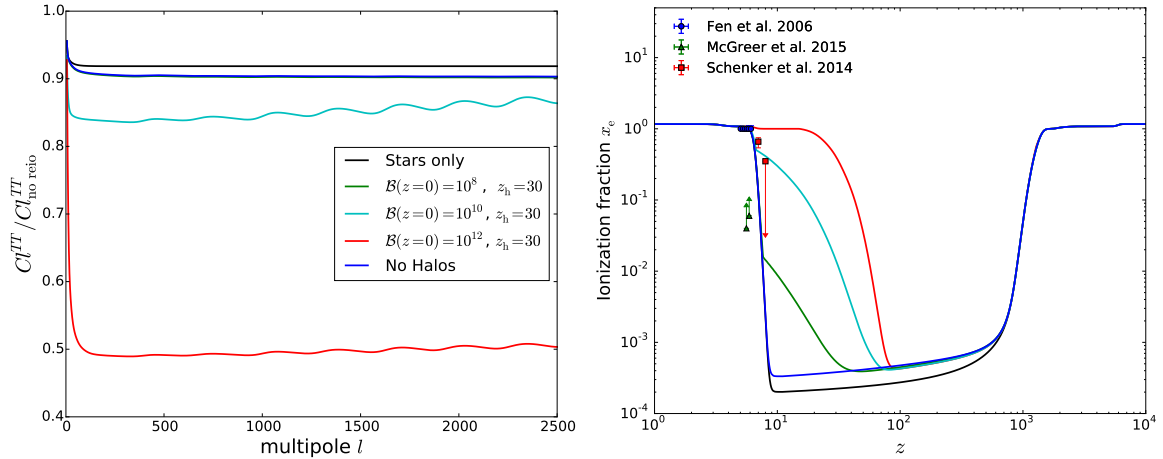
Figure 95: Left pannel - Comparison of the CMB temperature power spectrum for several mixed star-DM reionization models, with z_{\text{reio}} = 6.5 and a DM particle of 1 GeV annihilating into electrons, normalized to the CMB power spectrum in a universe without reionization. Right pannel - The corresponding ionization histories.
