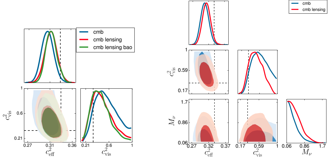
Figure 82: Left. Constraints in the (c_{\text{vis}}^2, c_{\text{eff}}^2) plane for combination of CMB, CMB+lensing and CMB+lensing+BAO data, in the \Lambda\text{CDM} + c_{\text{vis}}^2 + c_{\text{eff}}^2 model. Marginalised posterior distributions for both parameters are also shown. Right. Constraints on (c_{\text{vis}}^2, c_{\text{eff}}^2) and the total neutrino mass M_\nu for CMB and CMB+lensing datasets in the \Lambda\text{CDM} + c_{\text{vis}}^2 + c_{\text{eff}}^2 + m_\nu model. Dashed lines correspond to the standard values (c_{\text{eff}}^2, c_{\text{vis}}^2) = (1/3, 1/3) .
