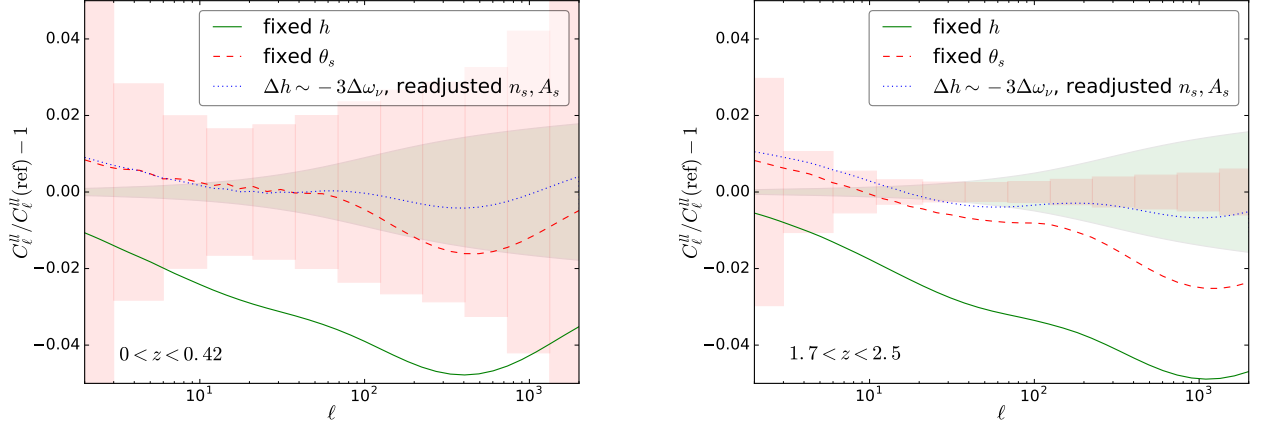
Figure 90: Relative error on the galaxy lensing C_\ell^{\text{II}} in the first redshift bin ( 0 < z < 0.42 , left panel) and in the tenth redshift bin ( 1.7 < z < 2.5 , right panel). Here the redshift range is 0 < z < 2.5 and is divided in ten equi-populated redshift bins. The light pink rectangles refers to the observational error. The light green shaded area shows the relative error associated to our model for the theoretical uncertainty on P_m(k, z) . Green solid and red dashed lines are the same as in figure 85, i.e. higher M_\nu with fixed h (green solid line) and higher M_\nu with fixed \theta_s and varying h (red dashed line). The blue dotted line, besides the higher M_\nu , implies a smaller value of h ( \Delta h \sim -3\Delta\omega_\nu ), an increase of n_s by 0.4% and of A_s by 2%.
