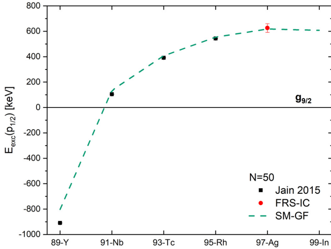
Fig. 3. Excitation energy of the 1/2^- isomeric state in odd-even N = 50 nuclei. The excitation energy measured with the MR-TOF-MS at the FRS Ion Catcher is shown as a red circle. In addition, the values taken from the atlas of nuclear isomers [42] are shown by black squares, and SM-GF calculations [55] by the green dashed line. The ^{89}\text{Y} value is negative because it is still in the \pi p_{1/2} sub-shell and 1/2^- is the ground state.
