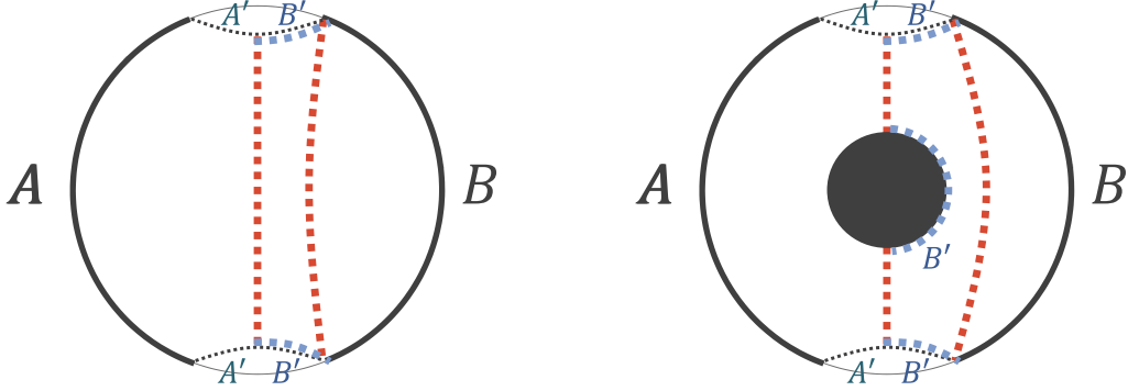
Figure 5.4: The E_M in the pure global \text{AdS}_3 (Left) and in the global BTZ (Right). The subsystems are taken as two disjoint intervals. (The figure is cited from [63])
