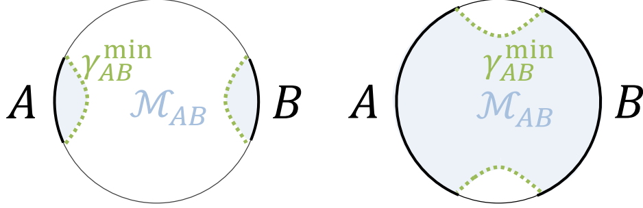
Figure 2.2: The Ryu-Takayanagi surface of S_{AB} in the two different configurations (Left and Right). The configuration that has smaller area of \gamma_A^{\min} will be chosen. The blue shaded region is the (time slice of) entanglement wedge of A \cup B .
