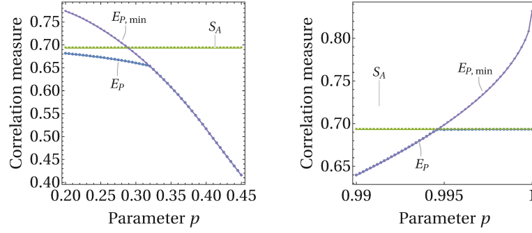
Figure 7.4: The detailed structure of the entanglement of purification for the Werner states of 0.2 \leq p \leq 0.45 (left) and 0.99 \leq p \leq 1 (right). There is a very tiny gap S_A > E_P(A : B) in the phase (d) (except p = 1 ), though it is hard to observe them in the plot. (The figure is cited from [61])
