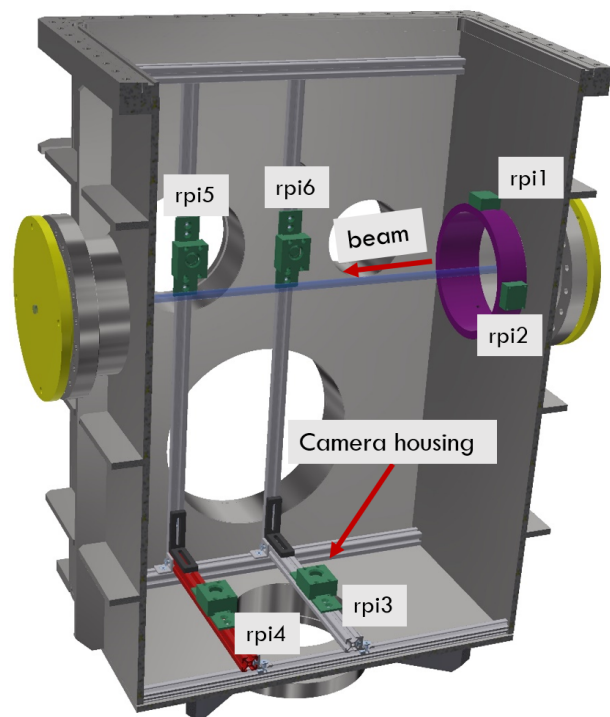
Figure 1: The image shows the first diagnostic chamber after the first solenoid in the FRANZ LEBT section. Six cameras are mounted along the beamline for continuous beam position determination.
