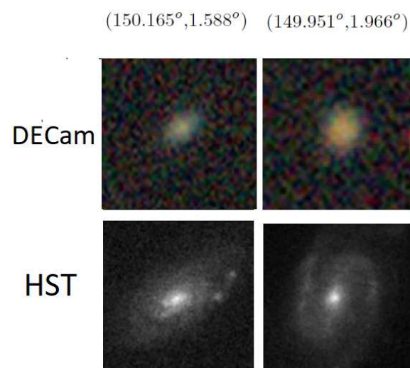
Figure 2. Galaxies imaged by DECam and the same galaxies imaged by the Hubble Space Telescope. The spin direction is clear in the HST images, but it is not clear in the DECam images.
