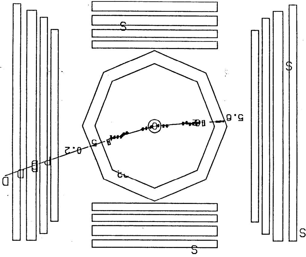
Fig. 4-12. - c) An e^+\mu^- event which results from the production of \tau^+\tau^- as discussed in the text.
