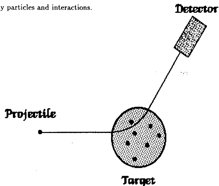
Fig. 4-1. - A projectile strikes a target, is deflected, and is observed in a detector.
