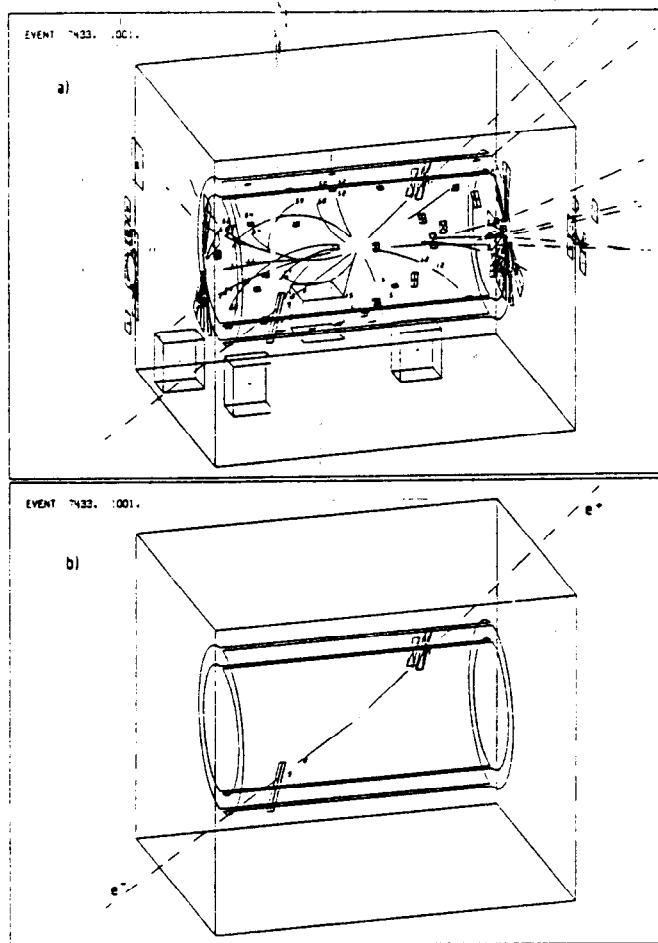
Fig. 5-10. A display of an event containing a Z that decays into e^+e^- . The top figure shows tracks of many of the particles produced in the collision of the proton and antiproton. The lower figure shows only those tracks with large momentum transverse to the direction of the colliding beams. By observing a number of such events, experimenters at CERN were able to demonstrate the existence of the Z . [UA-1 Collaboration, Phys. Lett. 126B , 398 (1983)]
