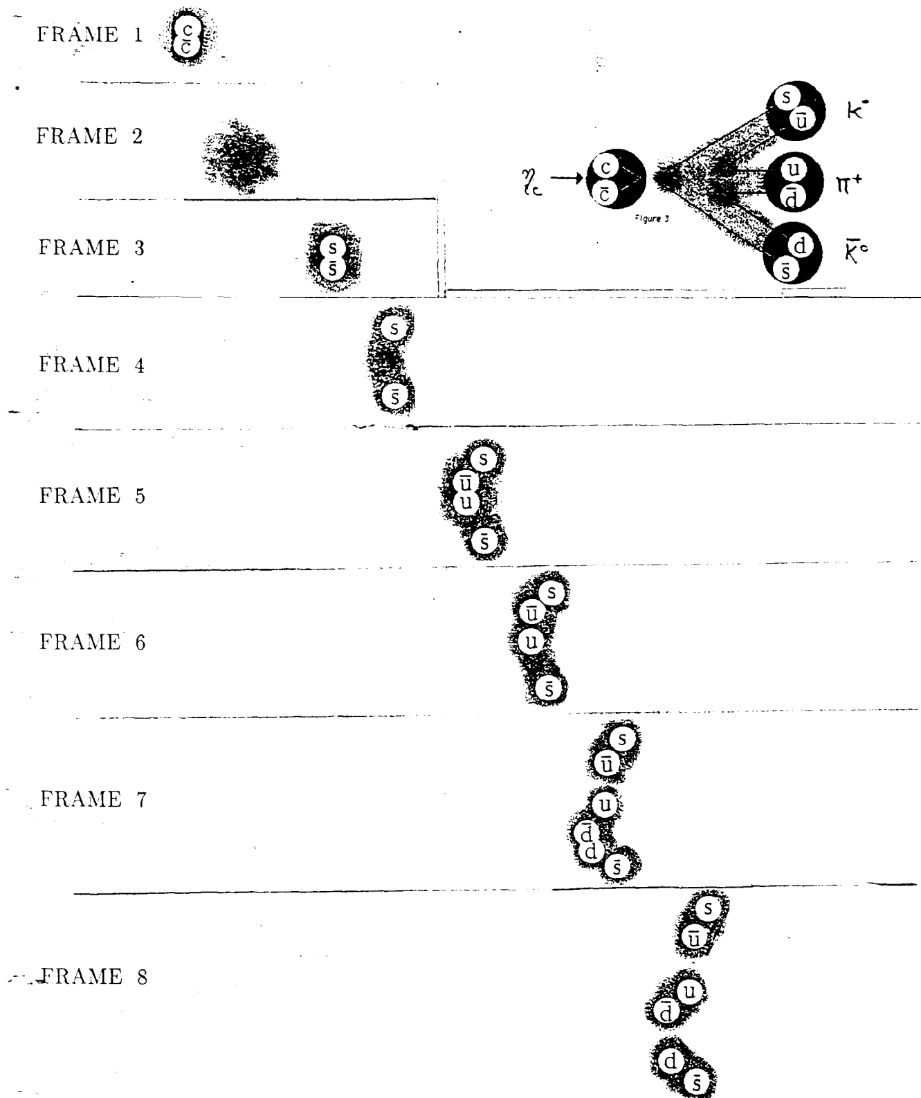
\eta_c \rightarrow \pi^+ K^0 K^- - Time lapse sequence for the quarks in an \eta_c meson to annihilate resulting in production of a pion and two K mesons.
