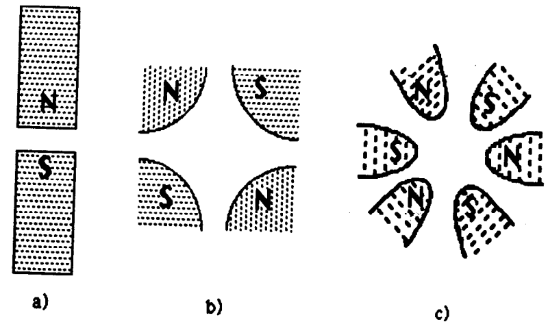
Fig. 4-6 Various magnet configurations. a) dipole. b) quadrupole. c) sextupole.
