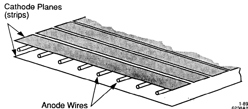
Fig. 4-9. - A portion of a multi-wire proportional chamber is shown illustrating the position of the anode wires which collect the avalanche of electrons produced in the gas when a particle traverses the device.
