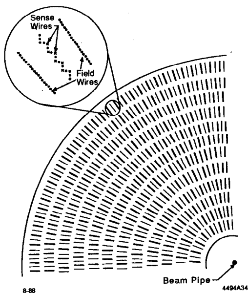
Fig. 4-10. - b) A quadrant of the end-plate of the large, cylindrical drift chamber used in the MARK II detector. A blowup region shows the position of the field wires and the sense wires for a single "cell".
