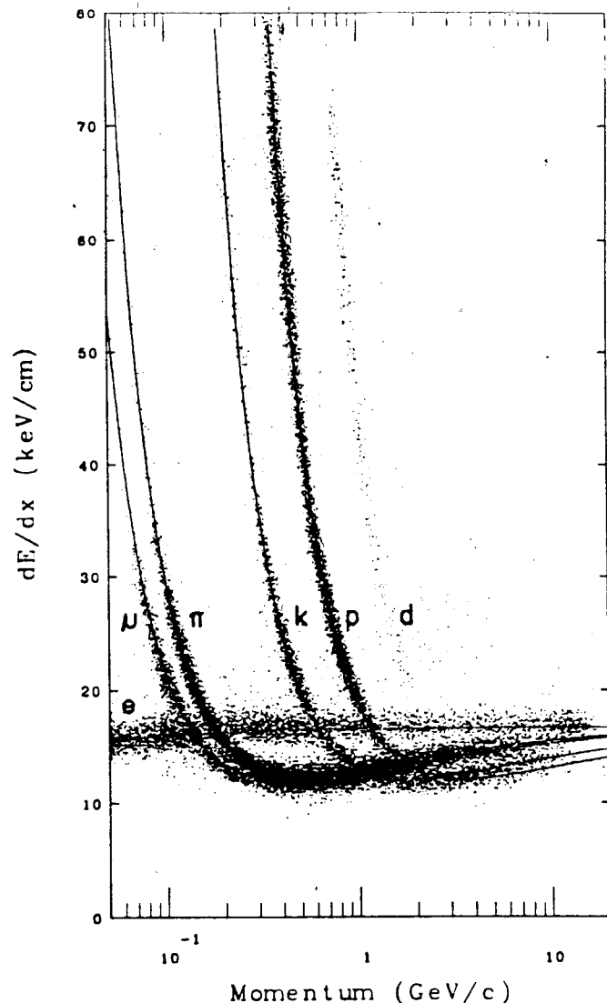
Fig. 4-7. - The energy lost per unit length in a gaseous drift chamber is plotted as a function of the charged particle's momentum (dots). The curves are the theoretical expectation for the particle types indicated on the figure namely electrons, muons, pions, kaons, protons and deuterons. This data is taken from the TPC detector at PEP.
