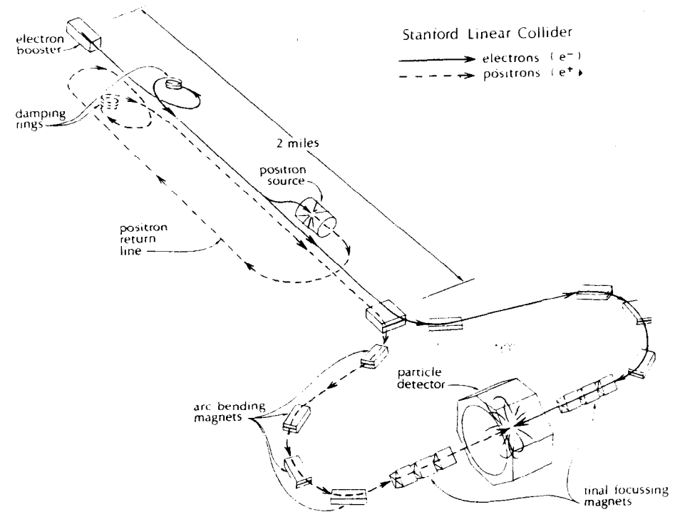
Fig. 4-4 - Schematic diagram of the SLC. (Drawing by Walter Zawojski.)
