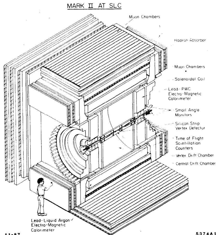
Fig. 4-11. - An drawing of a typical colliding beam detector. The major components are discussed in the text.
