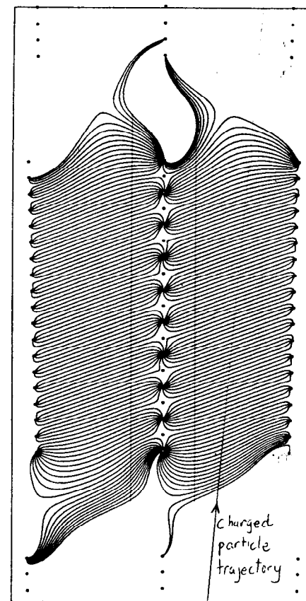
Fig. 4-10. - c) The paths taken by the electrons as they drift towards the sense wires are shown. Electrons liberated along the particle trajectory follow these drift lines to the sense wire.
