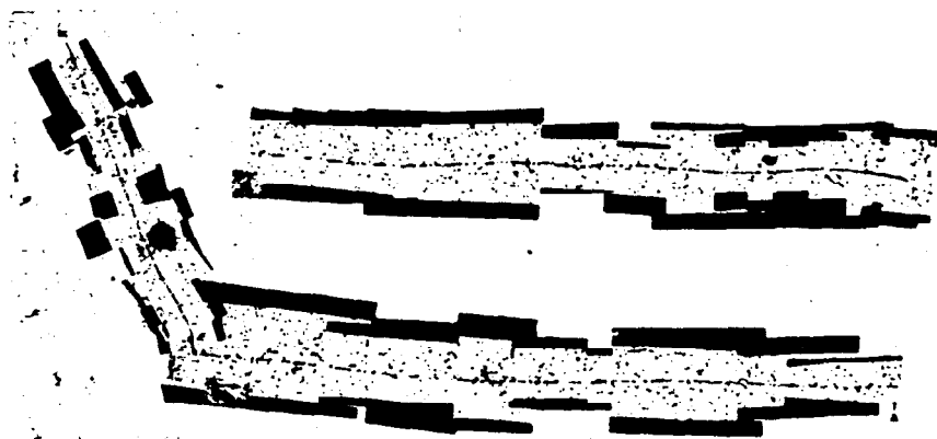
Fig. 5-3. A picture of a photographic emulsion showing a \pi^+ meson coming to rest (from upper left corner). The \pi^+ \rightarrow \mu^+ + \nu reaction occurs and the \mu^+ goes off to the right (continued above) and also comes to rest. The \mu^+ also decays to an e^+ and neutrinos. This emulsion was, however, not sensitive enough to record the e^+ (and neutrinos are not observable in such experiments). [C. M. G. Lattes et al. , Nature 159 , 694 (1947)]
