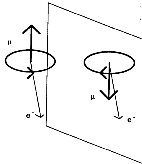
Fig. 5-5. A nucleus with spin in front of a mirror. The mirror image has its spin and magnetic momentum pointing opposite that of the real nucleus. If there is a correlation between the direction of the magnetic moment and the direction of the outgoing electrons from \beta decay, the correlation in the mirror will be the opposite. Thus it will be possible to distinguish between the real experiment and its mirror image. C. S. Wu and her co-workers found such a correlation and thus demonstrated that parity is not conserved.
