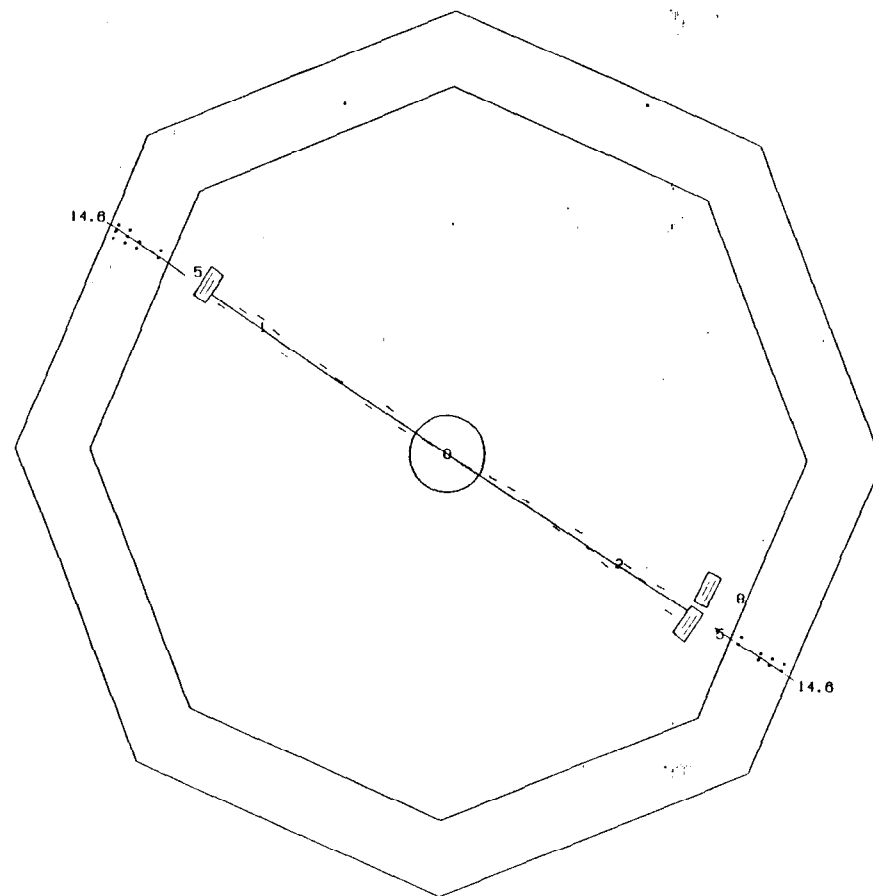
Fig. 4-12. - a) An e^+e^- final state. Two high-momentum, back-to-back tracks with momenta measured as 14.5 and 14.2 GeV/c each depositing 14.6 GeV of energy in the calorimeter. The beam energy in this run was 14.5 GeV.
