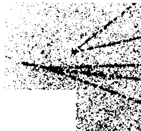
Fig. 5-9. A bubble chamber picture of the production and decay of a charmed particle and an anticharmed particle. One particle is charged and makes a track that splits into three tracks at the decay point. The other particle is neutral and decays into two charged particles. The particles were produced at SLAC by directing a beam of 20 GeV photons at the bubble chamber. The charmed particles were both created at the left end of the track of the charged charmed particle. [K. Abe et al., Phys. Rev. Lett. 48 , 1526 (1982)]
