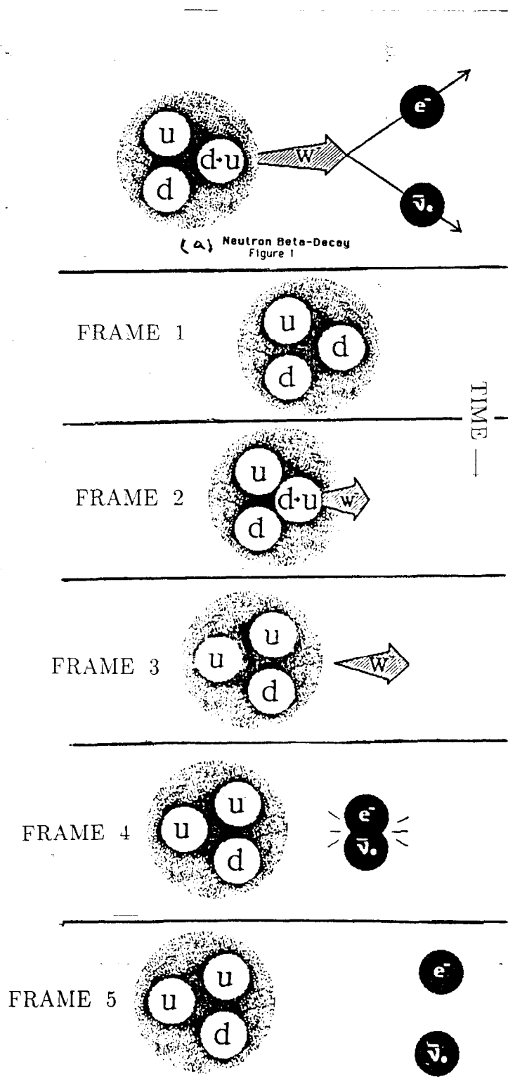
n \rightarrow pe^- \bar{\nu}_e - Time lapse pictures showing the sequence of events in neutron \beta -decay.
