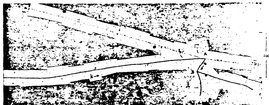
Fig. 5-4. The decay of a K^+ to \pi^+\pi^+\pi^- . The picture is of a photographic emulsion exposed to cosmic rays that was sensitive to charged particles. The K^+ entered along the path labeled k . At the point A , the K^+ decayed into three charged particles. The \pi^- interacted with a nucleus at the point B . [R. Brown et al. , Nature 163 , 82 (1949)]
