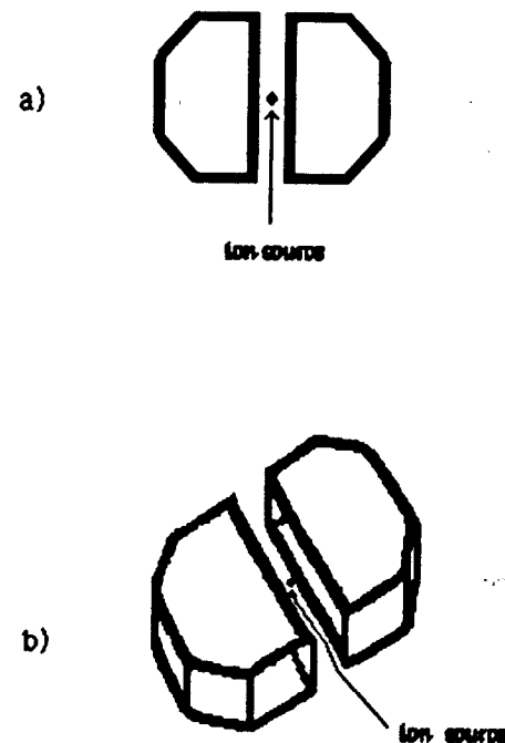
Fig. 4-5 The dees of the cyclotron developed by E. O. Lawrence. a) Top view. b) Perspective view. There is a magnetic field perpendicular to the top of the dees.
