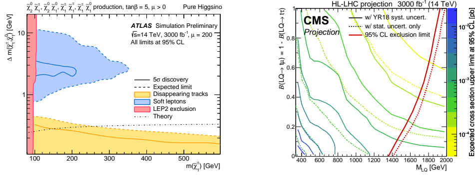
Figure 6: a) Expected 95% CL exclusion / discovery reach from disappearing-track and low-momentum lepton pair searches in higgsino-like electroweakino models (from 1) ), b) Expected upper limits on the LQ pair-production cross section at 95% CL as function of LQ mass and branching fraction (from 1) ).
