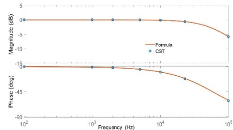
Figure 5: Frequency characteristics of the vacuum chamber.
