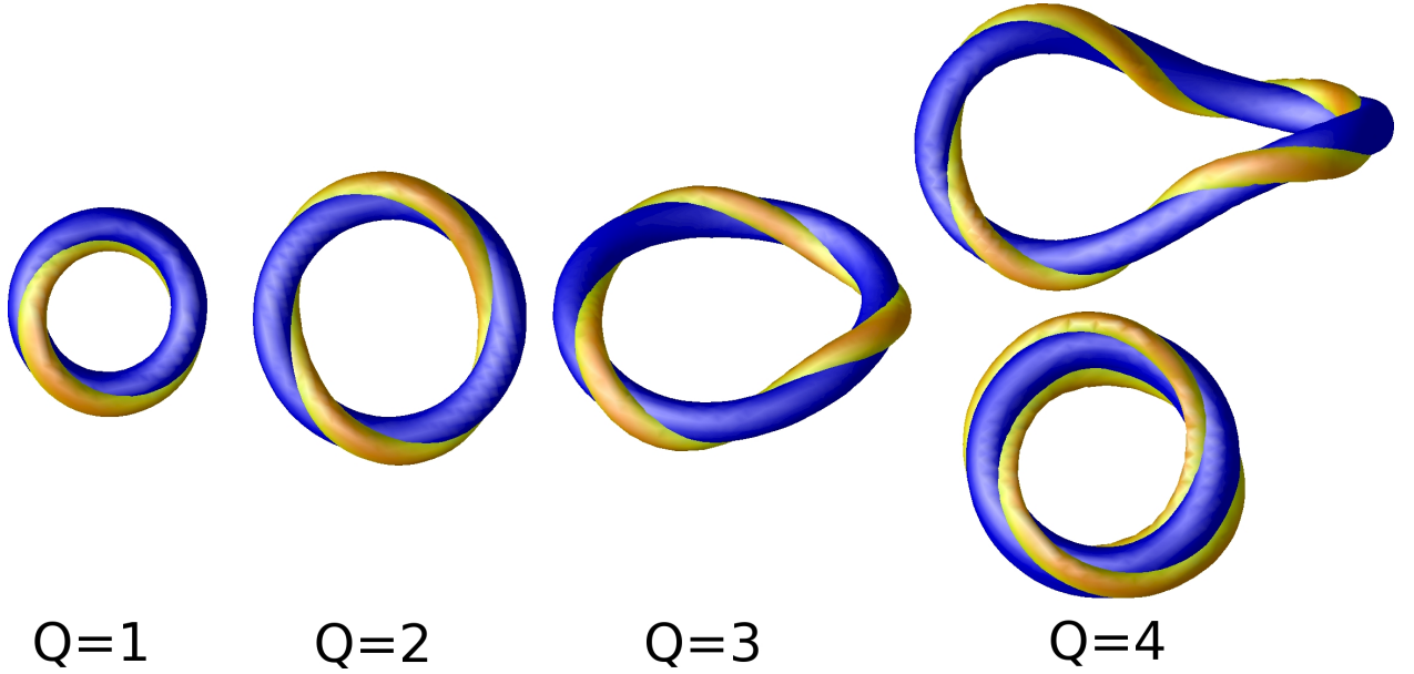
Figure 5.4: Minimum energies for m = 5 , Hopfions.
