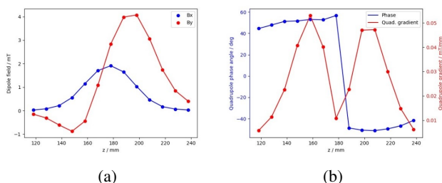
Figure 6: Dipole field (a) and quadrupole gradient and phase (b) at different measurement planes for 4.0 A solenoid current.
