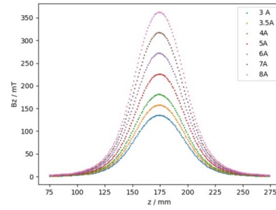
Figure 3: SC Solenoid longitudinal field on axis for different coil currents.
