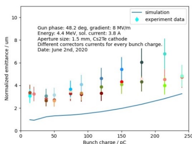
Figure 7: Normalized emittance vs. bunch charge. The spots with different colors are experiment data with different correctors current.
