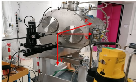
Figure 2: Cryomodule with SC solenoid and a 1D Hall magnetic field detector.
