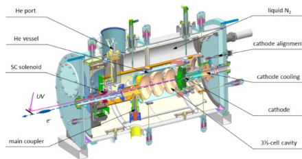
Figure 1: The current ELBE SRF Gun II and the SC solenoid in the cryomodule.
