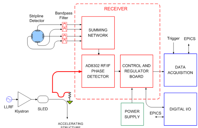
Figure 1: Block Diagram of AD8302 phase detector board (denoted by red dashes) showing bpm and linac rf phase reference inputs and EPICS output.
