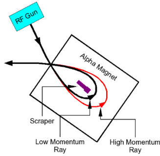
Figure 2: Diagram showing how rf gun power affects arrival time via alpha magnet dispersion.
