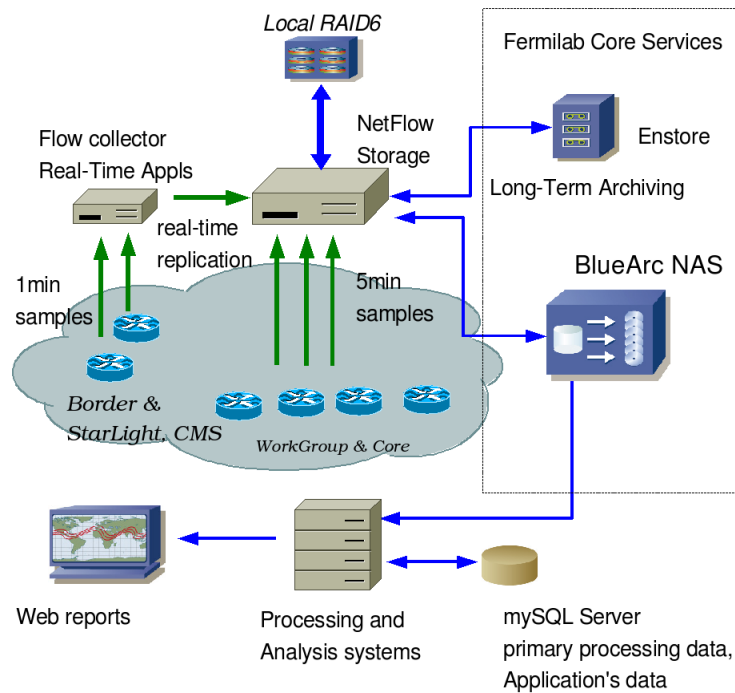
Figure 1: Distributed flow collection and analysis system
