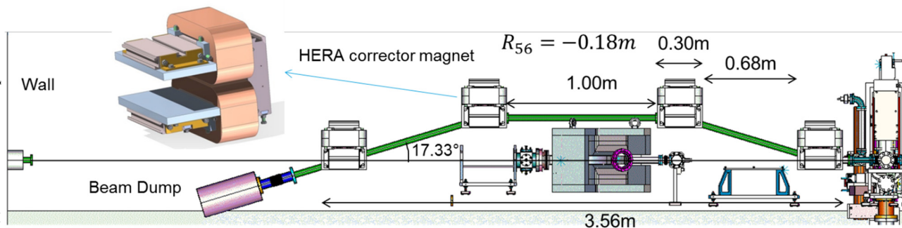
Figure 1: End-section of PITZ beamline in the main tunnel including the vertical chicane and the rotated beam dump.
