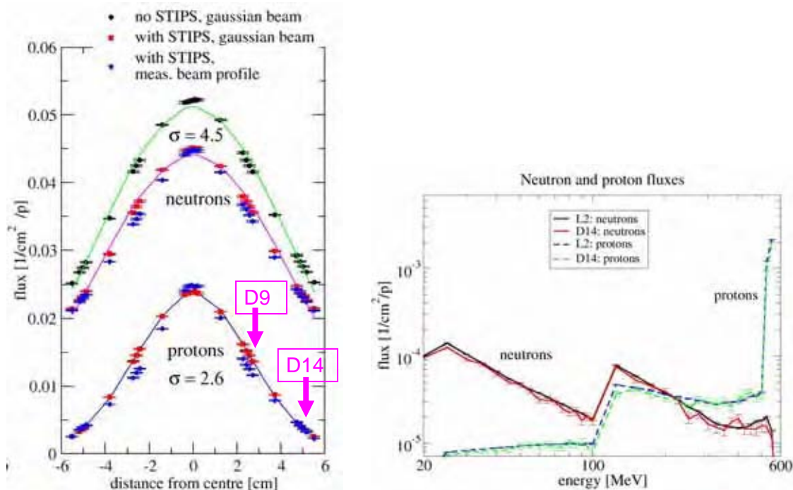
Figure 3: Left: Proton and neutron flux distribution in Rod3. The positions of the samples D9 and D14 are indicated. Right: Neutron and proton fluxes in the D14 sample and rod L2. The fluxes are normalised to one primary proton.
