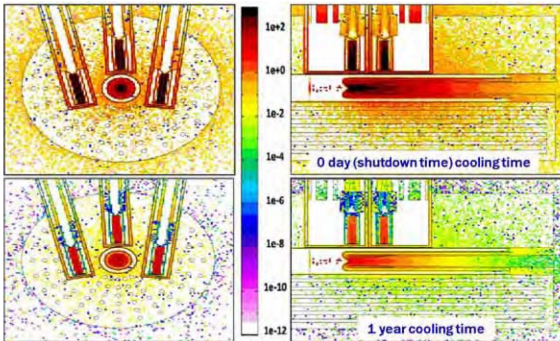
Figure 4: Activities ( \text{Ci}\cdot\text{g}^{-1} ) after shutdown. Decay contribution after 200 days of irradiation (4 MW power proton beam).
