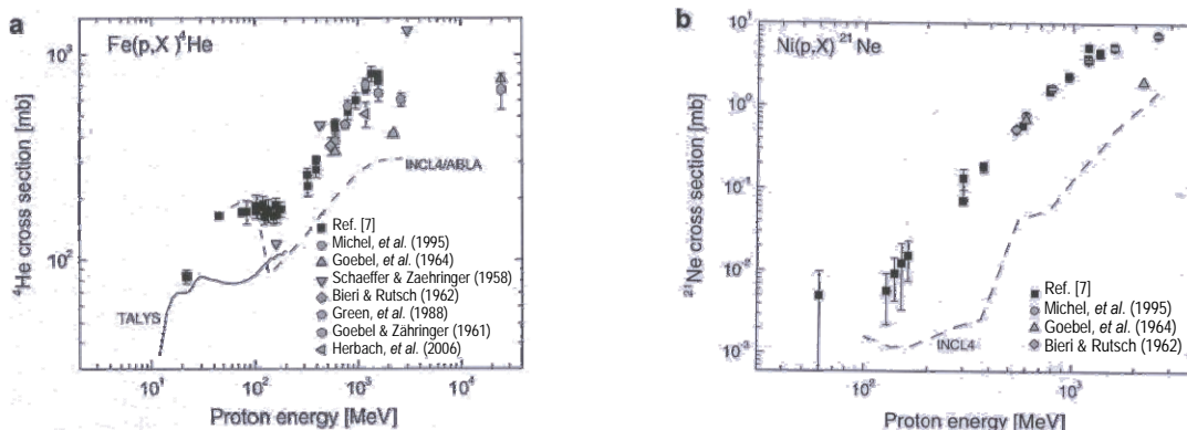
Figure 1: Alpha excitation function with proton on Fe on the left and ^{21}\text{Ne} excitation function with proton on Ni on the right. INCL4.2-AblV3p results are plotted in dashed line. Figures are from [7].
