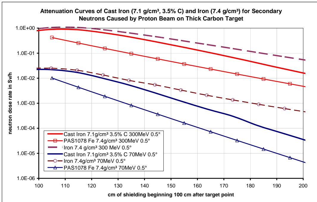
Figure 7: Compared attenuation curves for bulk shielding made of iron (7.4 g/cm 3 ) and cast iron (7.1 g/cm 3 , 3.5% C) for secondary neutrons from a thick carbon target hit by a proton beam
