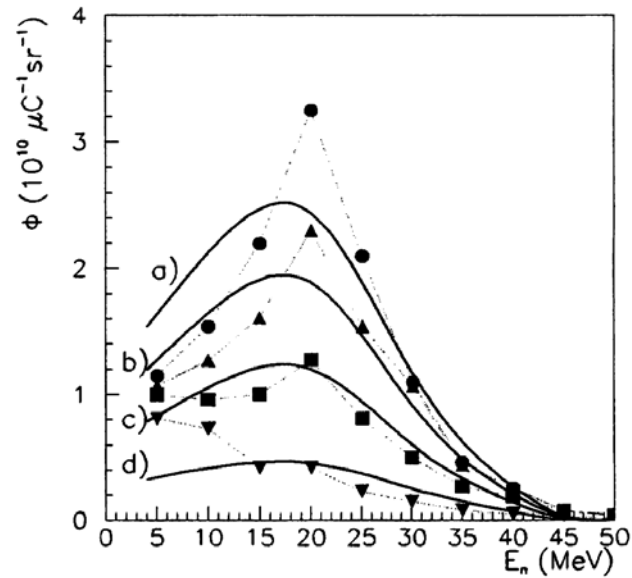
Figure 6: (a) Experimental energetic distributions of neutrons for 50 MeV ^2\text{H} incident energy on a thick Be target from Ref. [43]: filled circles at 0^\circ , filled triangles with up-point at 5^\circ , filled squares at 10^\circ , and filled triangles with down-point at 25^\circ . These distributions are compared with theoretical ones: (a) 0, (b) 5, (c) 10 and (d) 25^\circ . The dotted lines are to guide the eye.
