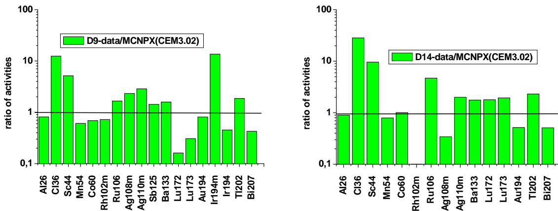
Figure 6: Same as Figure 4 but for the CEM3.02 model. Note that ^{194}\text{Ir} was not measured.
