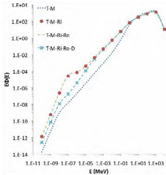
Figure 4: Neutron lethargy and time spectrum in the wave-guide
