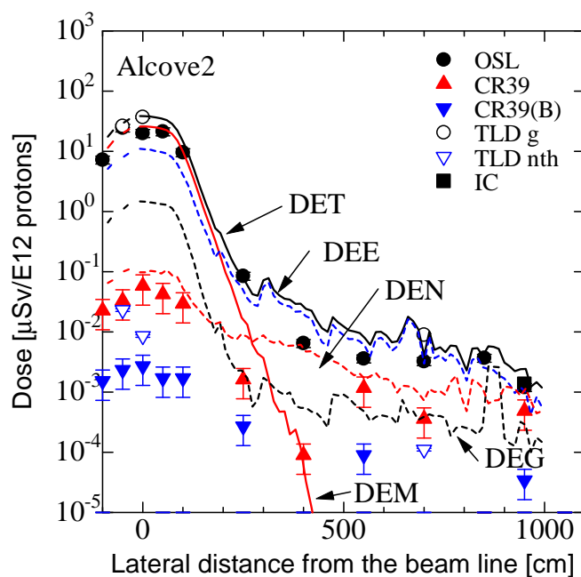
Figure 11: Dose rate distributions measured by various dosimeters along Alcove-2, which is compared with those of total, muon, photon, electron and neutron calculated by the MARS code [9]
