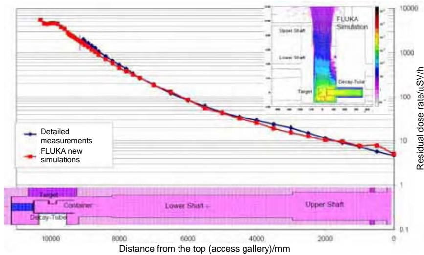
Figure 3: Comparison of residual dose rate measurements and FLUKA simulations inside the n_TOF installation pit down to the target position (without the target being installed)
