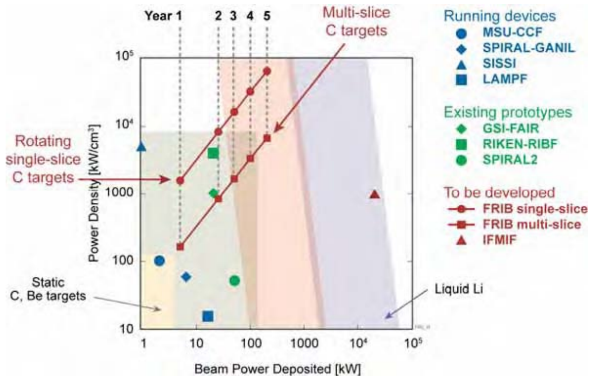
Figure 1: Choice of target technology
