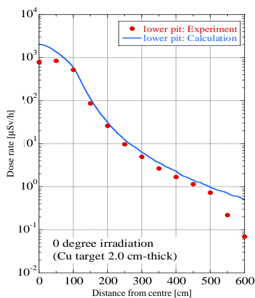
Figure 8: Comparison of dose rate distribution between measurement and calculation
