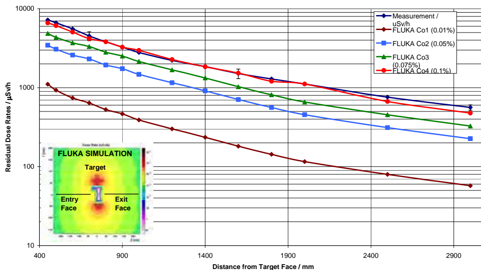
Figure 4: Comparison of residual dose rate measurements (dark blue) and FLUKA simulations for the target exit face and for different cobalt contents (brown, blue, green and red)
