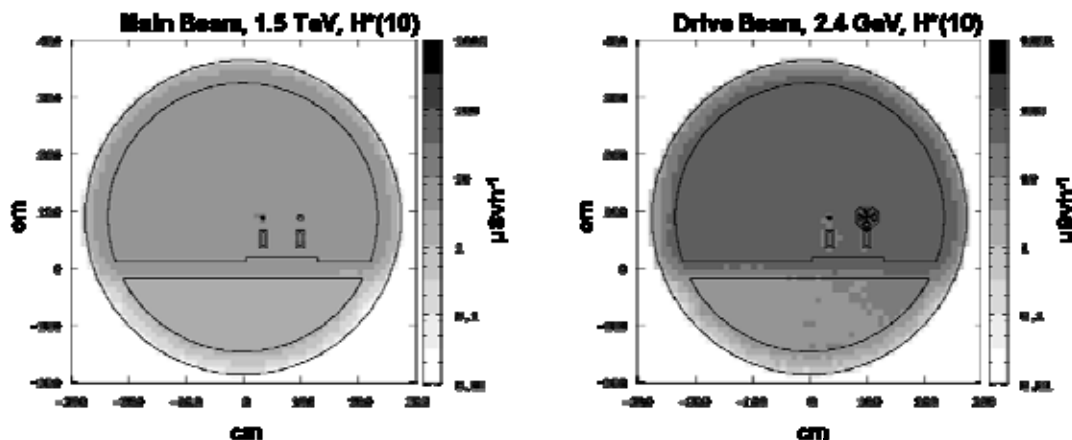
Figure 2: Residual ambient dose equivalent rates in the CLIC tunnel after 180 d running and 4 h waiting time, from losses at 1.5 TeV main beam (left) and 2.4 GeV drive beam (right), assuming maximum beam losses permitted by beam dynamics considerations
