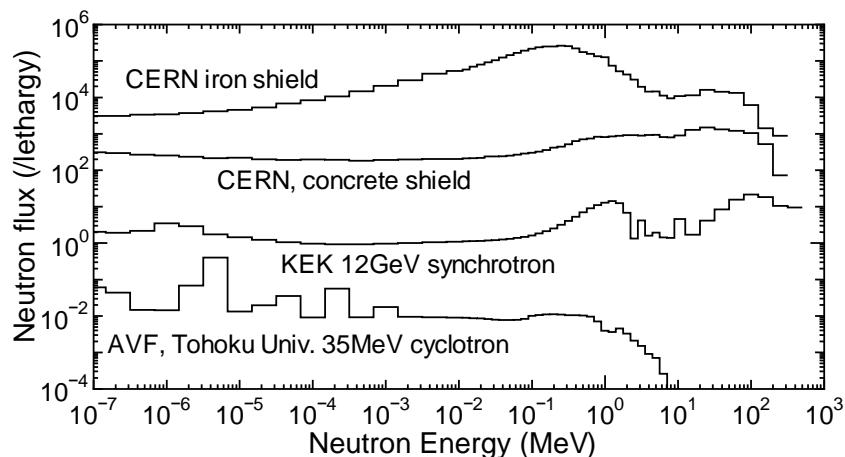
Figure 4: Examples of the neutron spectra used in the calculation of the effective doses and H^*(10) for various operational fields. The absolute values are arbitrarily adjusted for each spectrum in order to make each line distinctive.
