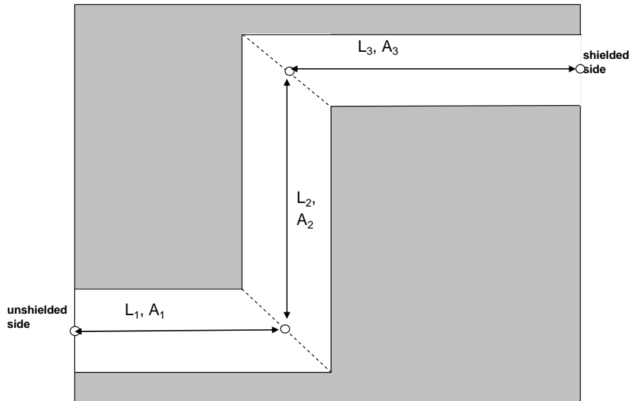
Figure 10: Sketch for the geometry model of the labyrinth case
