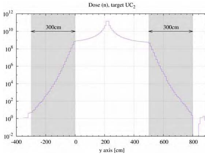
Figure 4: Ambient dose equivalent rate ( \mu\text{Sv/h} ) due to neutrons in the vertical direction (roof and floor areas are highlighted)
