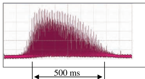
Figure 2: Pulse shape (as measured in synchrotron ring by HIMAC operators)
