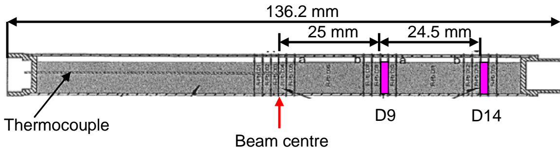
Figure 2: Rod 3 from SINQ Target 4 and its dimension. The locations of the samples D9 and D14 are indicated.
