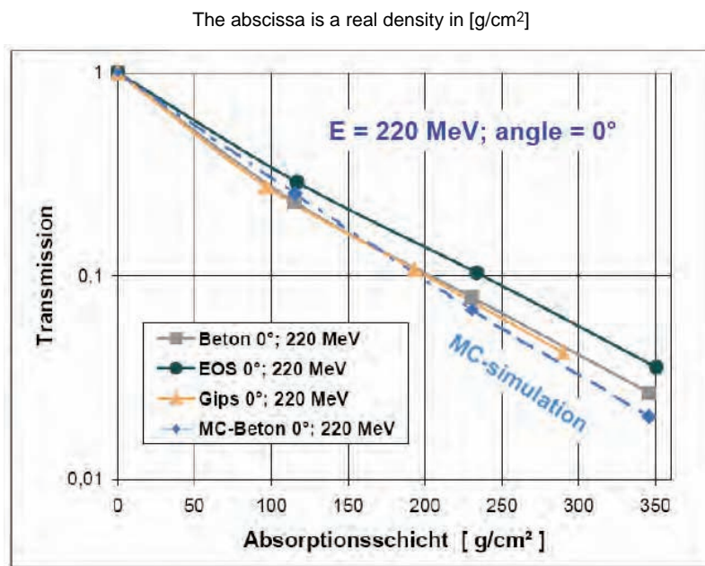
Figure 9: Transmission of neutrons generated by 220 MeV protons in a graphite target drawn for three materials: concrete (grey), electric arc slag EAS (German EOS) (green) and gypsum (beige). MC results for concrete are inserted as a light blue dashed line.
