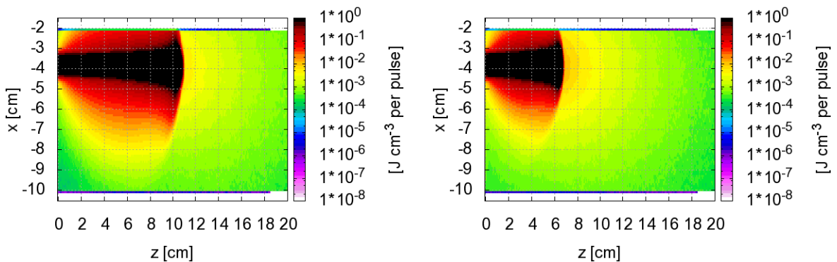
Figure 4: Profile (top view) of the average energy deposition inside the boron nitride dump (left) and the aluminium nitride dump (right). Units are J cm -3 per pulse.
