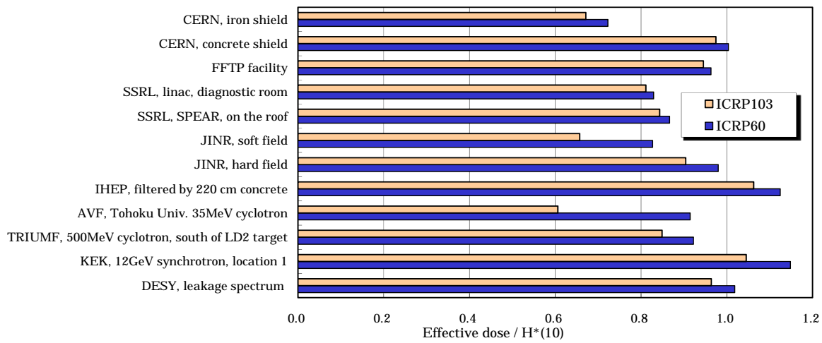
Figure 6: Ratios of the calculated effective doses based on ICRP103 and ICRP60 to the corresponding H^*(10) for various operational neutron fields
