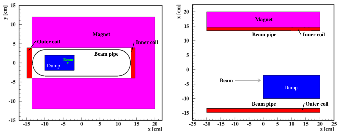
Figure 1: Left: transverse section of the dump at z = 0 (front view); right: horizontal section of the dump at y = 0 (top view)
