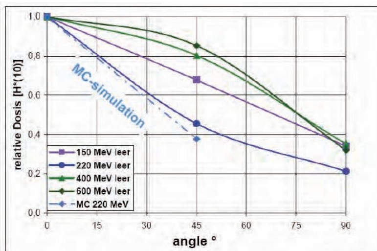
Figure 10: Measured effective dose H^*(10) depending on proton energy and angle. Each energy and angle are without any absorber in the window. The MC simulation fits well to the measured normalised data.
