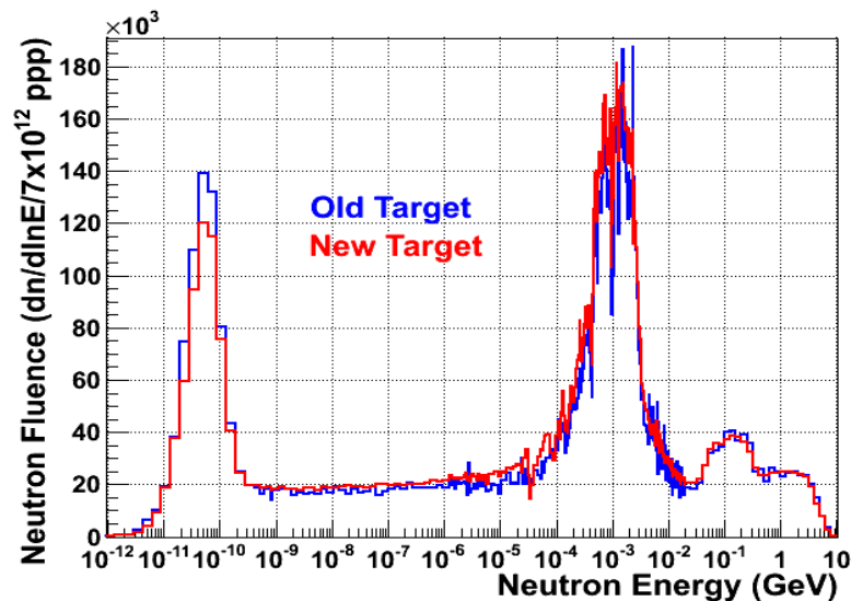
Figure 11: Simulated neutron fluence in the experimental area for the old target (in blue) and the new target (in red)
