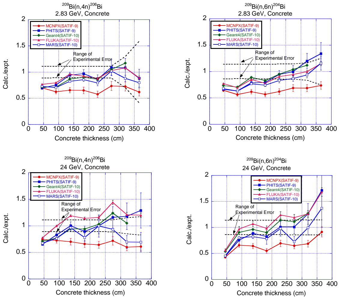
Figure 20: The C/E values of the reaction rates for the concrete shield
