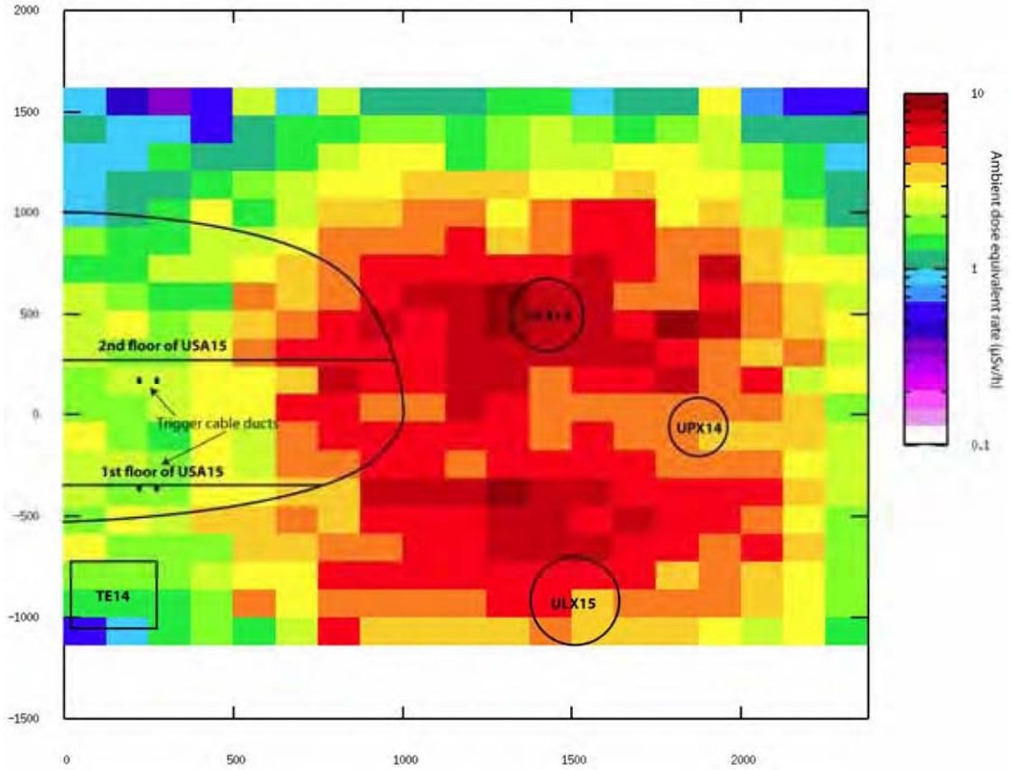
Figure 5: The dose rate distribution in the ULX15 passageway
