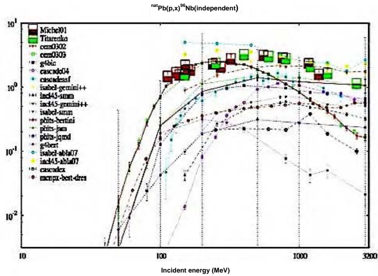
Figure 8: Excitation function of the ^{96}\text{Nb} isotope obtained with p+Pb reaction. Data (squares).
