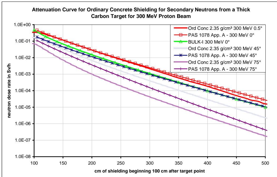
Figure 4: Attenuation curve for bulk shielding made of ordinary concrete for secondary neutrons from a thick carbon target hit by a 300 MeV proton beam
