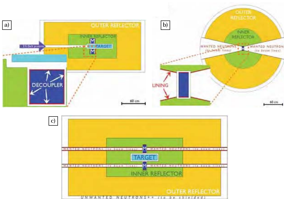
Figure 1: The full T-M-Ri-Ro-D-L geometry: a) side view; b) top view; c) beam's eye view
