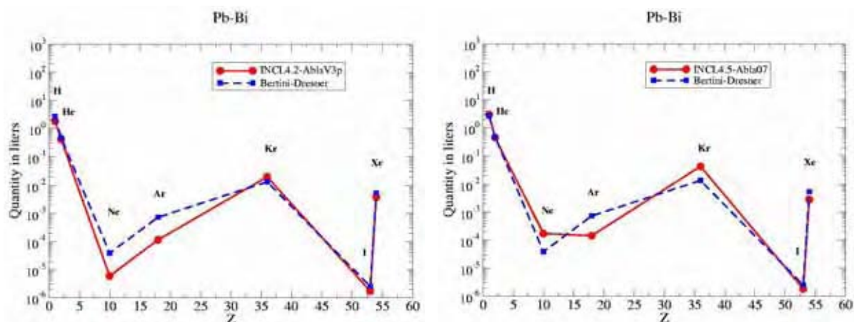
Figure 8: Quantity of volatiles (up to Xe) produced in the LBE target after 123 days of irradiation with 575 MeV protons at 0.947 mA using INCL4.2-AblaV3p (left) and INCL4.5-Abla07 (right). Bertini-Dresner, as the default option in MCNPX, is also plotted.
