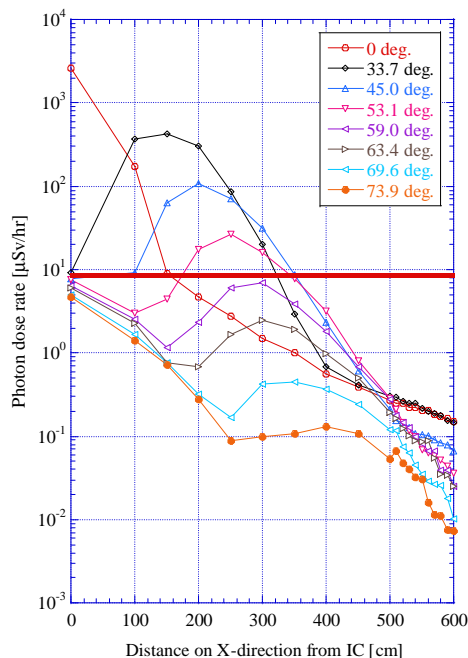
Figure 4: The dose rate distribution in the pit vs. angle of gantry head
