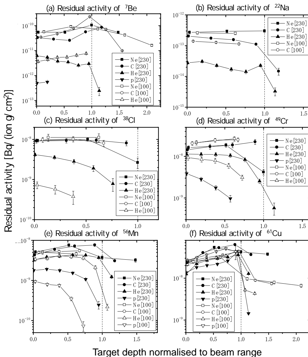
Figure 17: Spatial distribution of residual activities within Cu target depth. For example, “Ne[230]” signifies 230 MeV/nucleon Ne irradiation [82].
