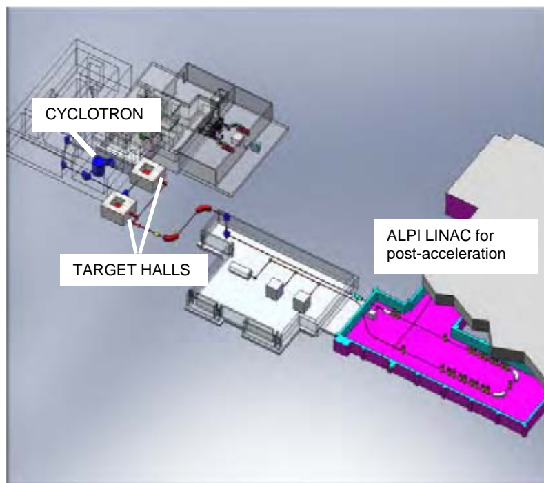
Figure 1: SPES layout. The ALPI linac already exists, while the cyclotron vault and the target halls have yet to be built.
