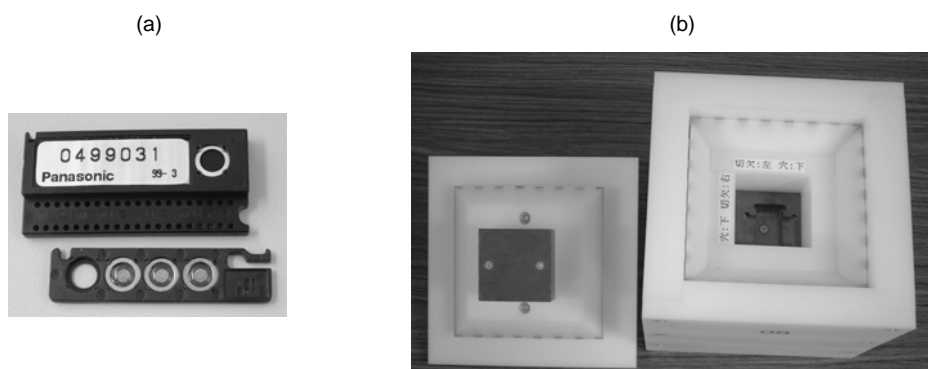
Figure 3: Photo on the left (a) shows the Panasonic UD804PQ TLD. Photo on the right (b) shows the moderator which provides the Sv response to the UD813PQ4 thermal-neutron sensitive TLD.
