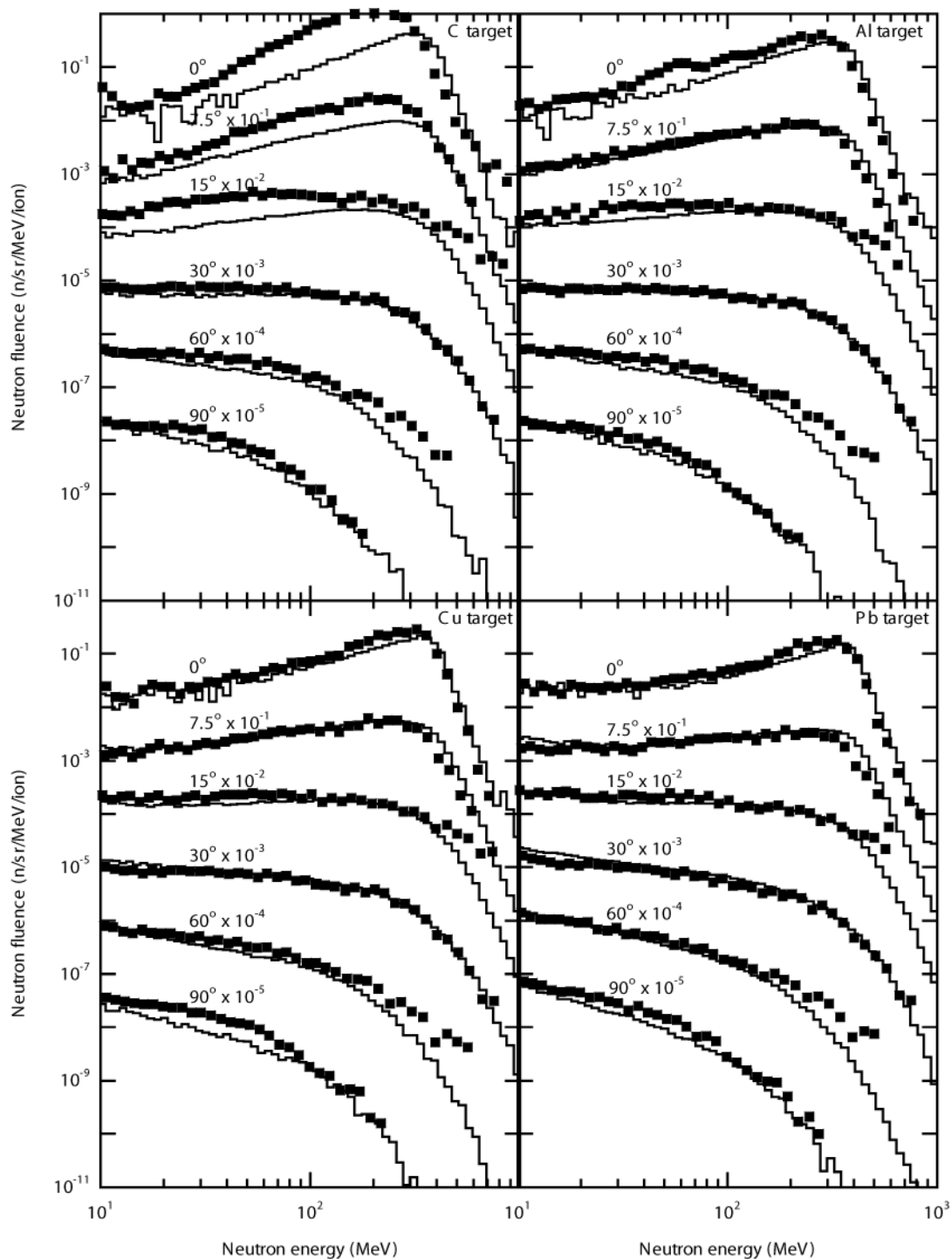
Figure 11: Neutron energy spectra for 400 MeV/nucleon Xe ion bombardment on thick C, Al, Cu and Pb targets. Marks indicate the experimental data and solid lines indicate the PHITS calculation [68].
