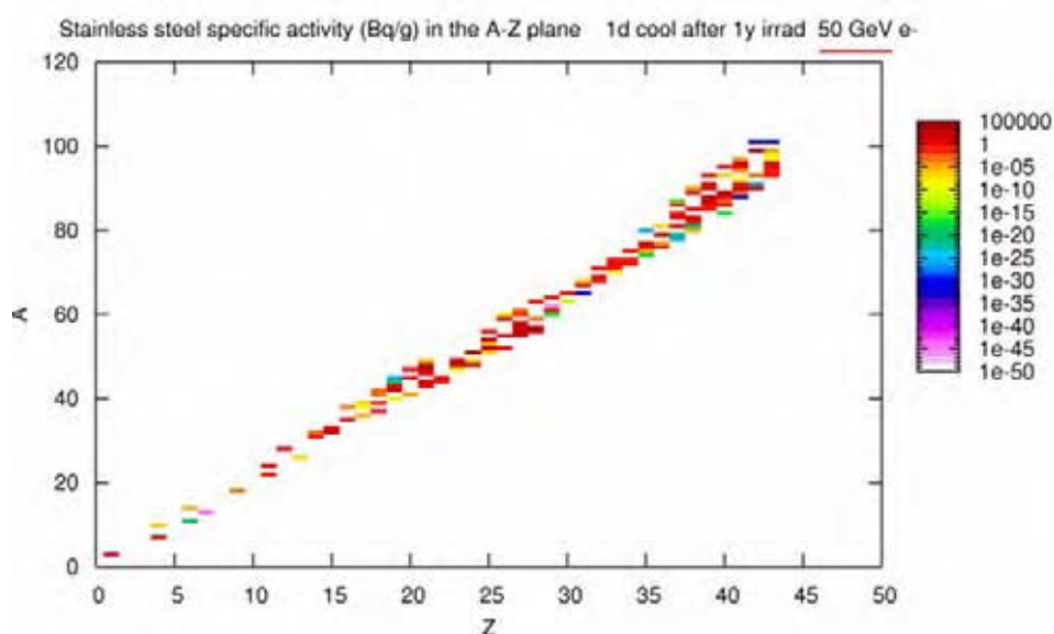
Figure 6: Distribution of the specific activity in the A-Z plane for the AISI-316L sample, after an irradiation of one year with the 50 GeV electron beam and a cooling time of 24 hours
