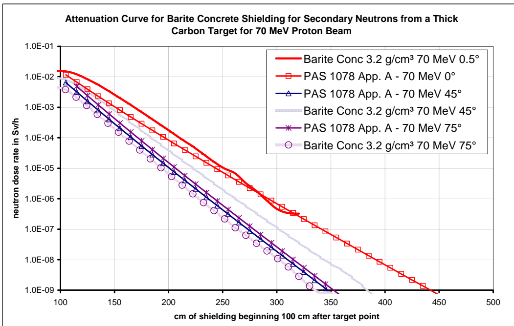
Figure 5: Attenuation curve for bulk shielding made of barite concrete for secondary neutrons from a thick carbon target hit by a 70 MeV proton beam
