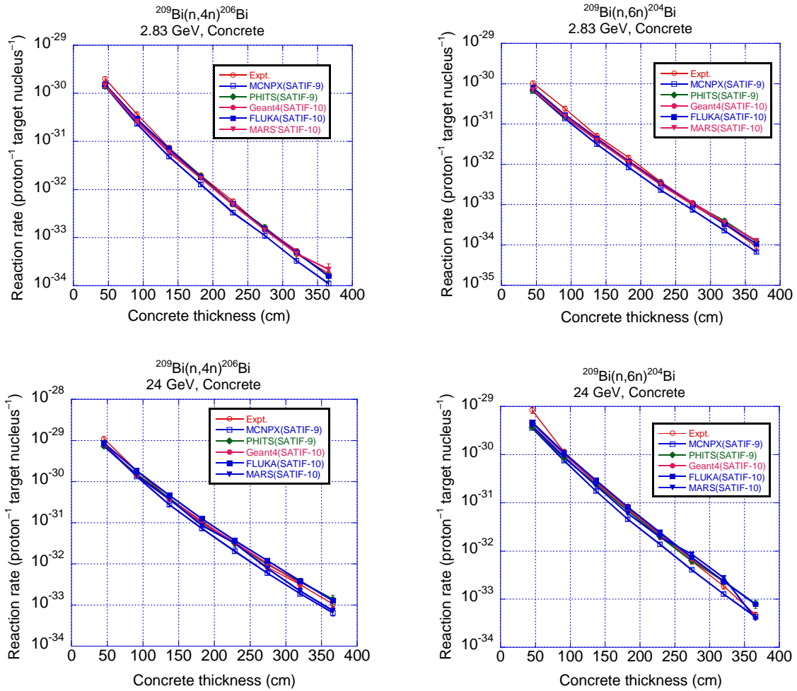
Figure 18: Comparison of calculated and measured reaction rates for the concrete shield
