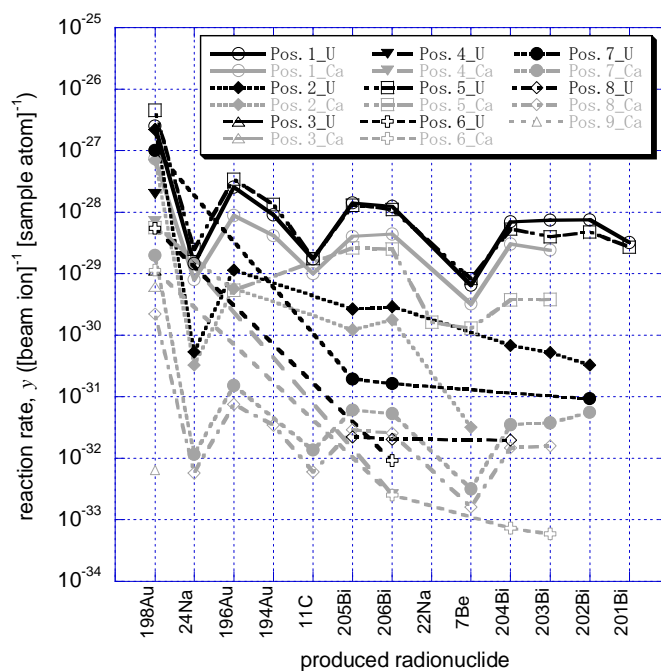
Figure 4: Measured activation reaction rate, \gamma , for U and Ca beams at various Positions 1-9. The abscissa is the produced radionuclide in order of threshold energies of the production reactions.
