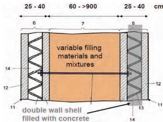
Figure 1: Principle of sandwich constructions with inner and outer double wall shells filled with concrete and in-between compacted filler materials of different kinds
