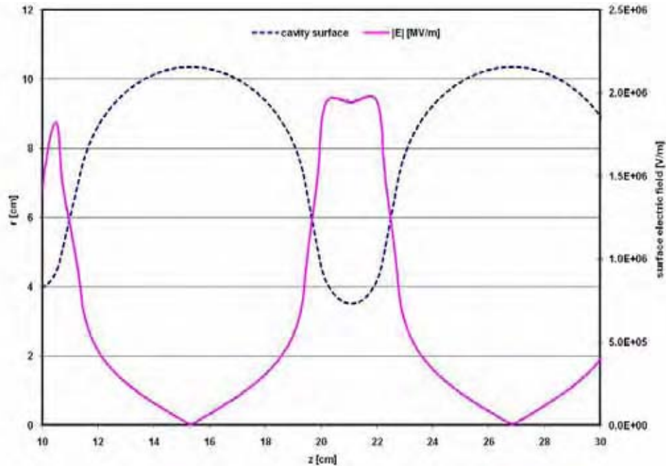
Figure 2: A zoomed view of the previous figure, showing detail around an iris in a nine-cell RF cavity
