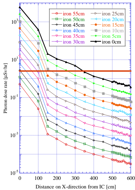
Figure 6: The calculated results of dose rate distribution in the pit for several iron thickness
