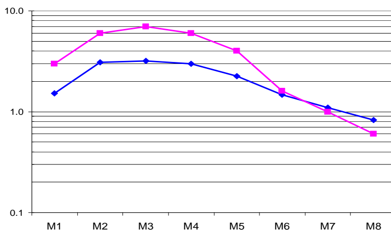
Figure 8: Dose rates in Sv/h at 100 cm distance along Target 4 (see Figure 7). The measured values are indicated by the squares, the calculated dose rates by the blue dots.
