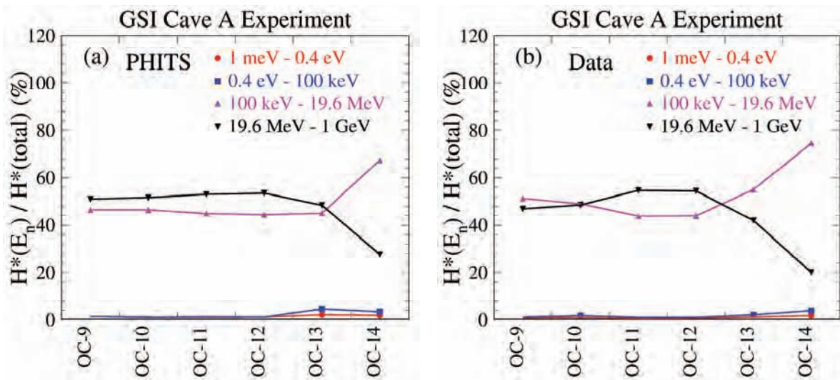
Figure 13: Relative contribution of different energy ranges to the total ambient dose equivalent: (a) this analysis; (b) Bonner sphere measurements [11]
