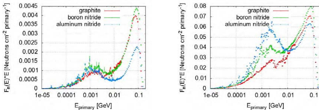
Figure 5: Neutron fluence. Left: from dump to downstream vacuum. Right: from dump to the dump shield region.
