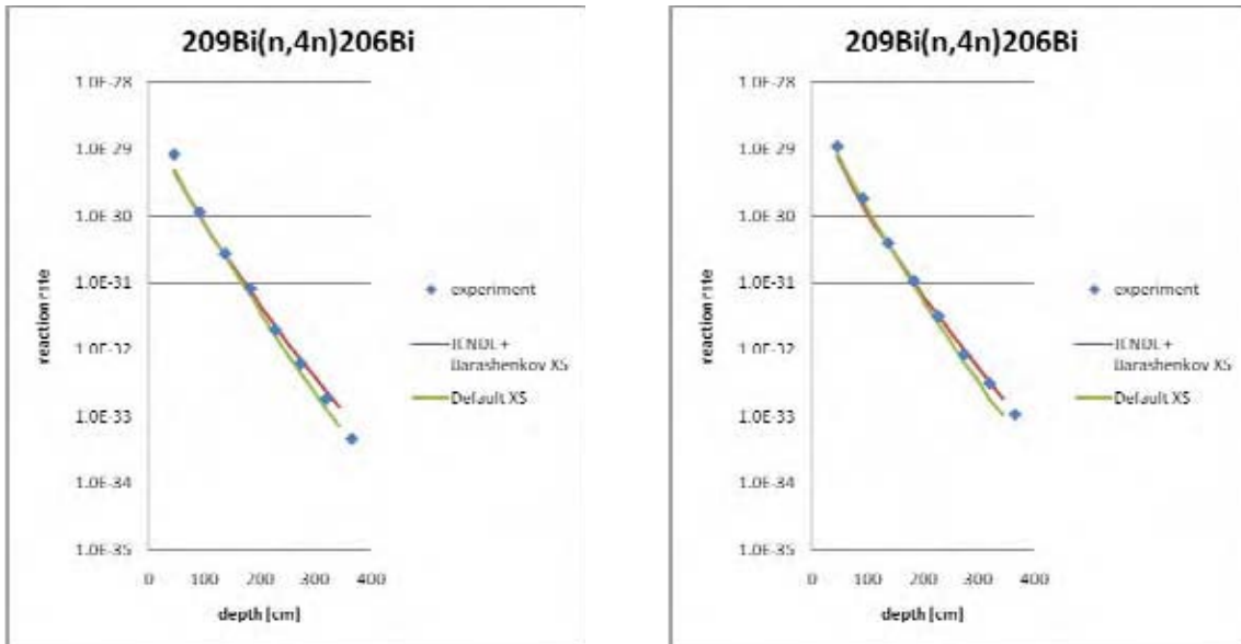
Figure 2: Comparison of calculated and measured reaction rates for the concrete shield
