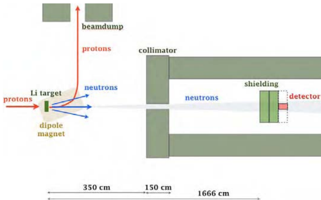
Figure 1: Geometry of the experiment
