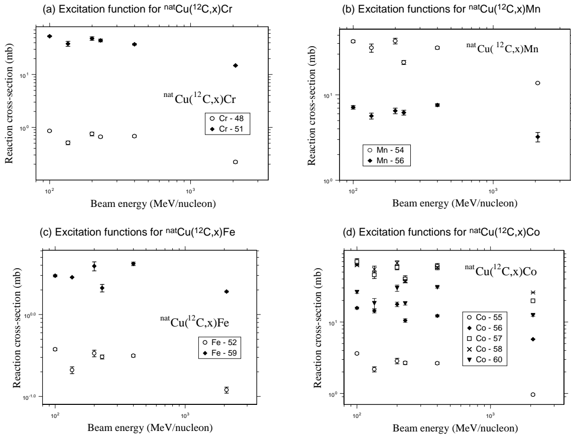
Figure 14: Excitation functions for various isotopes produced by ^{12}\text{C} interactions in Cu [2]
