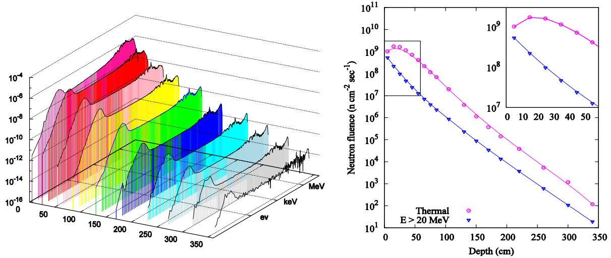
Figure 2: Left: energetic spectrum of neutrons as function of the depth in concrete (n/cm 2 /proton on target). Right: thermal (E < 1 eV) and high-energy neutrons (E > 20 MeV) as function of depth in concrete.
