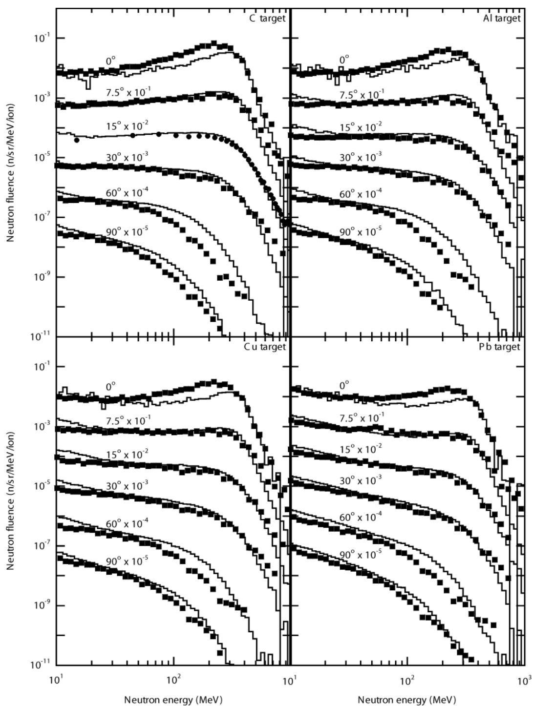
Figure 9: Neutron energy spectra for 400 MeV/nucleon C ion bombardment on thick C, Al, Cu and Pb targets. Marks indicate the experimental data and solid lines indicate the PHITS calculation [68].
