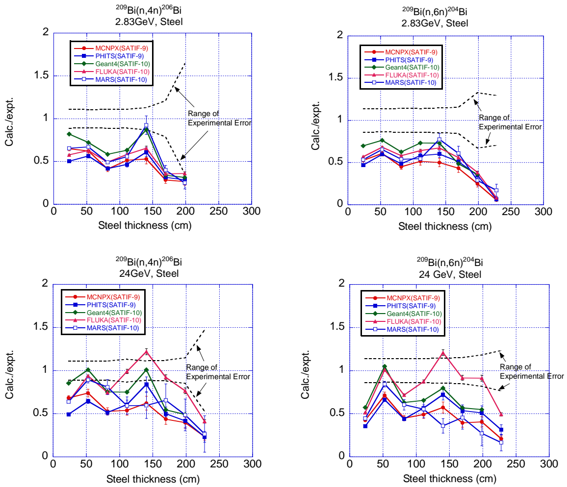
Figure 19: The C/E values of the reaction rates for the steel shield
