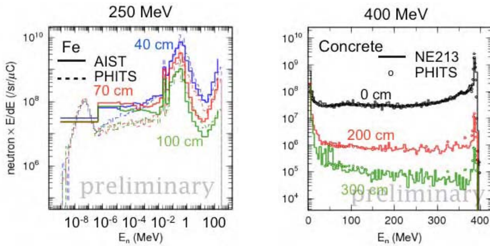
Figure 3: Preliminary results of the measured and calculated neutron energy spectra
