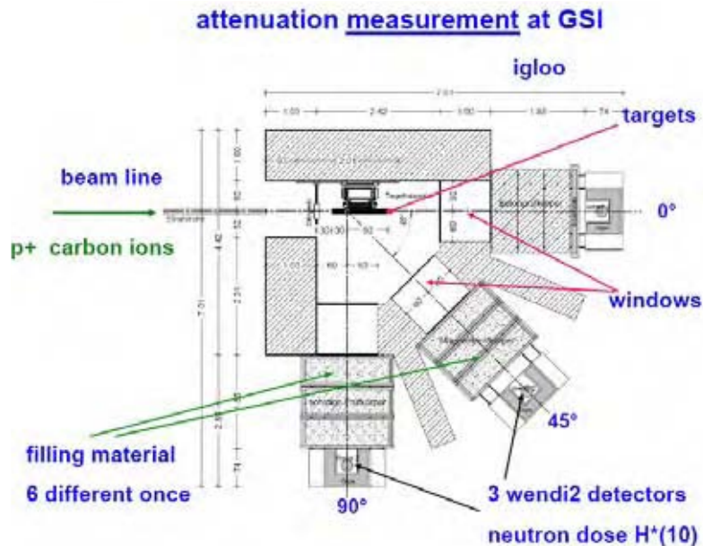
Figure 8: Real situation of the set-up in one cave at GSI (Darmstadt, Germany). The total mass which must be transported and inserted into the cave was about 240 t (igloo and testing materials).
