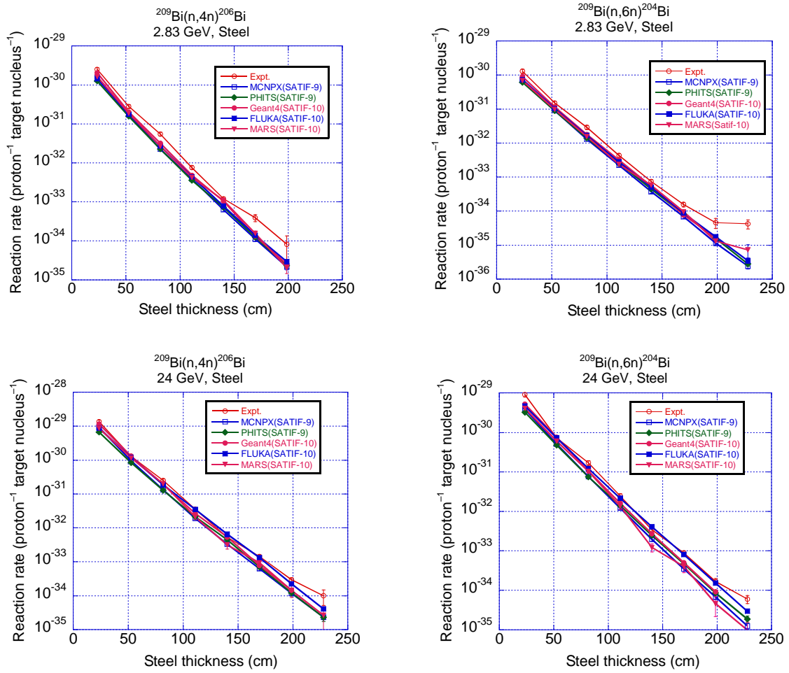
Figure 17: Comparison of calculated and measured reaction rates for the steel shield
