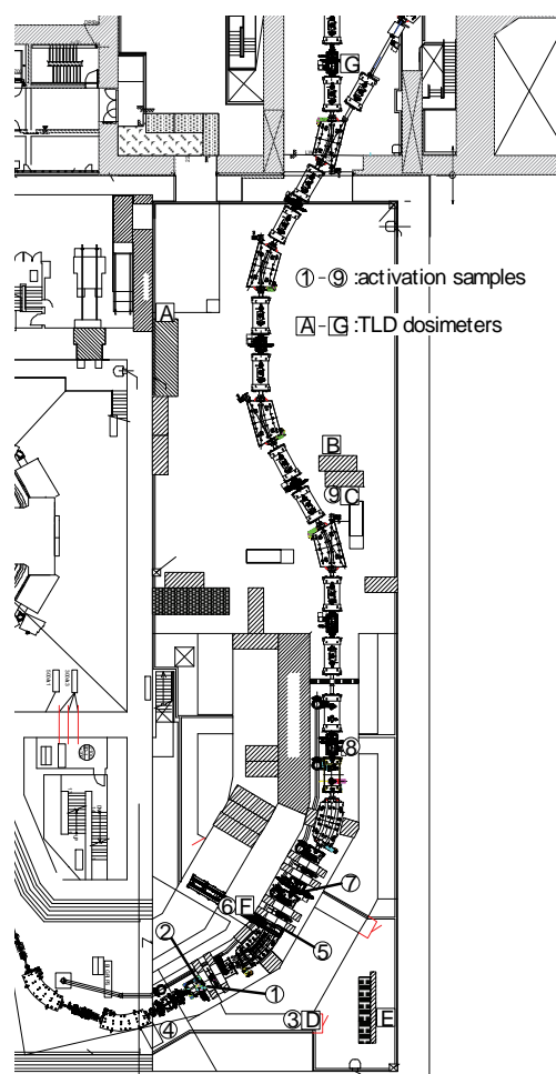
Figure 1: Positions where the activation samples and TLD were placed
