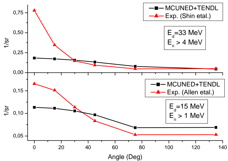
Figure 10: Normalised neutron angular distribution (experiments from Refs. [21,23])
