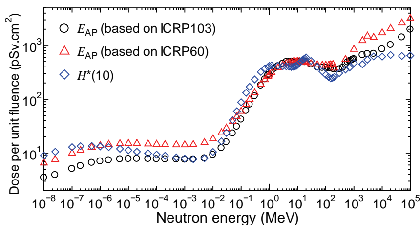
Figure 5: Conversion coefficients from fluence to the effective doses for the AP irradiation geometry, E_{AP} , and the ambient dose equivalent at 10 mm, H^*(10) , used in the calculation of neutron doses for various operational fields
