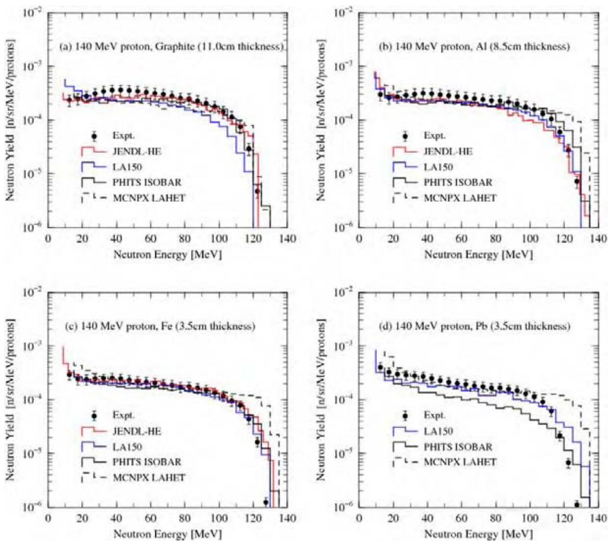
Figure 3: Neutron energy spectra for 140 MeV proton incidence on thick graphite, aluminium, iron and lead targets. The experimental results are compared with the calculated results as given in the text [21].
