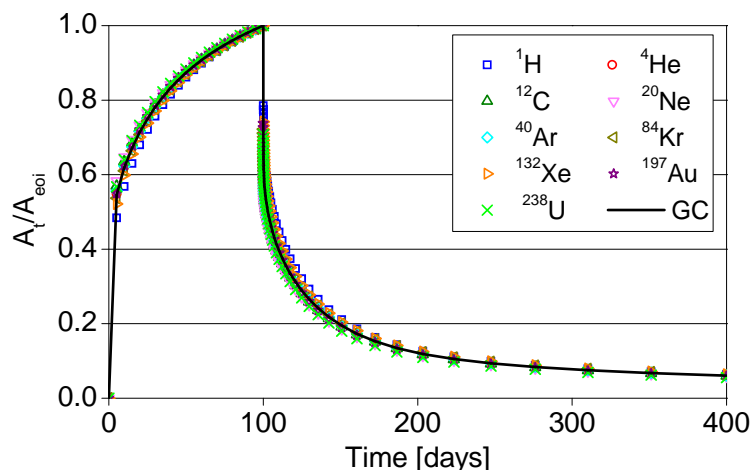
Figure 4: Time evolution of the relative activity induced in the beam pipe by different projectiles at 500 MeV/u calculated by FLUKA
