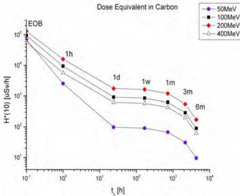
Figure 6: Ambient dose equivalent rate, as a function of cooling time, from a carbon target impacted by a proton beam of the indicated energies
