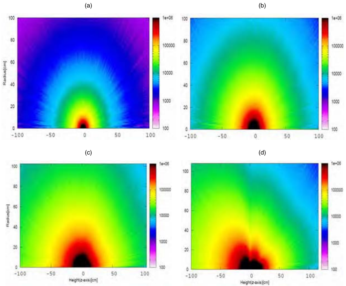
Figure 3: Ambient dose equivalent rates for a copper target [ \mu\text{Sv/h} ], impacted by a proton beam of: (a) 50 MeV, (b) 100 MeV, (c) 200 MeV and (d) 400 MeV after a cooling time of one day
