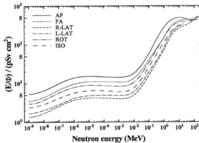
Figure 6: Neutron fluence-to-effective dose conversion coefficients according to ICRP 26 [5] and ICRU 57 [6] from thermal up to 200 MeV; conversion factors above 200 MeV; see Thomas, et al. [7]
