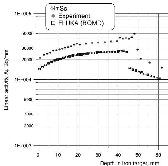
Figure 6: Experimental and simulated ^{44m}\text{Sc} activity distribution inside the target
