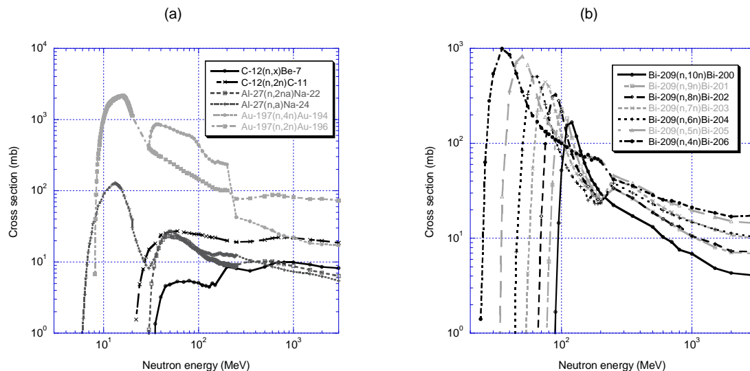
Figure 5: Activation reaction cross-sections of carbon, aluminium, gold (a) and bismuth (b)
