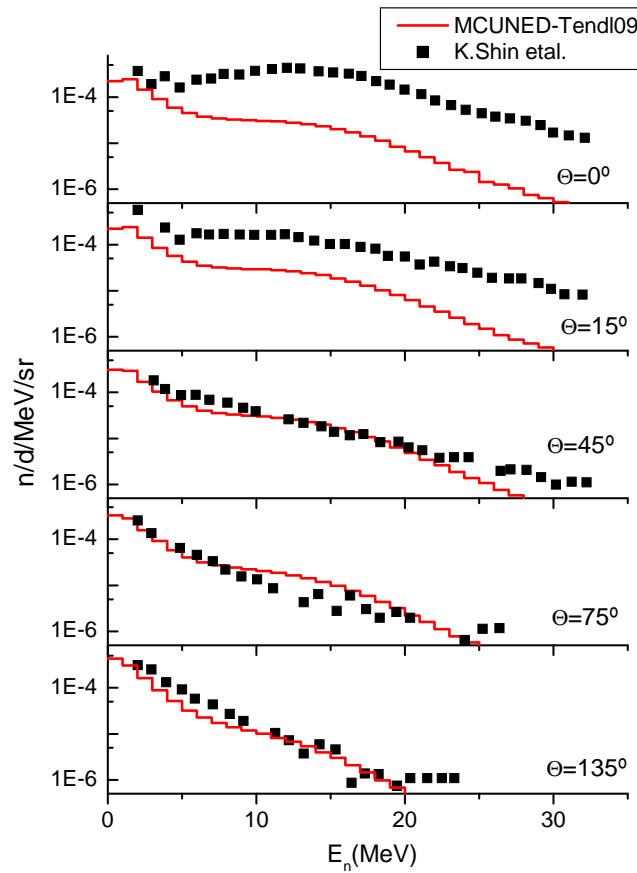
Figure 9: Neutron spectra produced by 33 MeV deuterons (experiments from Ref. [21])
