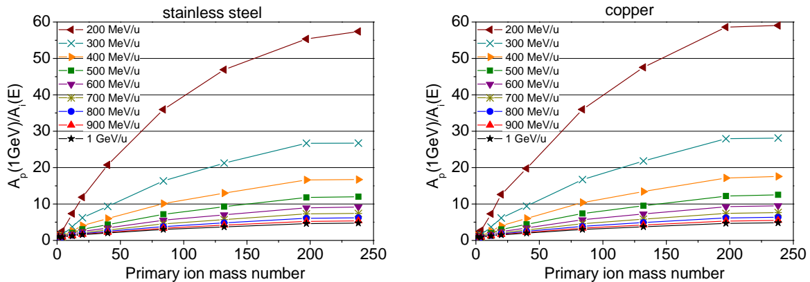
Figure 10: Scaling factor for the hands-on maintenance criteria as a function of ion mass for the bulky target
