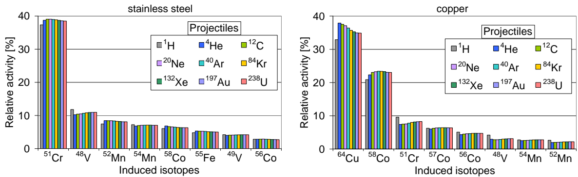
Figure 8: Isotope inventory and their relative activities 1 day after the end of irradiation induced by 1 GeV/u projectiles from proton up to uranium in stainless steel (left) and copper (right) bulky target calculated by FLUKA
