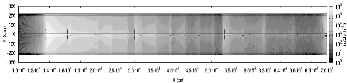
Figure 5: Residual \text{H}^*(10) in the collimation section for {}^{18}\text{Ne} after 1 week
