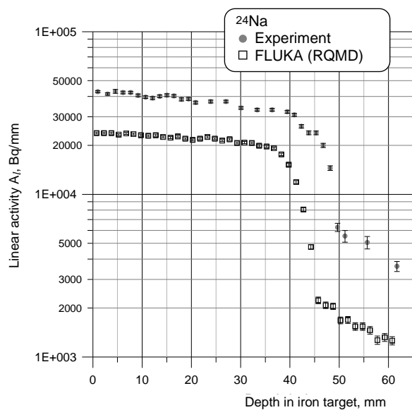
Figure 5: Experimental and simulated ^{24}\text{Na} activity distribution inside the target
