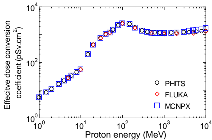
Figure 3: Irradiation-geometry dependence of the effective dose conversion coefficients for neutrons calculated by PHITS [7]
