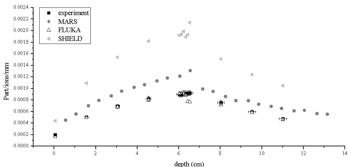
Figure 4: Depth profiles of ^{22}\text{Na} produced by 500 MeV/u argon beam in aluminium target. Comparison of experiment and simulations by FLUKA, MARS and SHIELD-A.
