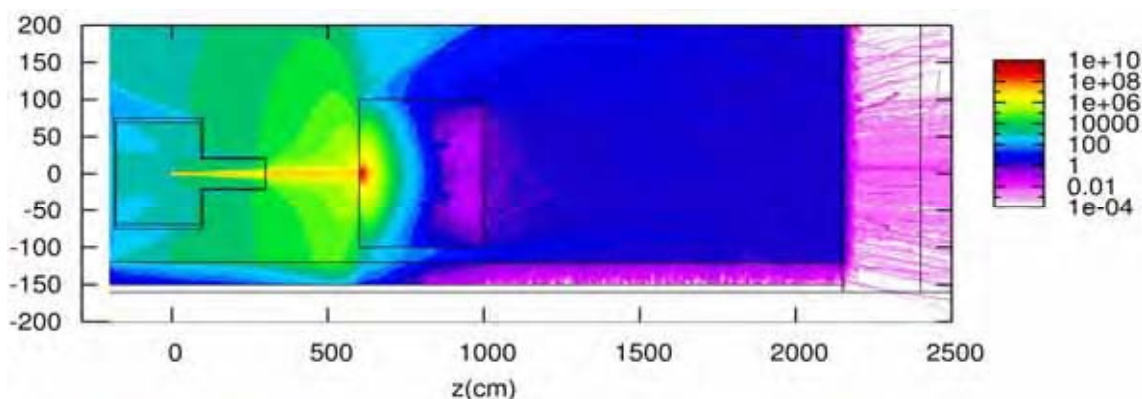
Figure 3: H^*(10) rate (in \mu\text{Sv/day} ) in the case of the 5 GeV electron beam, 10 Hz, impinging on a mono-material dump in copper
