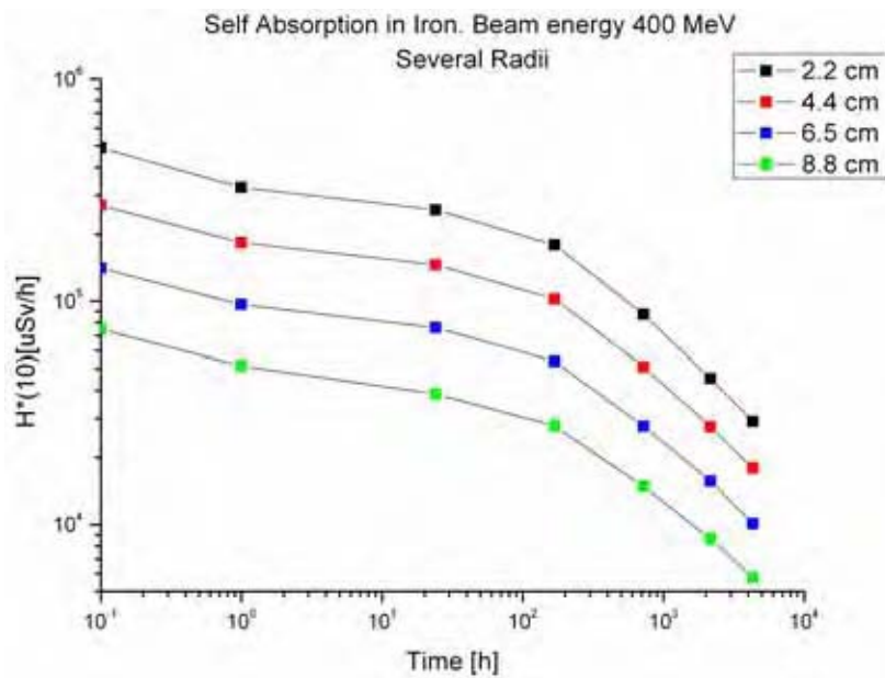
Figure 10: Ambient dose equivalent rate around an iron target, after irradiation with a 400 MeV beam, as a function of cooling time for different target radii
