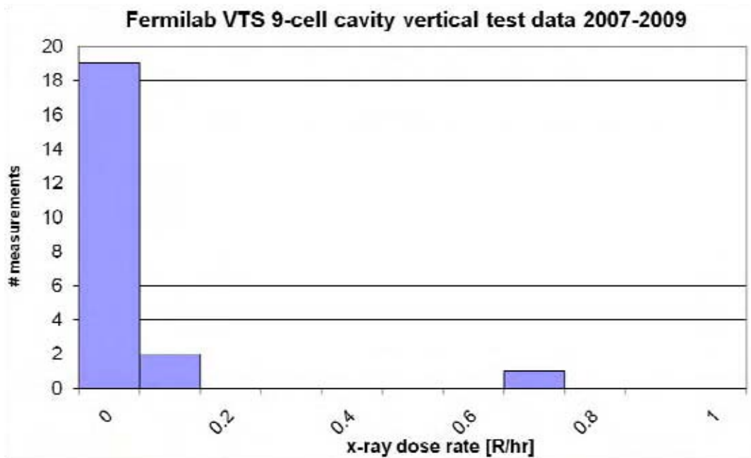
Figure 6: Dose rates measured at VTS1 for nine-cell superconducting RF cavities with various accelerating gradients
