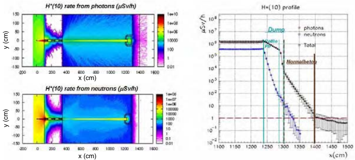
Figure 7: Ambient dose equivalent rate distributions inside the experimental neutron room, due to the photon and neutron beams from the radiator (left); H^*(10) rate profile obtained by averaging the same data in a volume 20 cm large and centred along the beamline (right)
