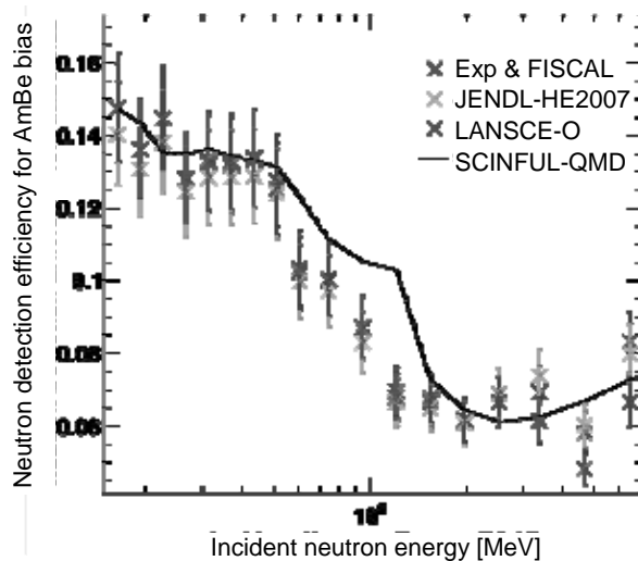
Figure 9: Neutron detection efficiency of an NE213 scintillator at LANCE
