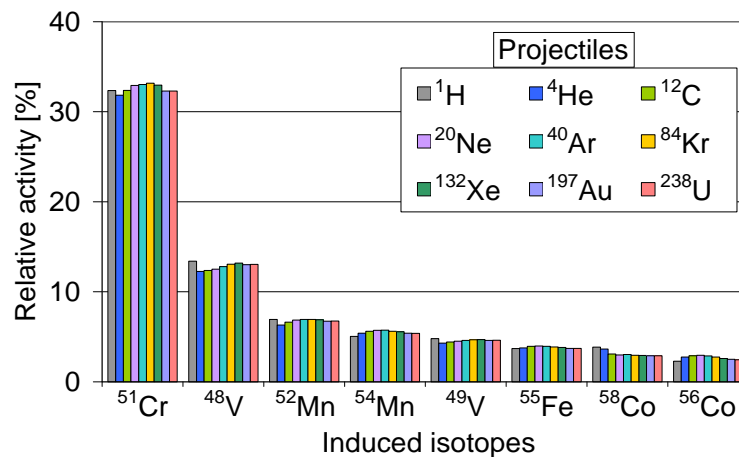
Figure 3: Relative activities of the isotopes induced by 1 GeV/u projectiles from proton up to uranium in the stainless steel beam pipe one day after the end of irradiation calculated by FLUKA
