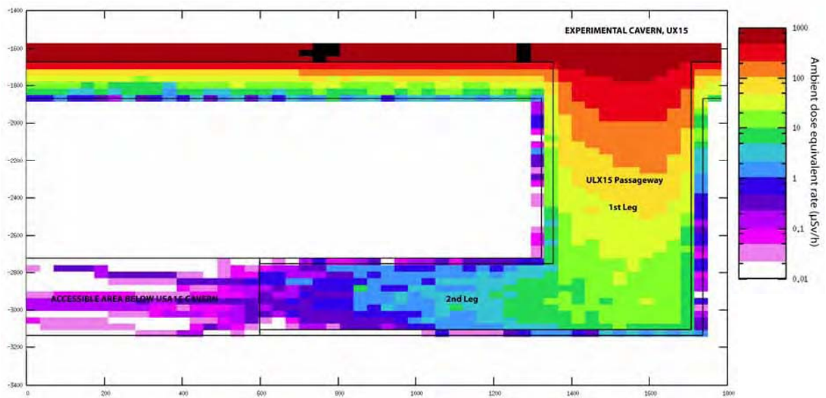
Figure 5: The dose rate distribution in the ULX15 passageway
