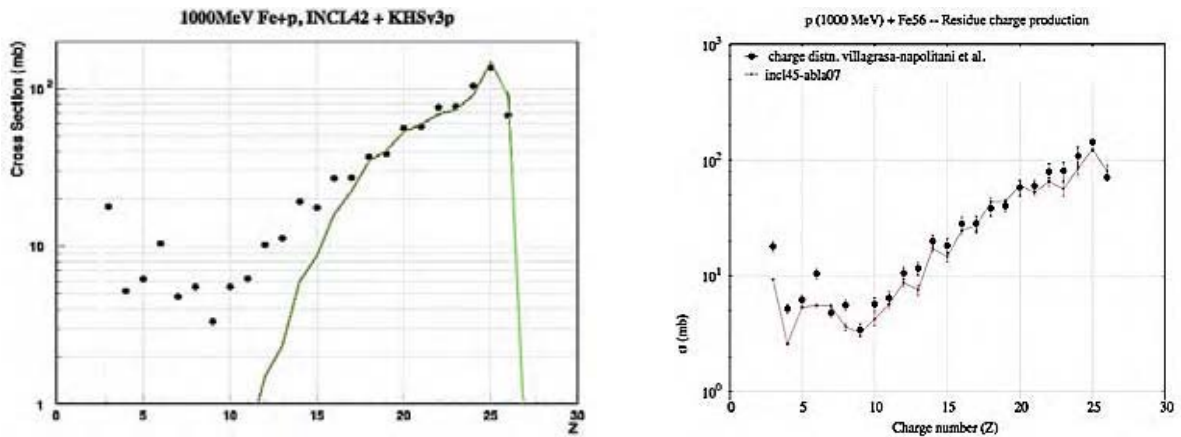
Figure 5: Charge distribution for the reaction Fe(1 GeV.u) + p
