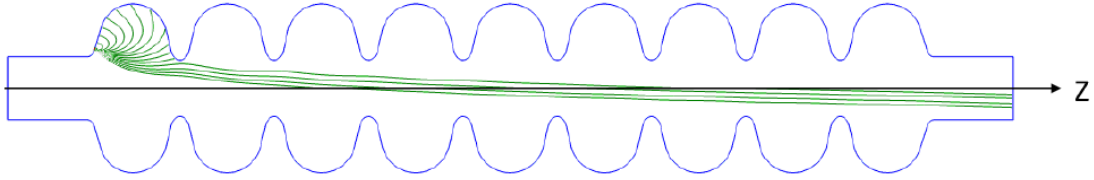
Figure 3: Simulated electron trajectories generated in a nine-cell SRF cavity with an accelerating gradient of 30 MV/m. The curves inside the cavity correspond to electron trajectories for 10° increments in the RF phase, for the half period in which the electric field has the correct sign to pull electrons from the surface.
