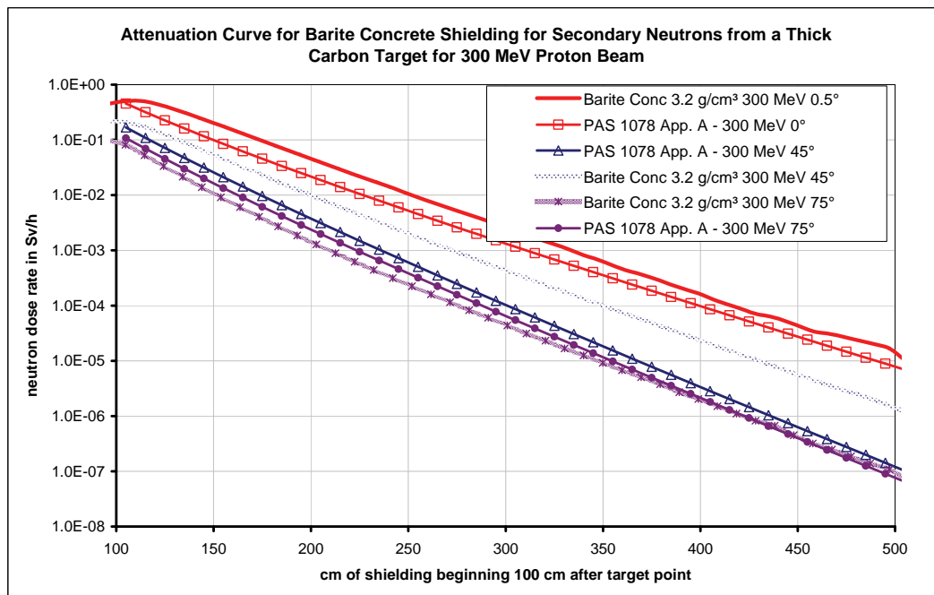
Figure 6: Attenuation curve for bulk shielding made of barite concrete for secondary neutrons from a thick carbon target hit by a 300 MeV proton beam
