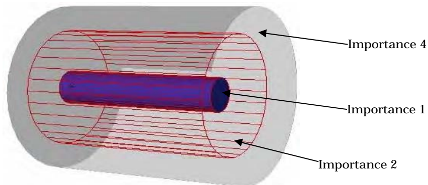
Figure 1: The importance biasing applied to the target in order to compensate for the attenuation of the neutron fluence
