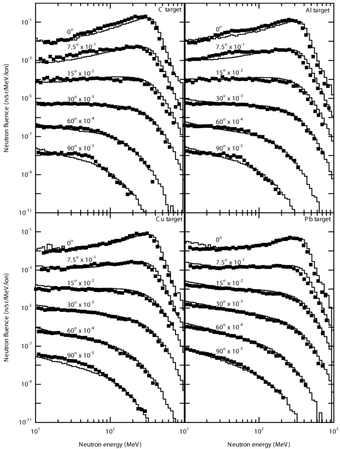
Figure 10: Neutron energy spectra for 400 MeV/nucleon Fe ion bombardment on thick C, Al, Cu and Pb targets. Marks indicate the experimental data and solid lines indicate the PHITS calculation [68].
