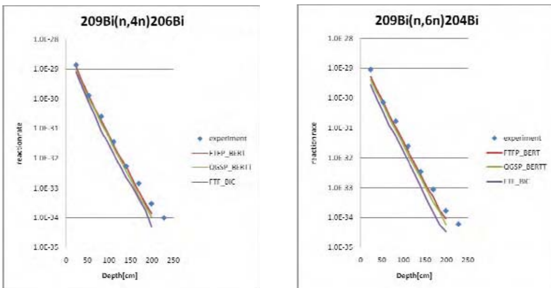
Figure 3: Comparison of calculated and measured reaction rates for the steel shield
