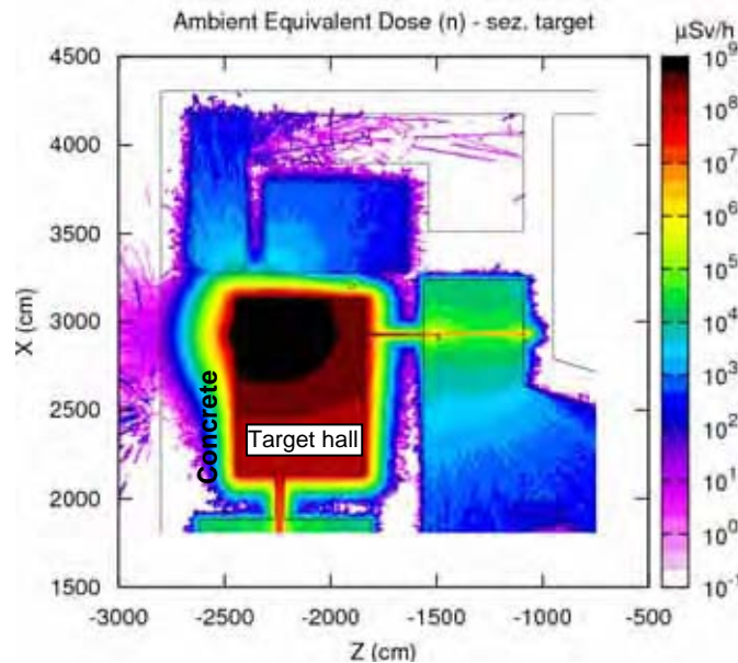
Figure 3: Ambient dose equivalent rate (μSv/h) due to neutrons in the target hall and in the adjacent rooms
