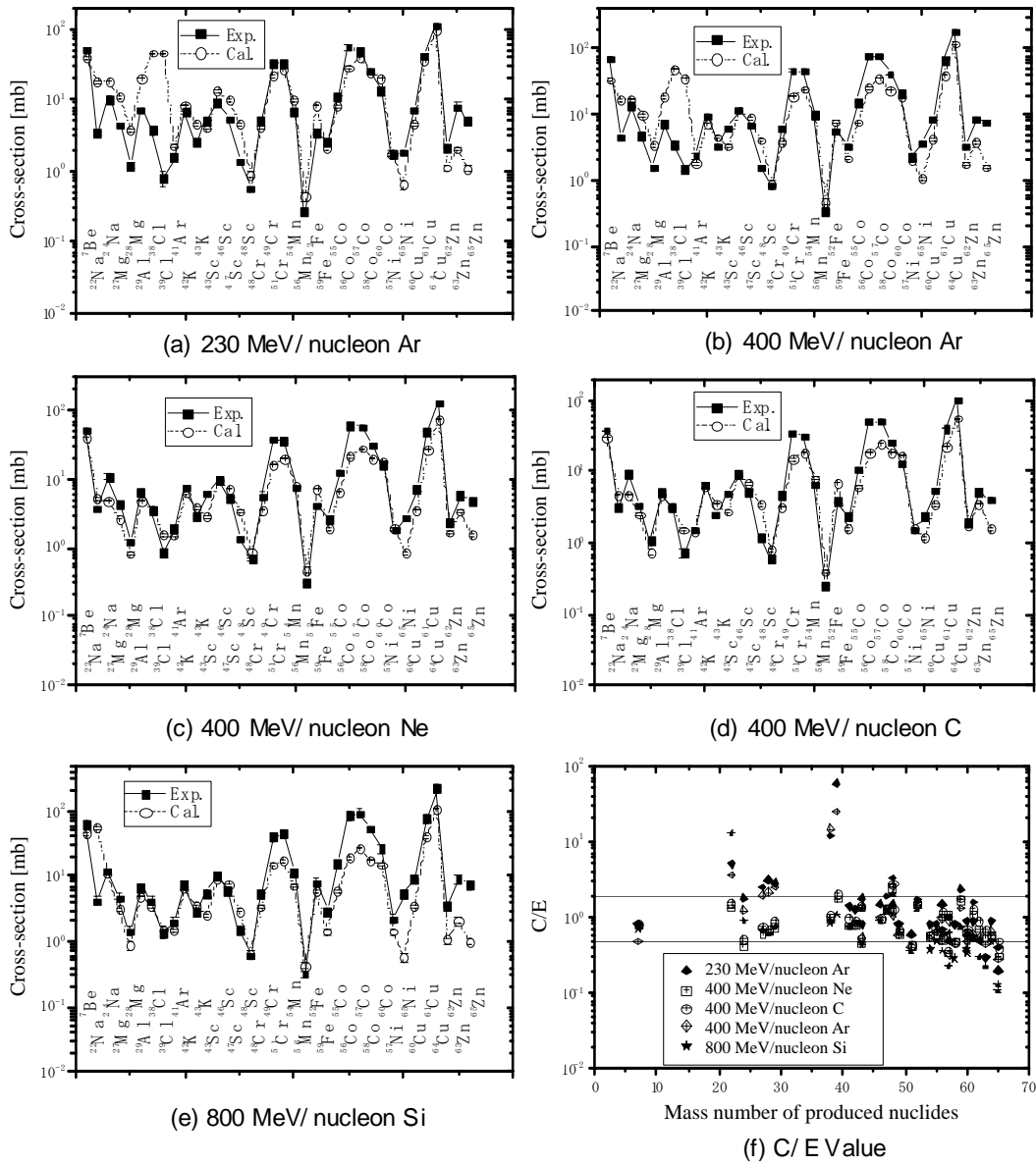
Figure 15: Comparison of measured cross-sections of radioactive nuclides produced in Cu for various projectiles with the PHITS Monte Carlo calculation [81]
