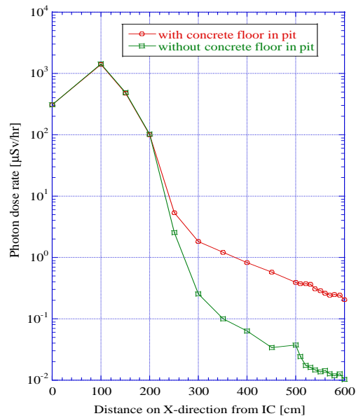
Figure 7: Calculated results of dose rate distribution with and without concrete floor in the pit
