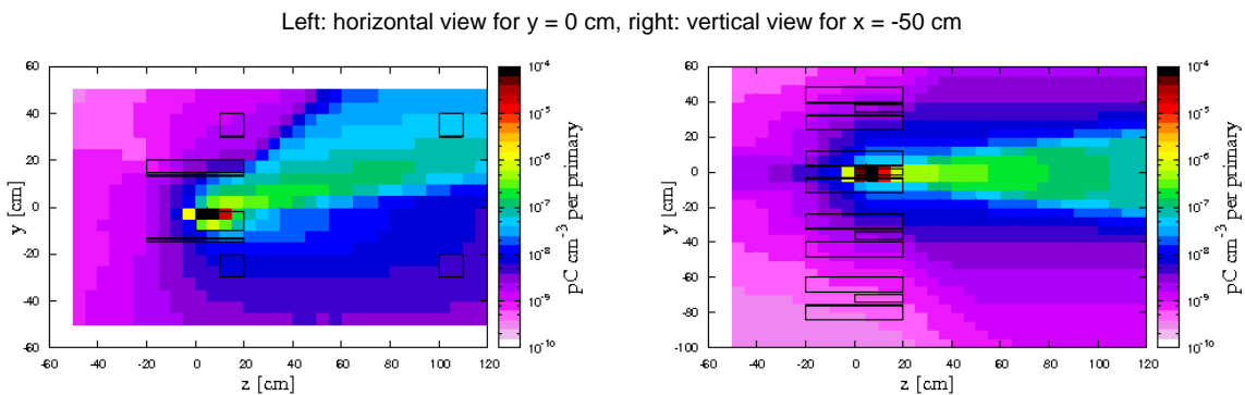
Figure 10: Plot of the charge deposited into a hypothetical BLM centred on the corresponding co-ordinates for a H 0 beam in the third PSB ring
