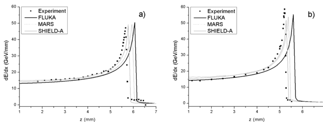
Figure 2: Penetration depth of U ions with energy E = 500 MeV/u a) in stainless steel, b) in copper
