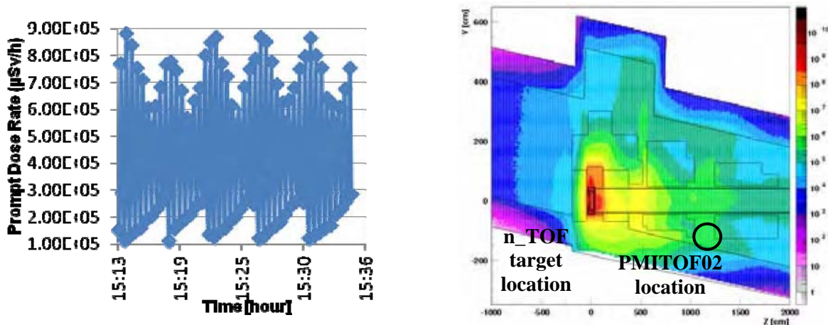
Figure 10: Prompt dose rate (in \mu\text{Sv/h} ) measured by PMITOF02 during few pulses on 11/11/2008 (left); FLUKA simulation of the prompt dose (in \mu\text{Sv/h} ) in the target area (right)
