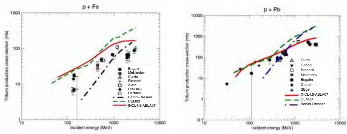
Figure 4: Helium excitation functions: Fe(p,x \alpha )
