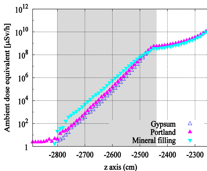
Figure 5: Comparison of the attenuation efficiency of concrete and sandwich-like structure with gypsum or blast furnace waste as filling. The target irradiated is made of \text{SiC} .
