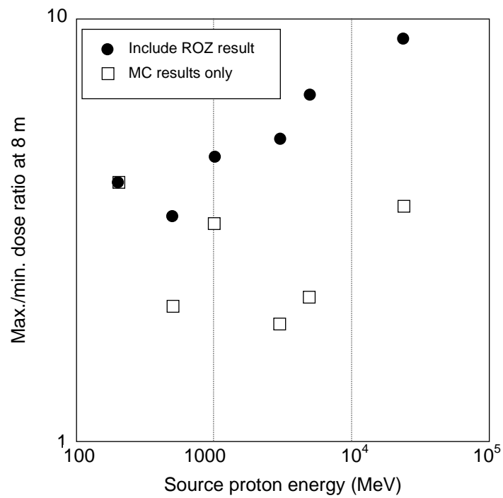
Figure 16: Neutron dose difference at 8 m inside concrete from secondary neutrons emitted to 90° ROZ 6.6, FLUKA, MARS, GEANT4 and HETC-3STEP
