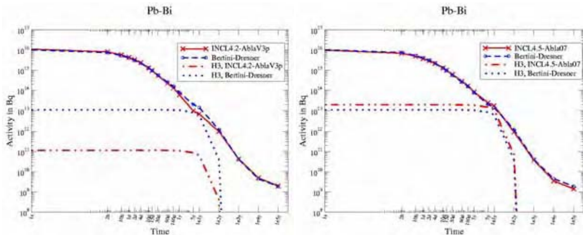
Figure 7: Total activity of the LBE target as a function of cooling time after 123 days of irradiation with 575 MeV protons at 0.947 mA using INCL4.2-AbIaV3p (left) and INCL4.5-AbIa07 (right). Bertini-Dresner, as default option in MCNPX, is also used as the contributions from tritium.
