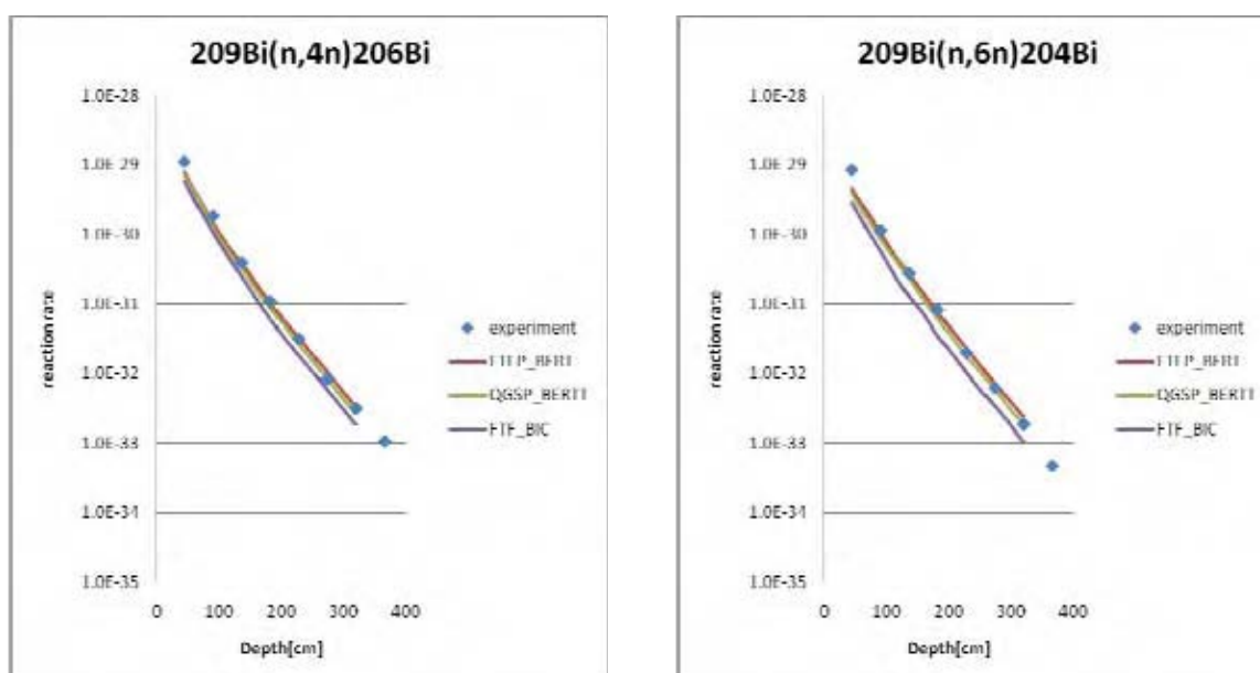
Figure 4: Comparison of calculated and measured reaction rates for the concrete shield
