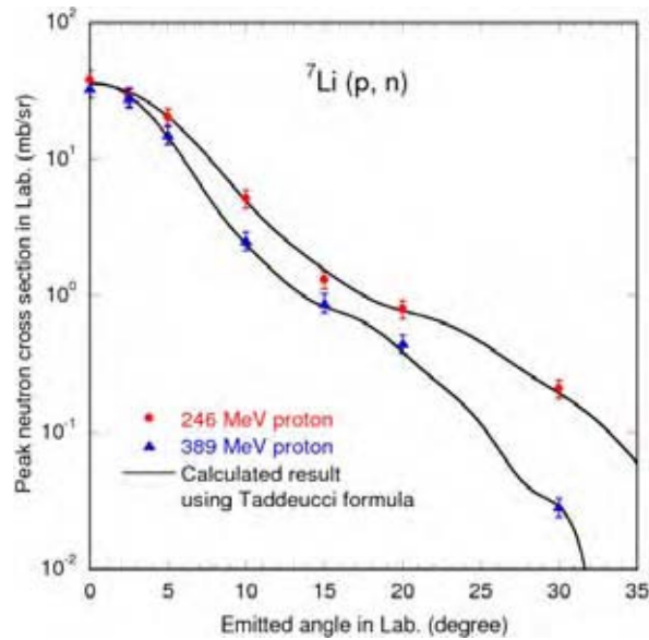
Figure 7: Angular distribution of the peak cross-sections
