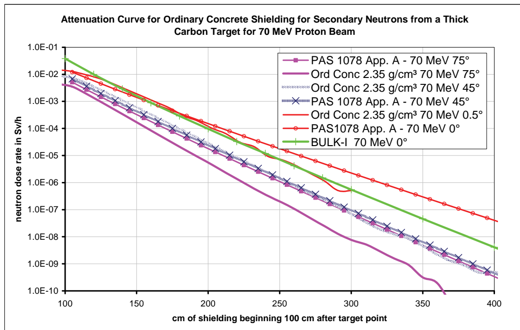
Figure 3: Attenuation curve for bulk shielding made of ordinary concrete for secondary neutrons from a thick carbon target hit by a 70 MeV proton beam
