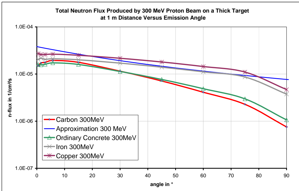
Figure 2: Total neutron flux produced by a 300 MeV proton beam directed onto a thick target at 1 m distance versus emission angle – comparison for various target materials with the approximation
