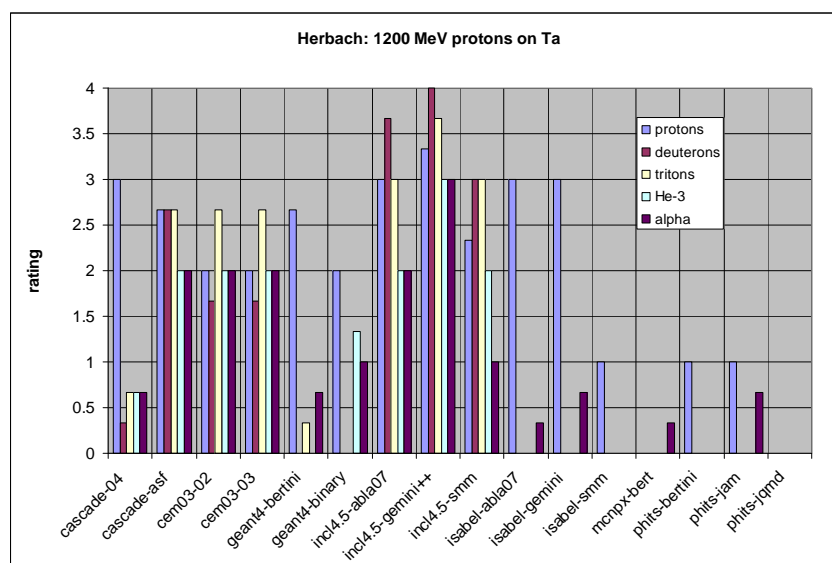
Figure 4: Rating for each model for the different types of LCP [p(1.2 GeV) + Ta]. Models having no mechanism to produce high-energy composite particles have not been rated for these types of LCP.
