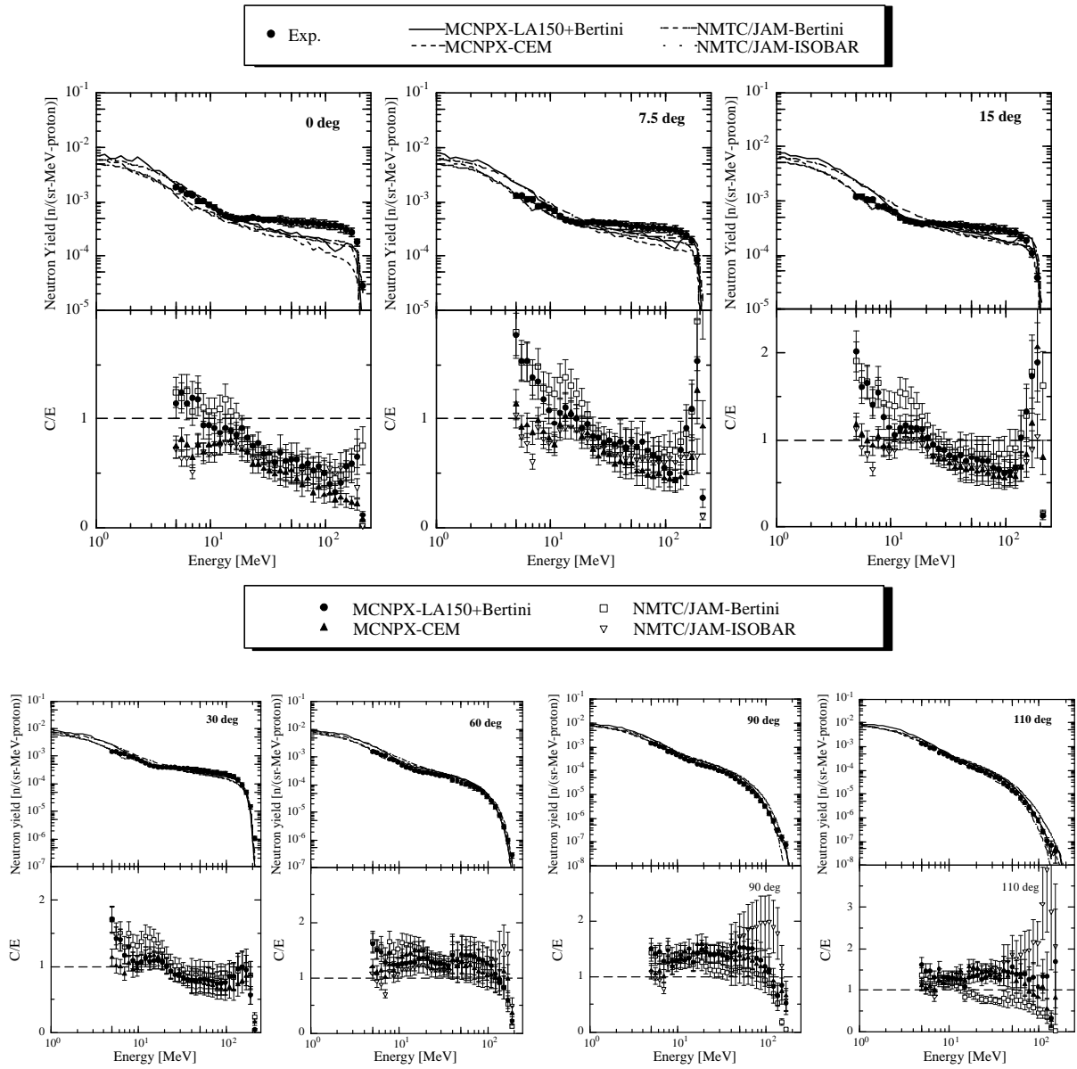
Figure 2: Neutron energy spectra from the iron target bombarded by 210 MeV proton compared with the calculations at angles of 0, 7.5, 15, 30, 60, 90 and 110° [20]
