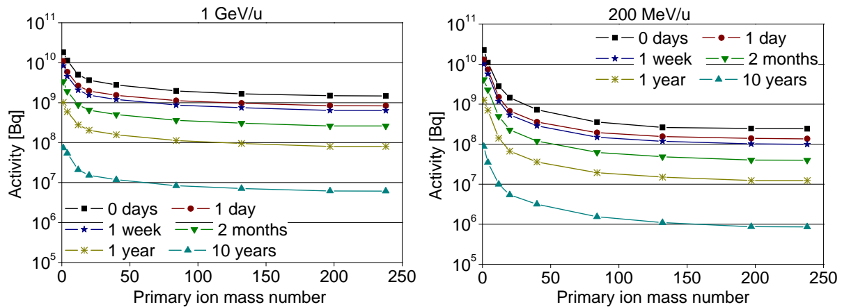
Figure 5: Activity of the stainless steel beam pipe induced by 1 W/m of primary beam loss at 1 GeV/u (left) and 200 MeV/u (right) calculated by FLUKA
