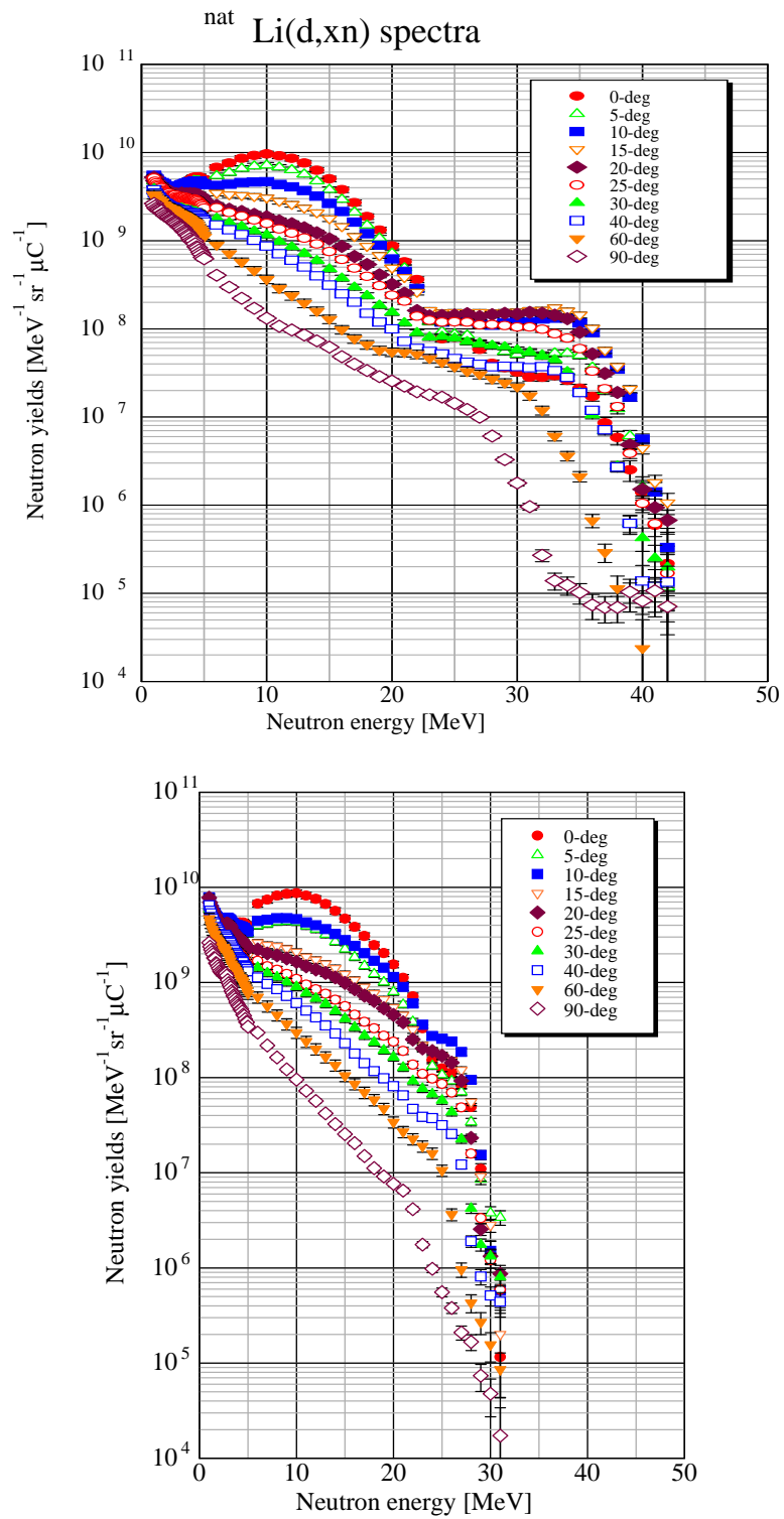
Figure 5: The results of thick-target neutron yields for (a) the \text{Li}(d,n) reaction and (b) the {}^9\text{Be}(d,n) reaction for incident deuteron energy of 25 MeV [45]
