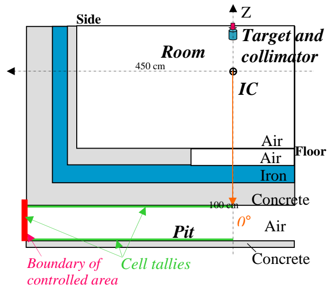
Figure 5: The calculation model of estimation for iron thickness
