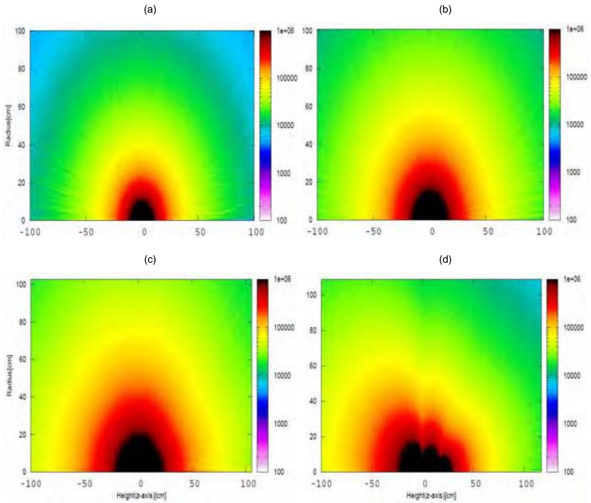
Figure 4: Ambient dose equivalent rates for a stainless steel target [ \mu\text{Sv/h} ], impacted by a proton beam of: (a) 50 MeV, (b) 100 MeV, (c) 200 MeV and (d) 400 MeV after a cooling time of one day
