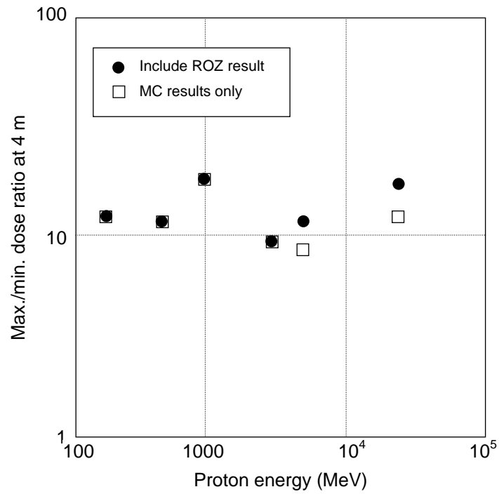
Figure 15: Neutron dose difference at 4 m inside iron from secondary neutrons emitted to 90° between ROZ 6.6, FLUKA, MARS, GEANT4 and PHITS
