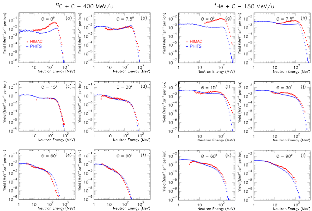
Figure 2: Comparison of the neutron doubly differential thick-target yields calculated with PHITS and the HIMAC data obtained for: (a-f) 400 MeV/u ^{12}\text{C} ions and (g-l) 180 MeV/u ^4\text{He} ions stopping in graphite
