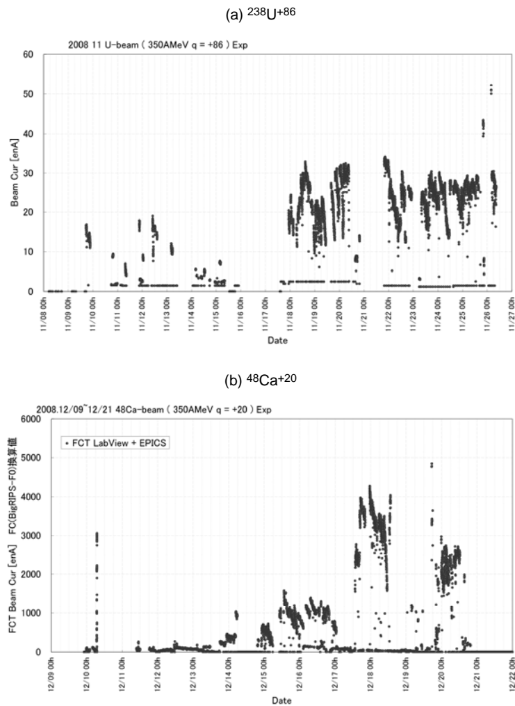
Figure 2: Beam current during the irradiation. The y axis is the electric current in nA.
