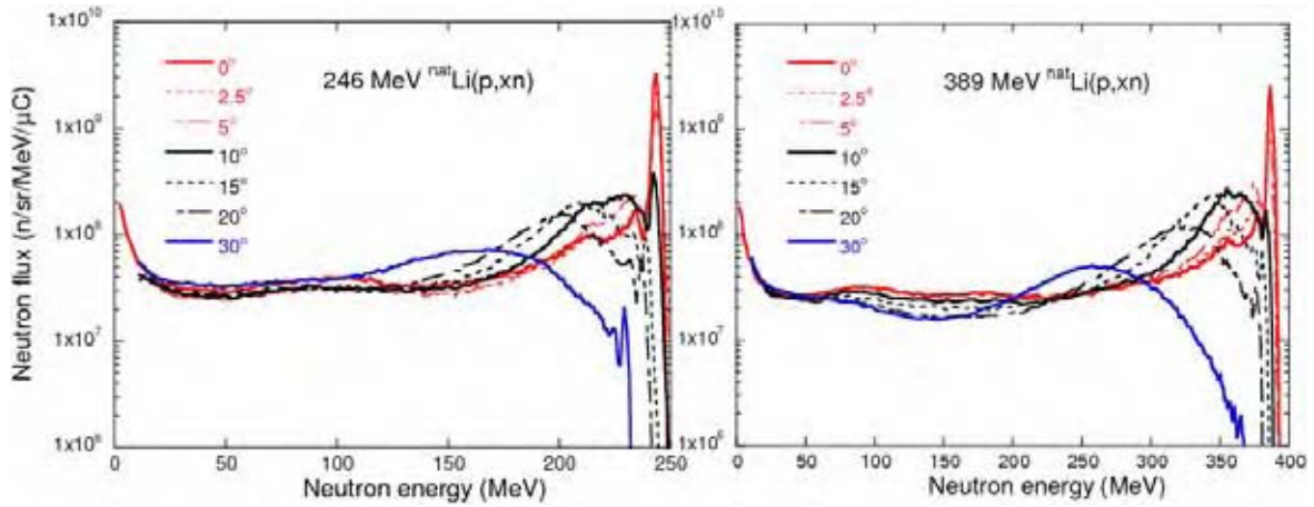
Figure 6: Angular distribution of neutron energy spectra
