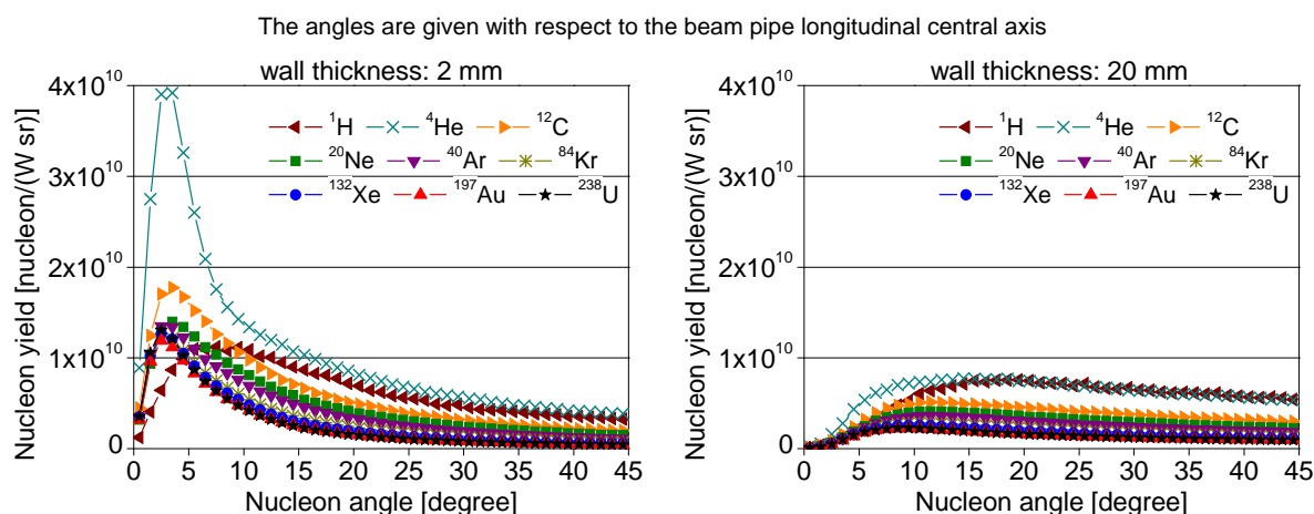
Figure 12: Angular distribution of nucleons escaping from the beam pipe for wall thickness of 2 mm and 20 mm
