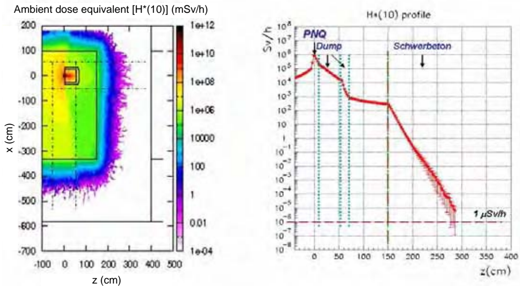
Figure 6: Ambient dose equivalent rate distribution in a vertical projection containing the source and crossing the roof in heavy concrete (left). On the right side the H^*(10) rate profile calculated along a narrow column that contains the source is also shown.
