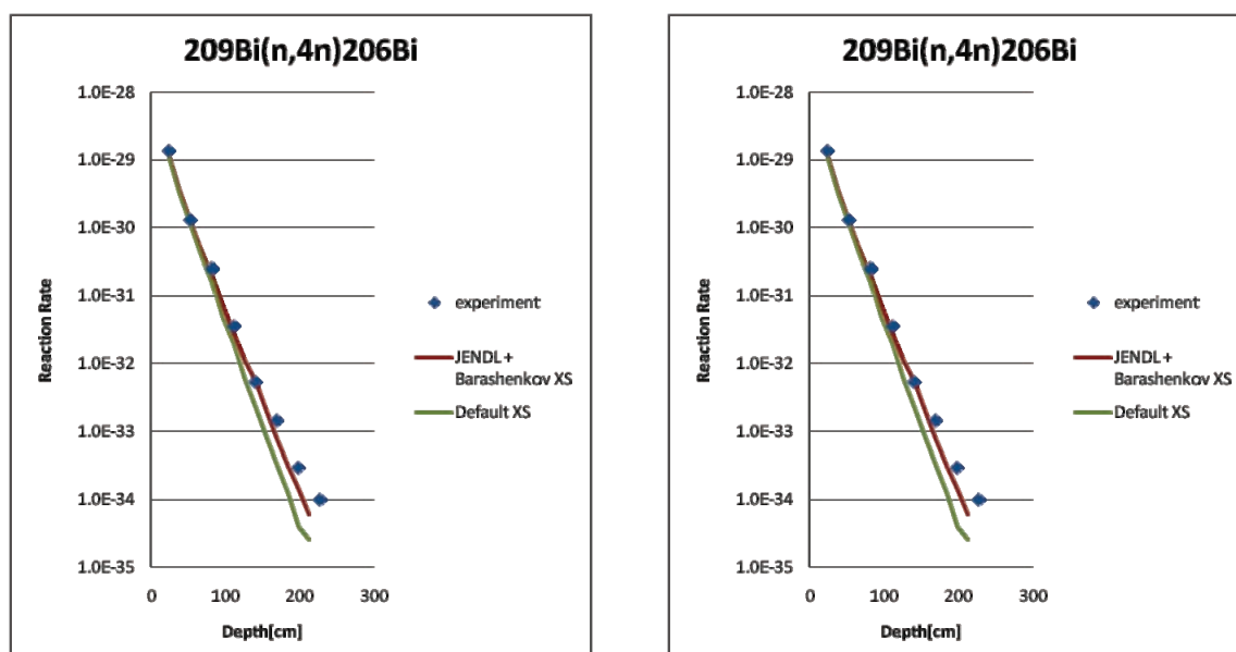
Figure 1: Comparison of calculated and measured reaction rates for the steel shield
