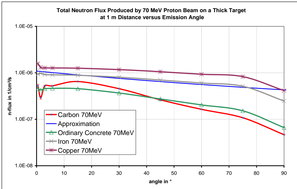
Figure 1: Total neutron flux produced by a 70 MeV proton beam directed onto a thick target at 1 m distance versus emission angle – comparison for various target materials with the approximation
