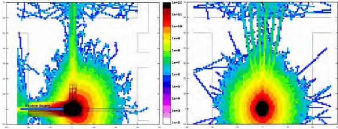
Figure 3: Spallation target and fission targets areas. Neutron flux ( n\text{ cm}^{-2}\text{ mA}^{-2} ), FLUKA performed calculations.
