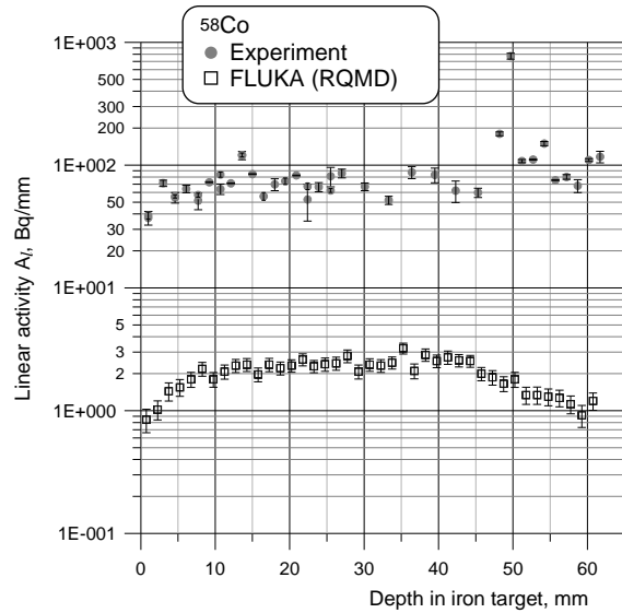
Figure 8: Experimental and simulated ^{58}\text{Co} activity distribution inside the target
