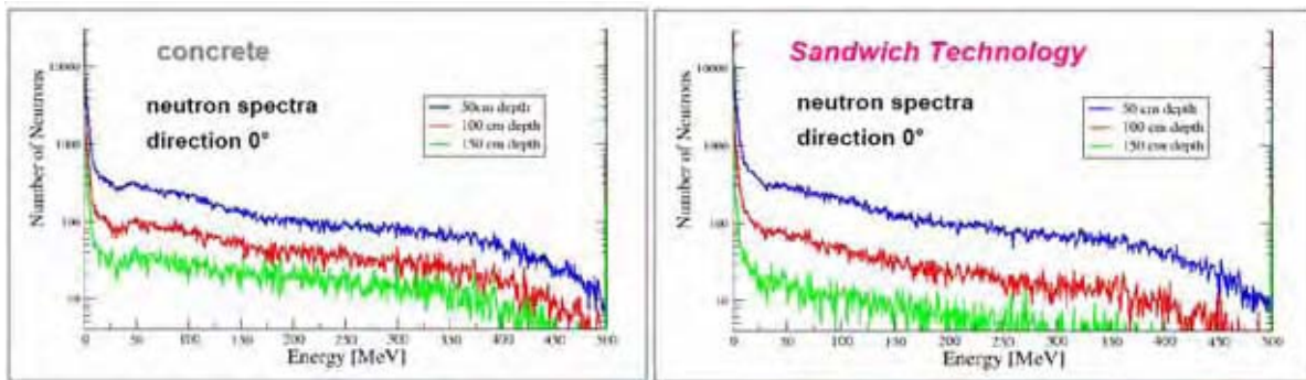
Figure 5: Energy spectra of the neutrons generated by 430 MeV/u carbon ions in a graphite target depending on different layers of shielding material; optimised mineral mixture of sandwich technology is obviously more effective than concrete
