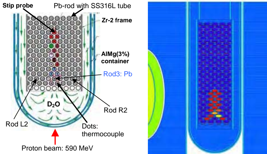
Figure 1: Left: Sketch of the SINQ target insert No. 4. The tubes are from steel 316L and filled with lead. Right: Cut through the geometrical model built in MCNPX. Due to the oblique cut, the cross-section of the rods looks oval shaped.
