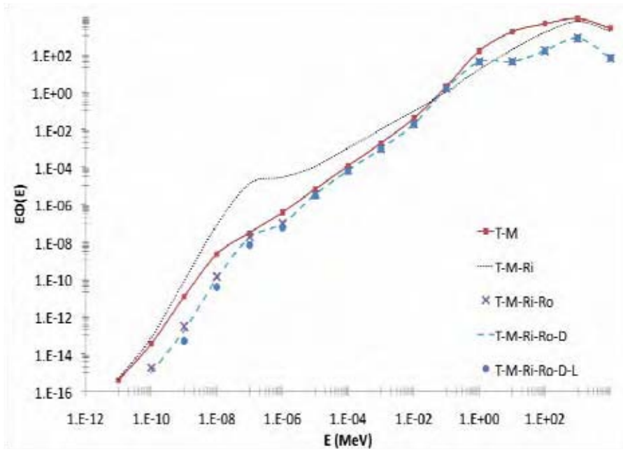
Figure 5: Neutron lethargy escaping the target system
