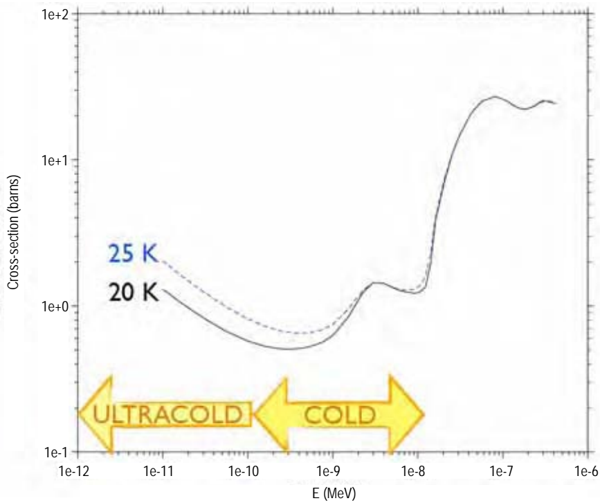
Figure 8: S(\alpha,\beta) inelastic cross-sections of hydrogen at different temperatures
