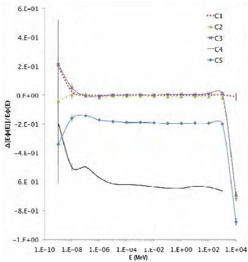
Figure 6: Fractional change in neutron lethargy escaping the target system
