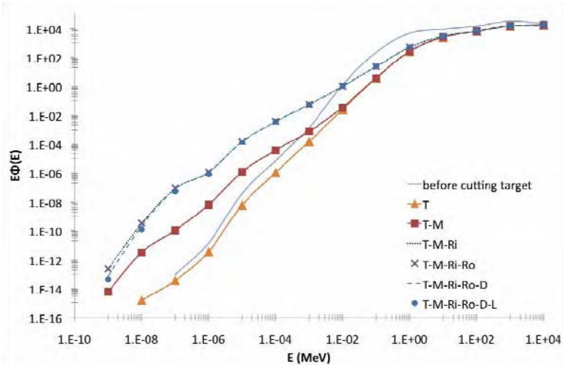
Figure 2: Neutron lethargy in the target
