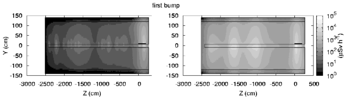
Figure 4: On the left {}^6\text{He} , on the right {}^{18}\text{Ne} – residual \text{H}^*(10) after 1 week near a quadrupole
