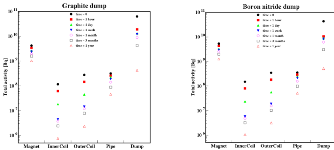
Figure 8: Total induced radioactivity (in Bq) in the dump (for graphite and boron nitride dump) and in the surrounding materials at the seven cooling times
