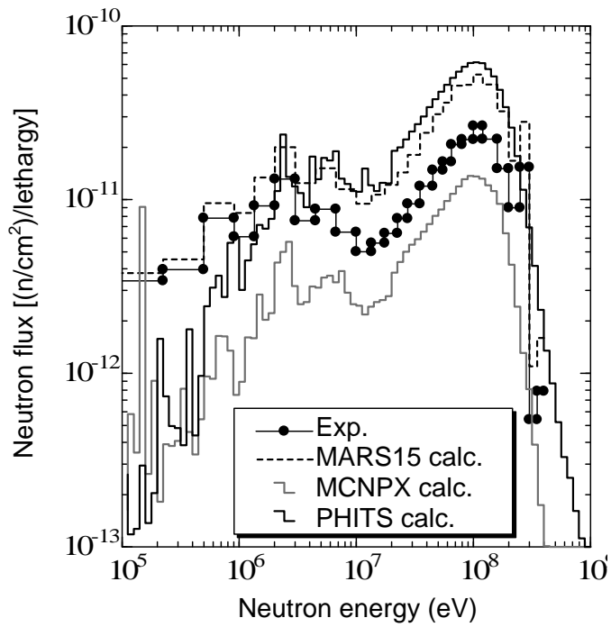
Figure 6: Neutron energy spectra above the Pbar target station measured by the Bonner spheres and calculated by the PHITS, MARS and MCNPX codes
