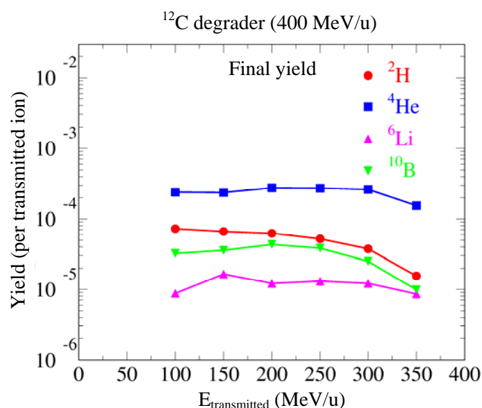
Figure 5: Evolution of the yield of secondary ions transmitted by the ESS to the patient as a function of transmitted ^{12}\text{C} beam energy
