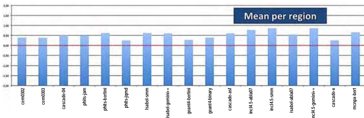
Figure 1: Rating results obtained using the method given in the upper part of Table 1 (neutron DDXS)
