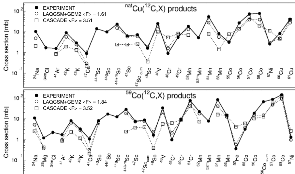
Figure 16: Comparison of measured cross-sections radioactive reaction products in Co and Cu induced by 200 MeV/nucleon C with the LAQGS+GEM2 and CASCADE calculations [84]
