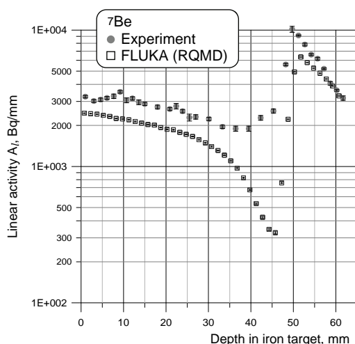
Figure 3: Experimental and simulated ^7\text{Be} activity distribution inside the target
