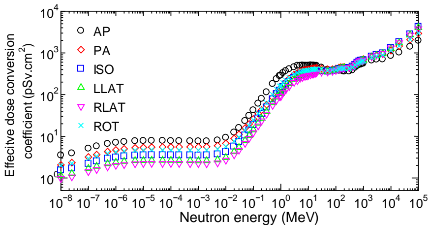
Figure 3: Irradiation-geometry dependence of the effective dose conversion coefficients for neutrons calculated by PHITS [7]
