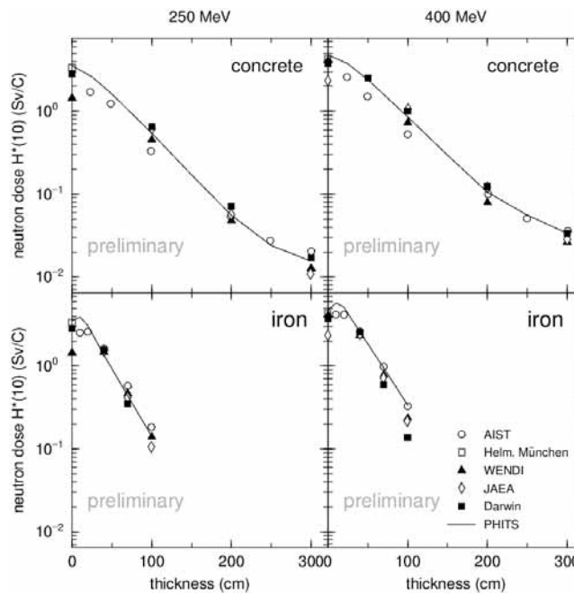
Figure 4: Preliminary results of the measured and calculated neutron dose attenuation
