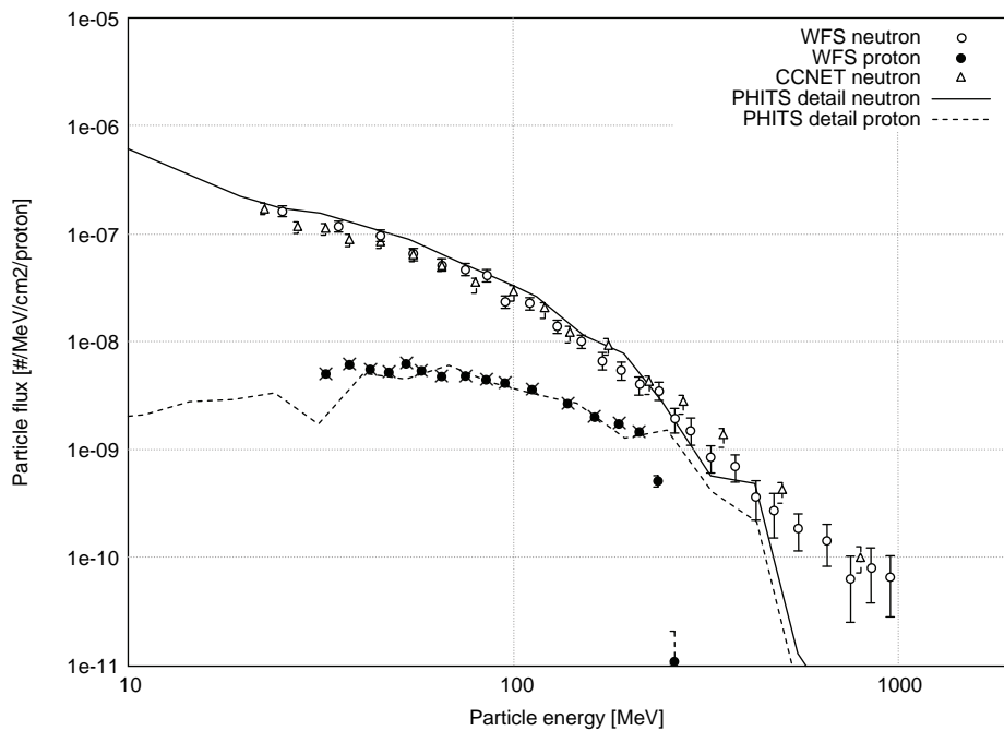
Figure 12: 120 GeV proton-induced proton and neutron thick target yields at 90° using a wave form digitiser DAQ system
