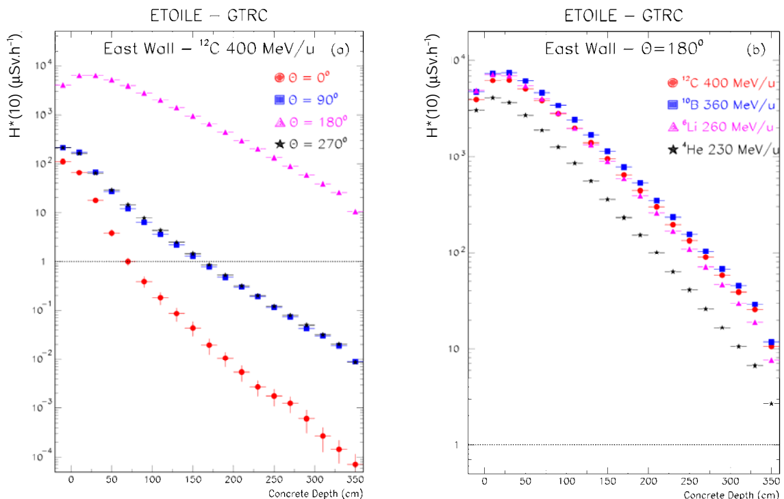
Figure 9: Evolution of ambient dose equivalent as a function of concrete depth in the east wall of the carbon gantry room: (a) 400 MeV/u ^{12}\text{C} ions with different gantry rotation angles; (b) various ion species with the same gantry orientation angle of 180^\circ
