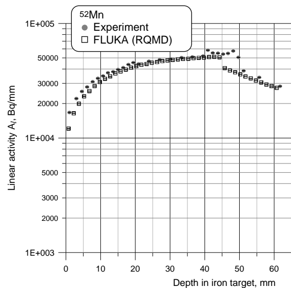
Figure 7: Experimental and simulated ^{52}\text{Mn} activity distribution inside the target
