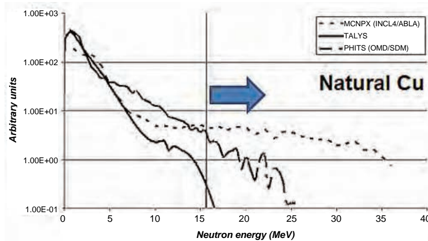
Figure 6: Probability distribution of emitted neutrons for ^{nat}\text{Cu} and 9 MeV incident deuterons
