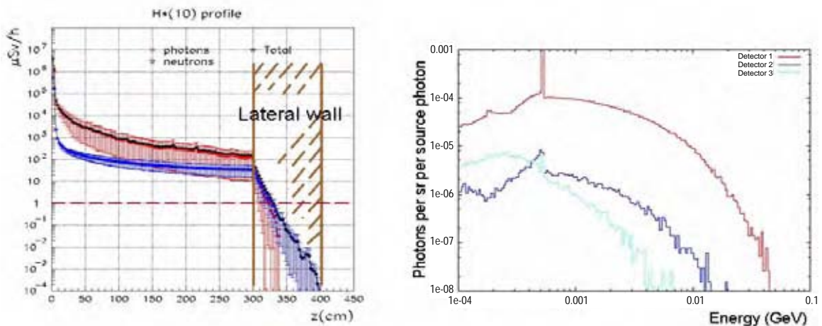
Figure 8: H^*(10) rate profile through a lateral wall (left), obtained by averaging the FLUKA data on a volume that crosses the horizontal plane containing the beamline and is narrow in y (20 cm) and several meters long in x ; photon energy spectra calculated on different scoring surfaces, as illustrated in the text (right)
