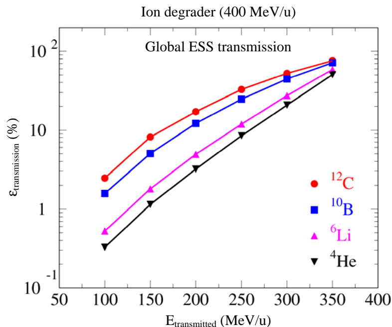
Figure 6: Variation of ESS transmission efficiency as a function of beam transmitted energy for the various ions produced by the C400
