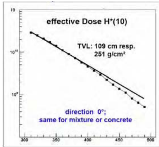
Figure 4: Calculated effective dose H^*(10) for 220 MeV protons and a sandwich wall by double convolution
