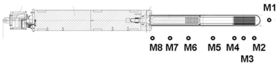
Figure 7: Layout of the Target 4 insert. The labelled dots indicate the locations of the measured dose rate.
