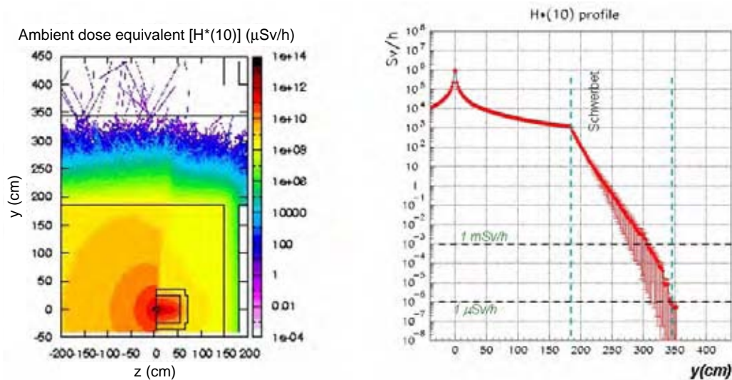
Figure 6: Ambient dose equivalent rate distribution in a vertical projection containing the source and crossing the roof in heavy concrete (left). On the right side the H^*(10) rate profile calculated along a narrow column that contains the source is also shown.
