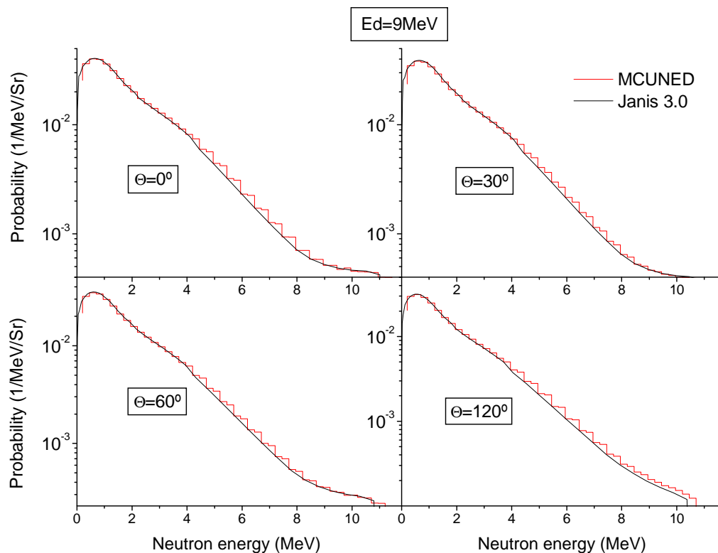
Figure 7: Neutron double differential cross-section for the reaction d-^{63}\text{Cu} and 9 MeV deuterons
