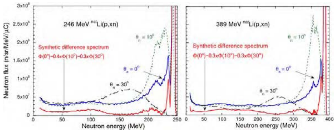
Figure 8: 0^\circ , 10^\circ and 30^\circ spectra and synthetic difference spectrum
