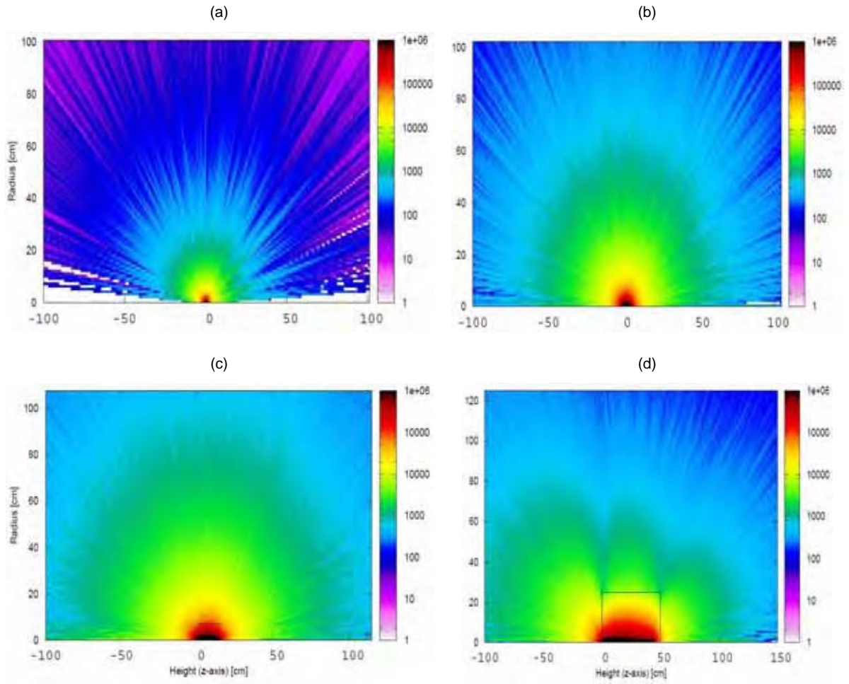
Figure 2: Ambient dose equivalent rates for a carbon target [ \mu\text{Sv/h} ], impacted by a proton beam of: (a) 50 MeV, (b) 100 MeV, (c) 200 MeV and (d) 400 MeV after a cooling time of one day
