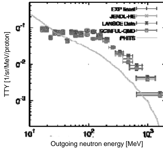
Figure 11: 120 GeV proton-induced neutron thick target yield at 90° using a CAMAC DAQ system
