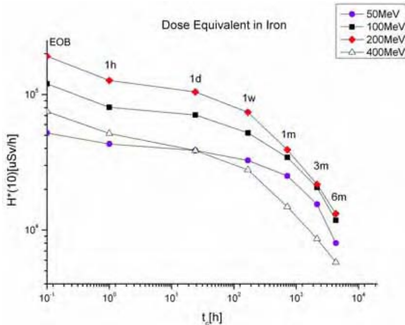
Figure 8: Ambient dose equivalent rate, as a function of cooling time, from an iron target impacted by a proton beam of the indicated energies
