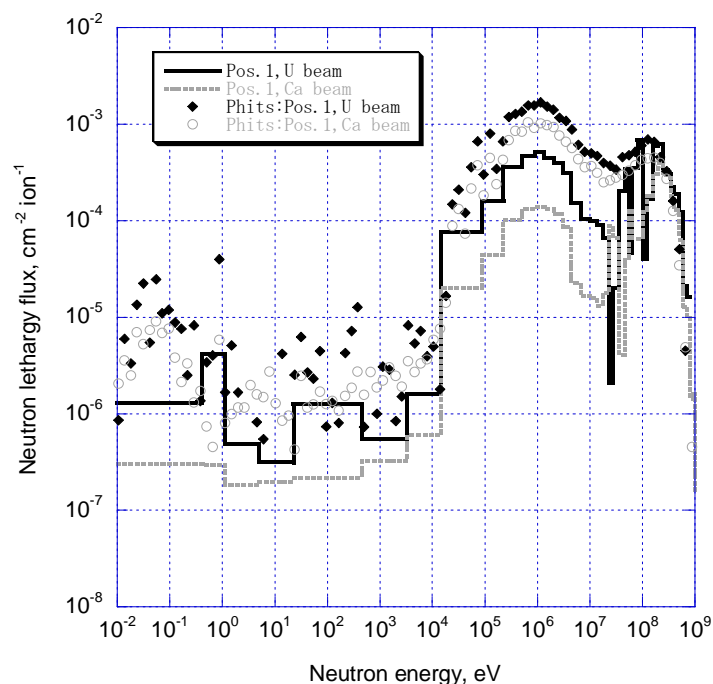
Figure 6: Neutron spectra near the target at 30° from beam direction. Histograms are the measured data and the marks are the PHITS results. 24 Na production data were ignored in the unfolding process.
