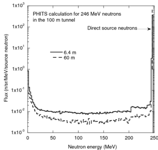
Figure 4: Calculated results of neutron energy spectra at 6.4 and 60 m in the 100 m tunnel for the 246 MeV neutron incidence
