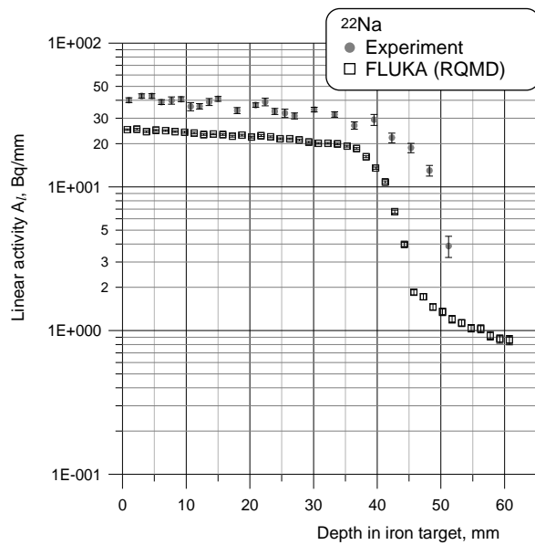
Figure 4: Experimental and simulated ^{22}\text{Na} activity distribution inside the target
