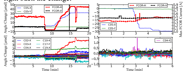
Figure 1: Comparison between (left) v2 bump with FOFB “relaxed” mode and (right) v3 bump with normal FOFB, showing horizontal 30-urad bump creation at C05 ID (top) and the impact on all the other ID sources (bottom).
