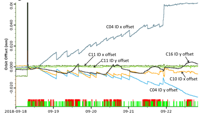
Figure 2: Local Bump Agent working hard to maintain C11 ID bump offset during the C04 orbit drift event. The red bars at the bottom indicate when any of the ID gaps was moving, while the green bars show when any local bump correction was happening.
