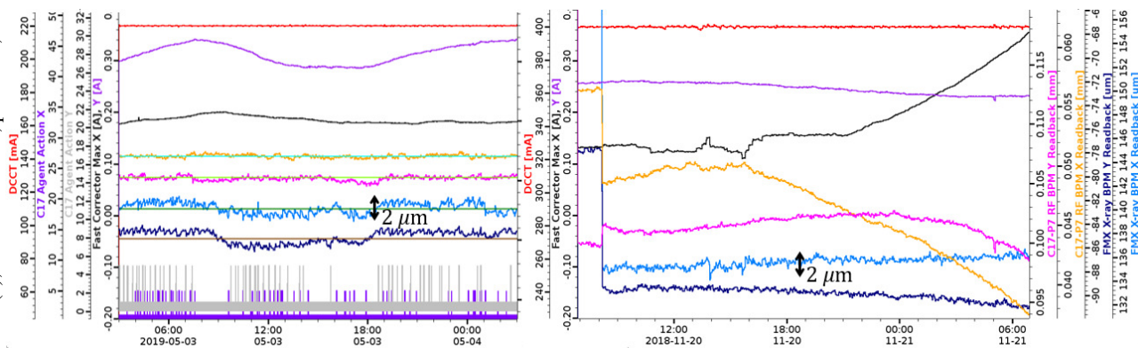
Figure 3: Performance of v4 local bump agent (feedback) (left) and PLFB (right).
