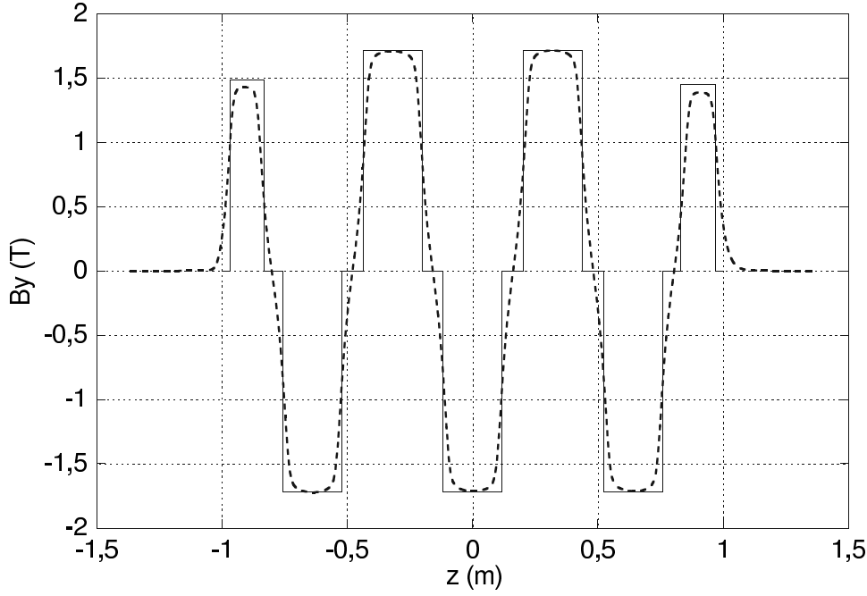
Figure 4.7: The wiggler field along the longitudinal z axis: the dashed line is the measured field and the full line the hard-edge model.
