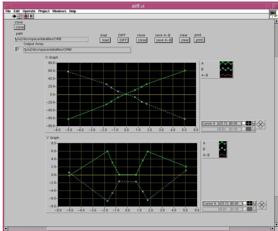
Figure 2.5: Horizontal and vertical trajectories of the electron and positron beams along IR1 as they are shown by the DAΦNE control system, for beams colliding in IP1.
