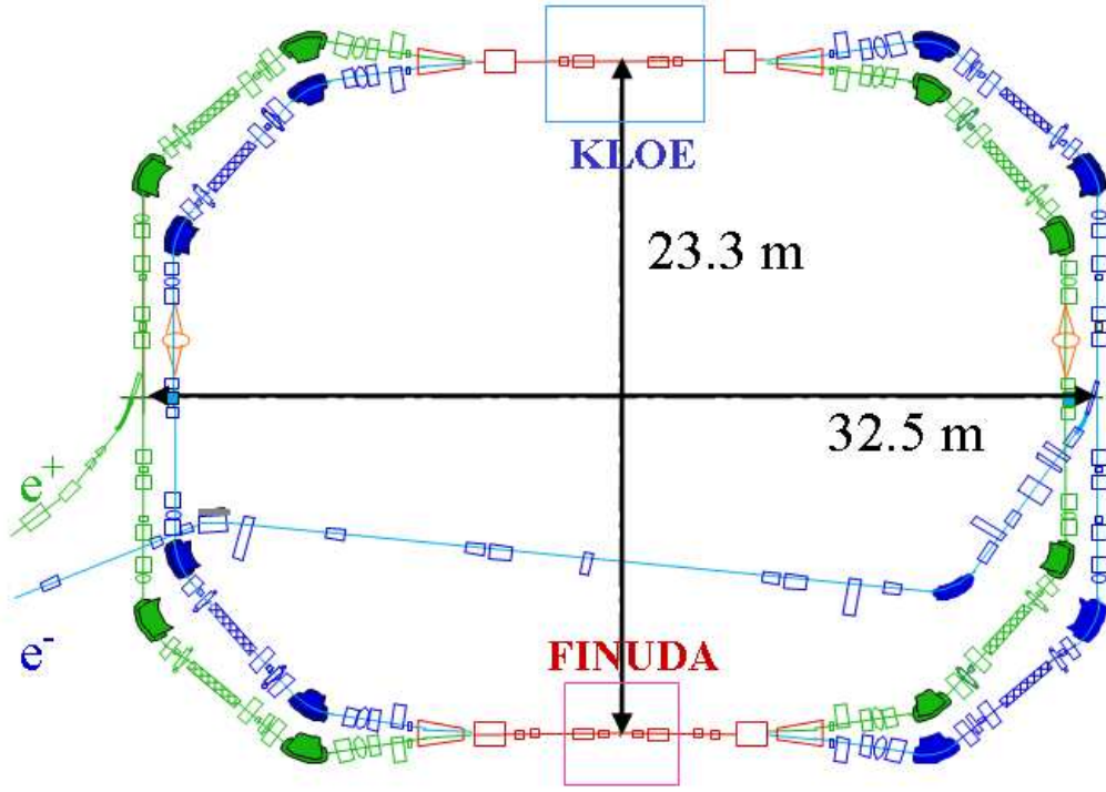
Figure 2.2: Layout of the DA\Phi NE main rings.
