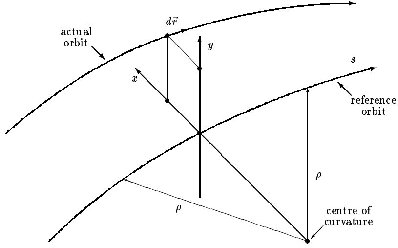
Figure 2.3: The coordinate system employed to describe the particle motion.
