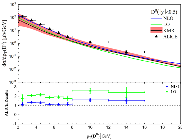
Fig. 4 The differential cross section of D^0 compared with ALICE data and the KMR model at 2 < p_T < 20 GeV
