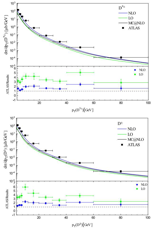
Fig. 3 The differential cross sections of D^{*\pm} (up) and D^\pm (down) mesons as a function of p_T compared to ATLAS data (symbols)
