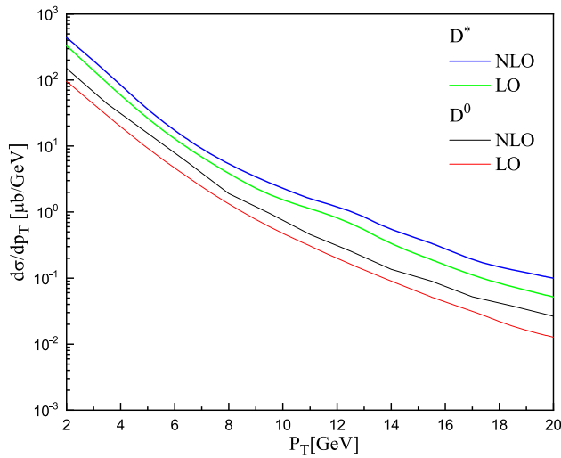
Fig. 2 The differential cross sections of D_0 and D^* mesons as a function of p_T in |\eta| < 0.5
