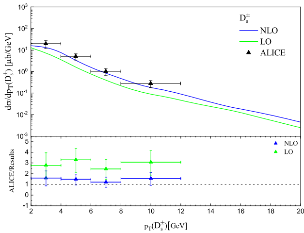
Fig. 1 The differential cross sections of mesons D_s^\pm as a function of p_T compared to ALICE data
