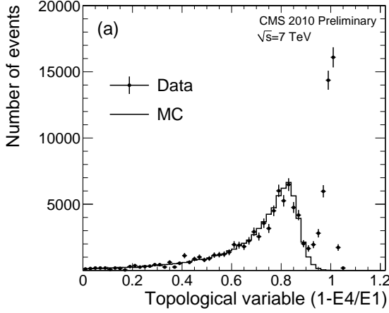
Figure 4.23: Distribution of the “Swiss Cross” topological variable ( 1 - E_4/E_1 ) for data and simulation. Only deposits with E_T > 3 GeV are plotted [187].
