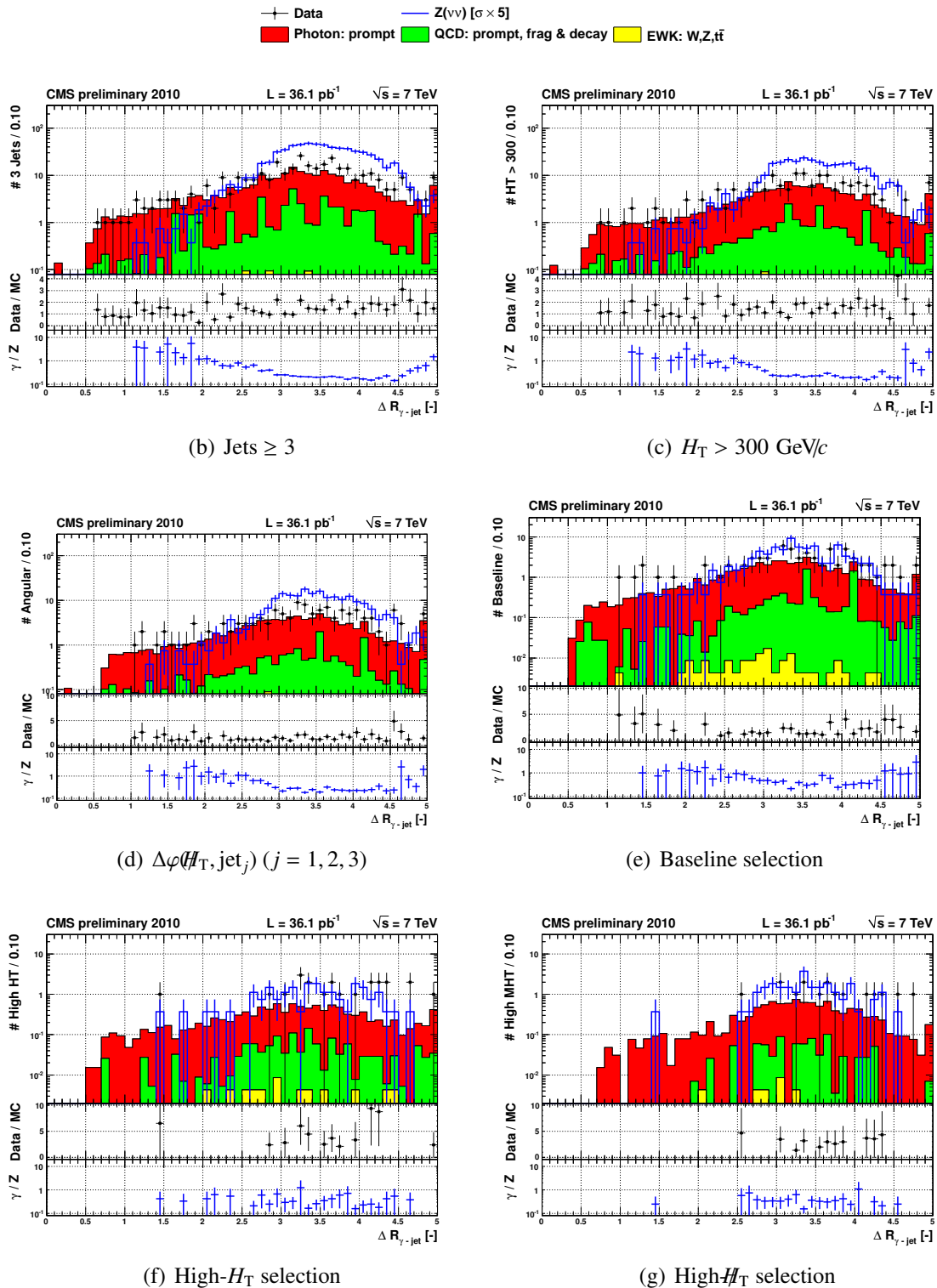
Figure 7.14: \Delta R(\gamma, \text{jet}) plots at different stages of the event selection. The simulated Z(\nu\bar{\nu}) + \text{jet} distributions are shown for comparison. They are scaled up to the total Z + \text{jet} cross section ( \sigma_{Z+\text{jet}} = 5 \times \sigma_{Z(\nu\bar{\nu})+\text{jet}} ).
