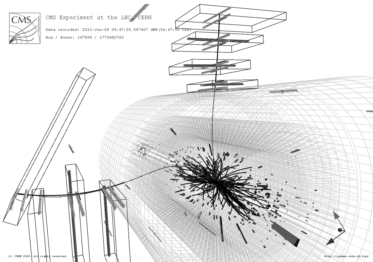
Figure 3.9: Event display of a B_s \rightarrow \mu\mu -candidate of event 1 773 682 763 recorded in run 167 898. Two particles identified as muons emerge from the tracker and leave hits in the DTs and RPCs [158].
