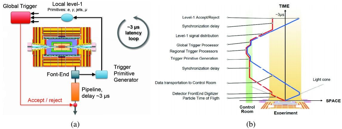
Figure 3.27: Illustrations of the Trigger Latency of the Level 1 Trigger [131].
