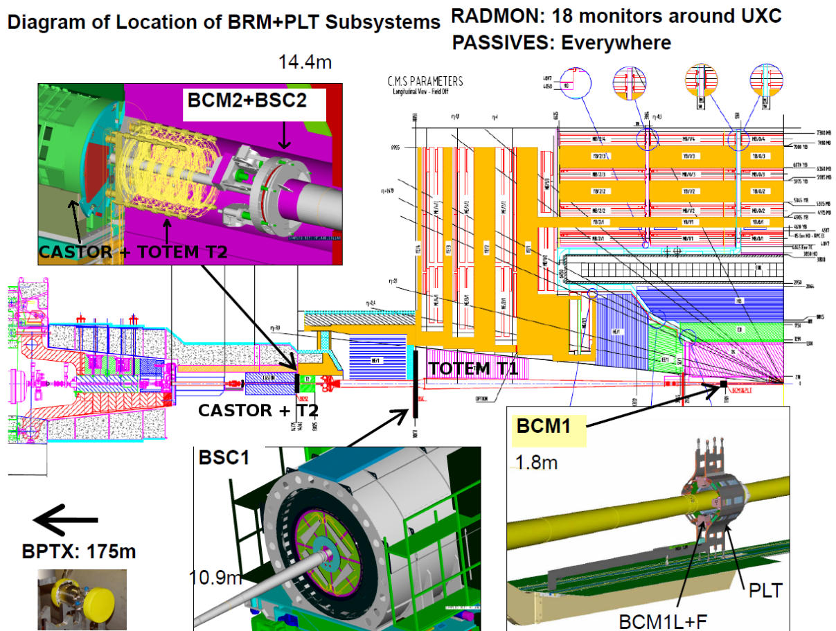
Figure 3.24: Layout of a quarter of the CMS detector and the very forward region. The different BRM sub-systems are shown, in addition to the TOTEM T1 and T2 telescopes and the CASTOR calorimeter [131].
