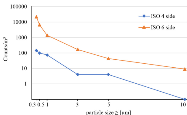
Figure 4: Measured particle concentrations during roll-up door operation inside the lock (ISO 4) and on the ISO 6 side.
