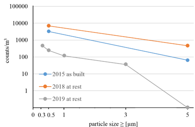
Figure 3: Particle concentrations at the “worst” spot of CR 1 during classification measurements after the CR was built (2015), altered (2018) and today.
