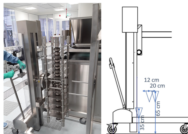
Figure 5: Left: Photo of the lift trolley handling over a cavity in its frame to the lifter system of the ultrasonic bath. Picture was taken during the testing of the cleanroom infrastructure with a 3 GHz cavity from TU Darmstadt [20]. Right: Sketch of the probe positions during particle measurements without cavity.
