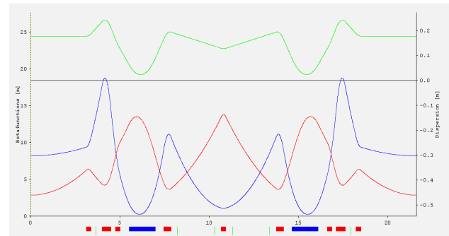
Figure 7: Elettra optics for reduced emittance.
