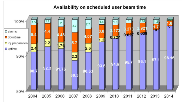
Figure 1: Availability of Elettra. The downtime is shown with red, with yellow the time lost for refilling and with light turquoise the time lost due to electricity surges.
