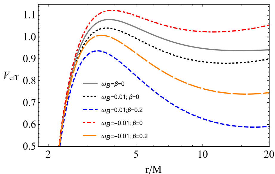
Figure 1. The radial dependence of the effective potential for magnetized and charged test particles.
