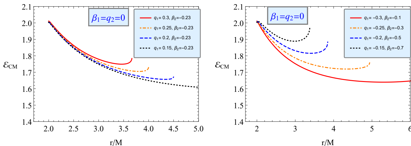
Figure 13. The same as Figure 9 but for collisions of positively charged particles with non-dipole-negative magnetized particles with no charge.
