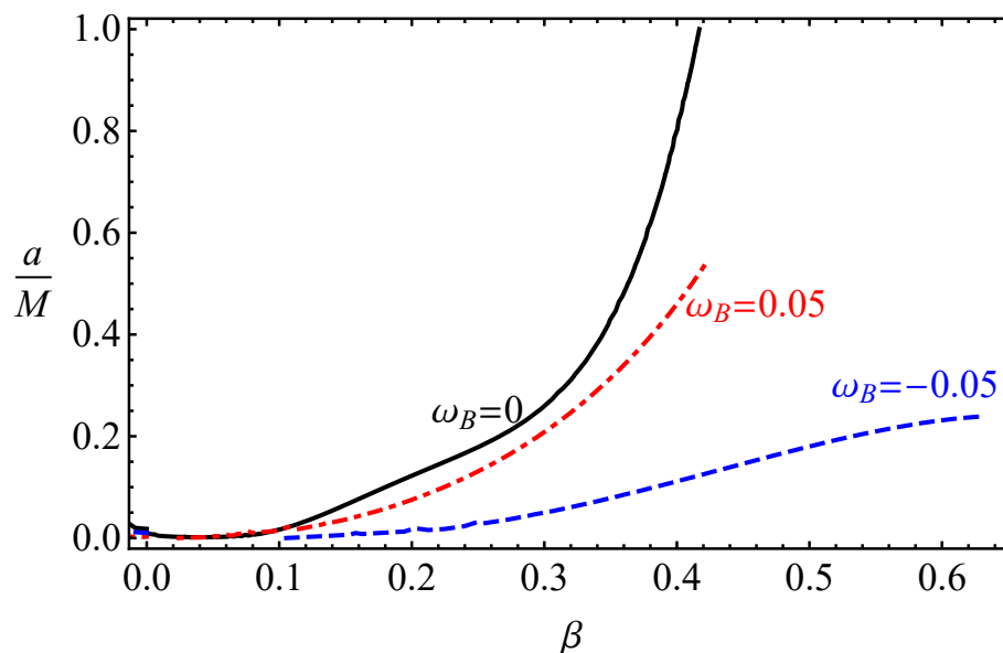
Figure 6. Degeneracy between parameter \beta and a , i.e., for a given value of \beta there exists a Kerr geometry with a given value of spin parameter a/M that has the same ISCO radius for various combinations of parameter \omega_B . The point to be noted here is that a/M represents a black hole rotation (spin) parameter.
