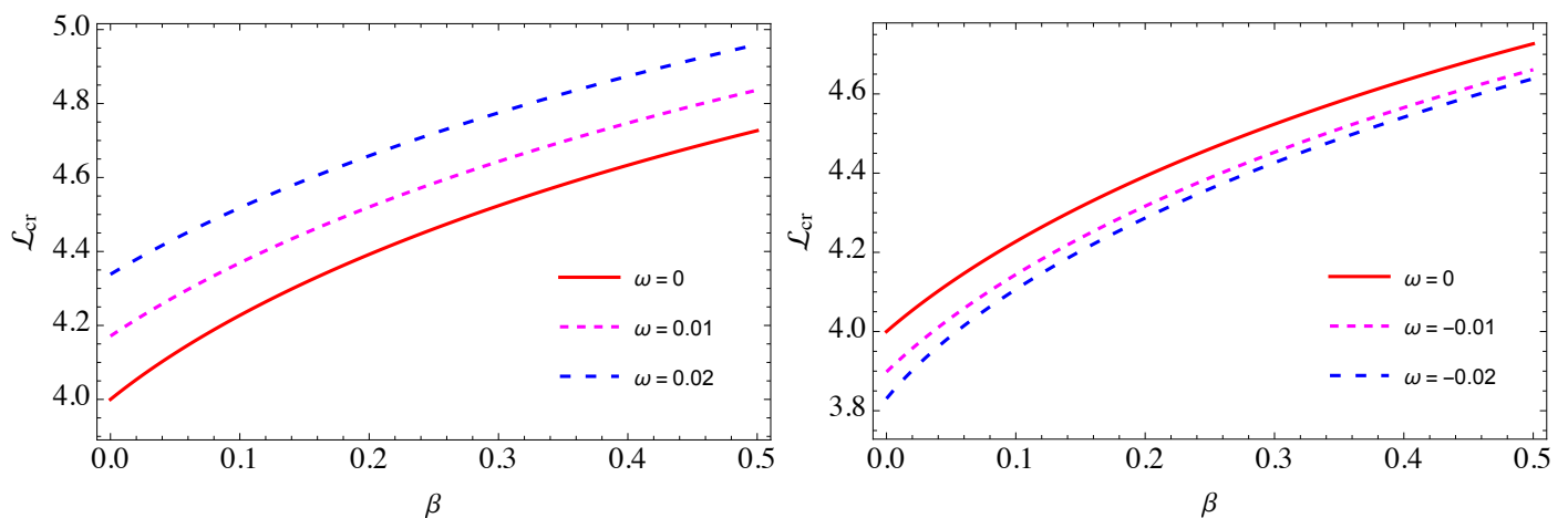
Figure 8. The dependence of critical angular momentum on parameter \beta with the different values of \omega_B .
