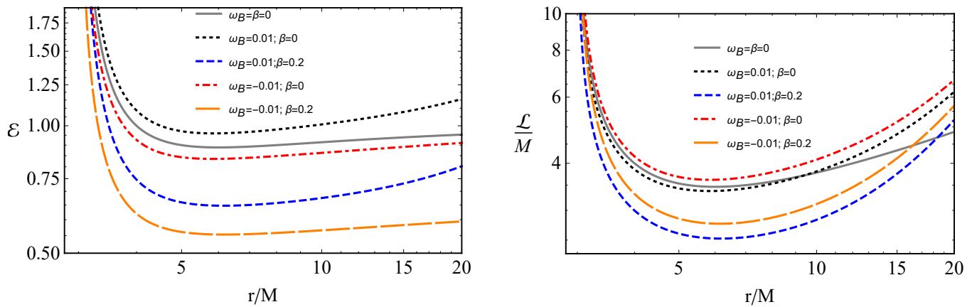
Figure 2. Radial profiles of the specific energy (left panel) and angular momentum (right panel) for magnetized and charged particles at the circular orbits.
