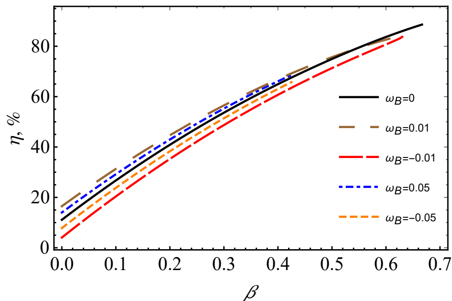
Figure 5. Dependence of the energy efficiency on the magnetic-coupling parameter \beta for different values of the parameter \omega .
