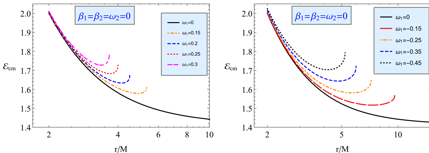
Figure 9. Figure shows the radial dependence of \mathcal{E}_{cm} of the collisions of two positively and negatively charged particles with electrically neutral particles on the different values of the charge.
