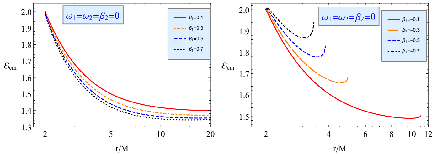
Figure 10. The same as Figure 9 but for collisions of neutral-magnetized particles with positive magnetic dipole particles.
