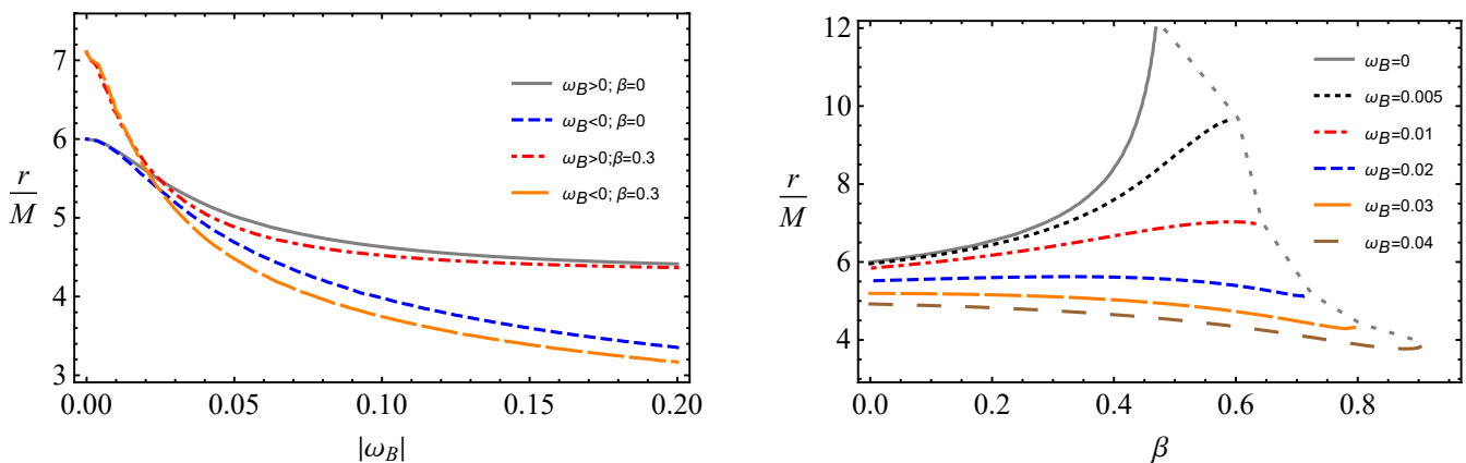
Figure 3. The dependence of the ISCO radius on the parameters \omega_B (left panel) and \beta (right panel).
