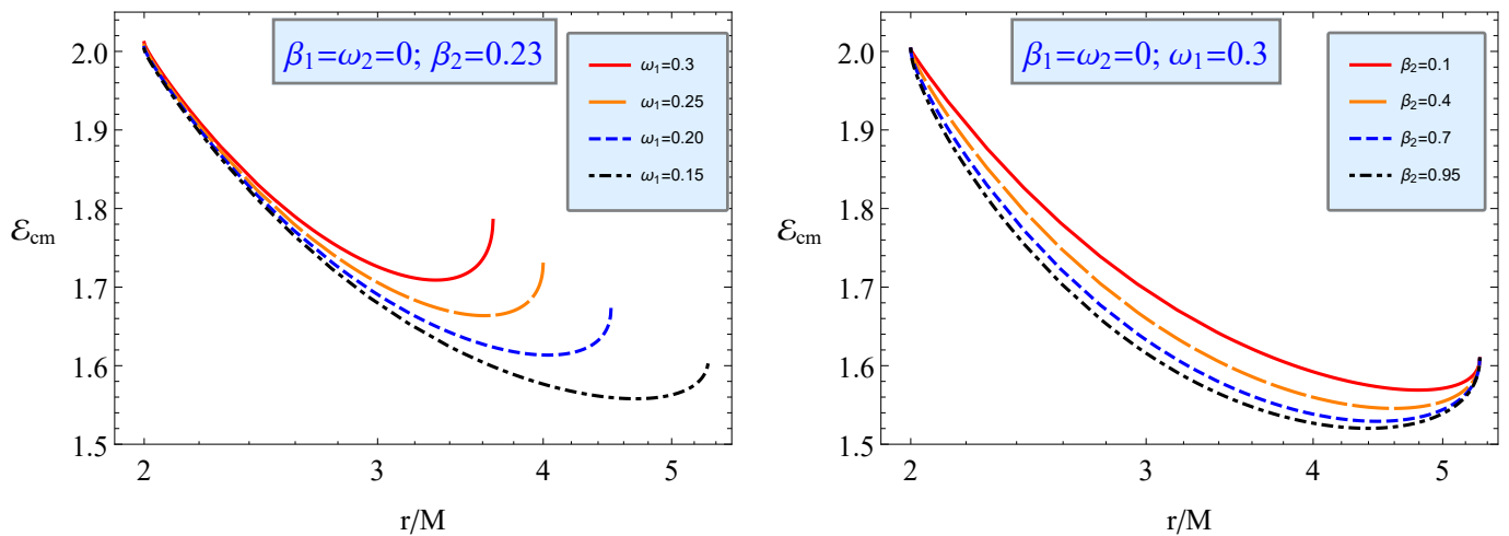
Figure 11. The same as Figure 9 but for collisions of positively charged particles with no magnetic dipole-positive magnetized particles with no charge.
