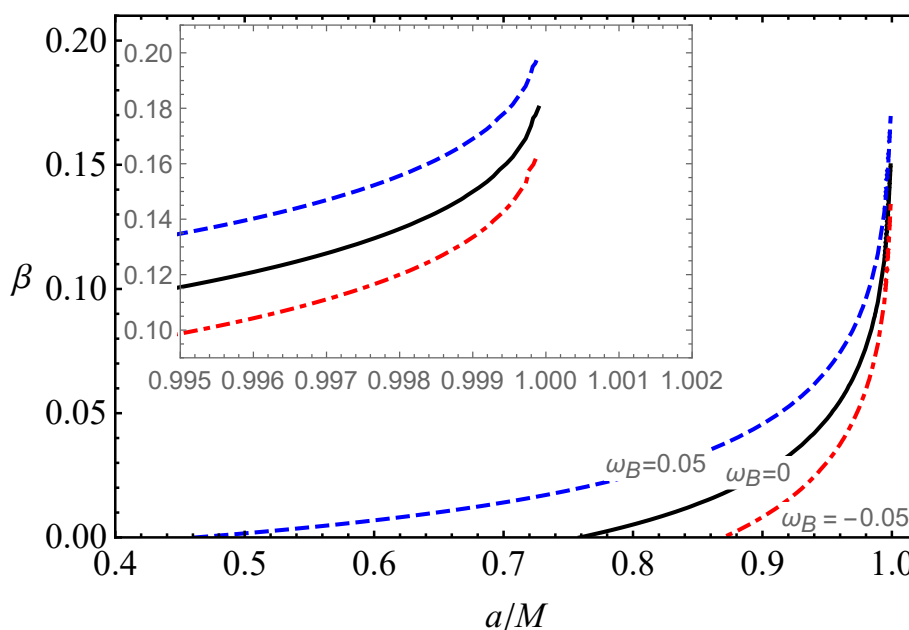
Figure 7. Degeneracy between the parameter \beta and the spin parameter of Kerr BH, providing the same energy efficiency for different values of parameter \omega .
