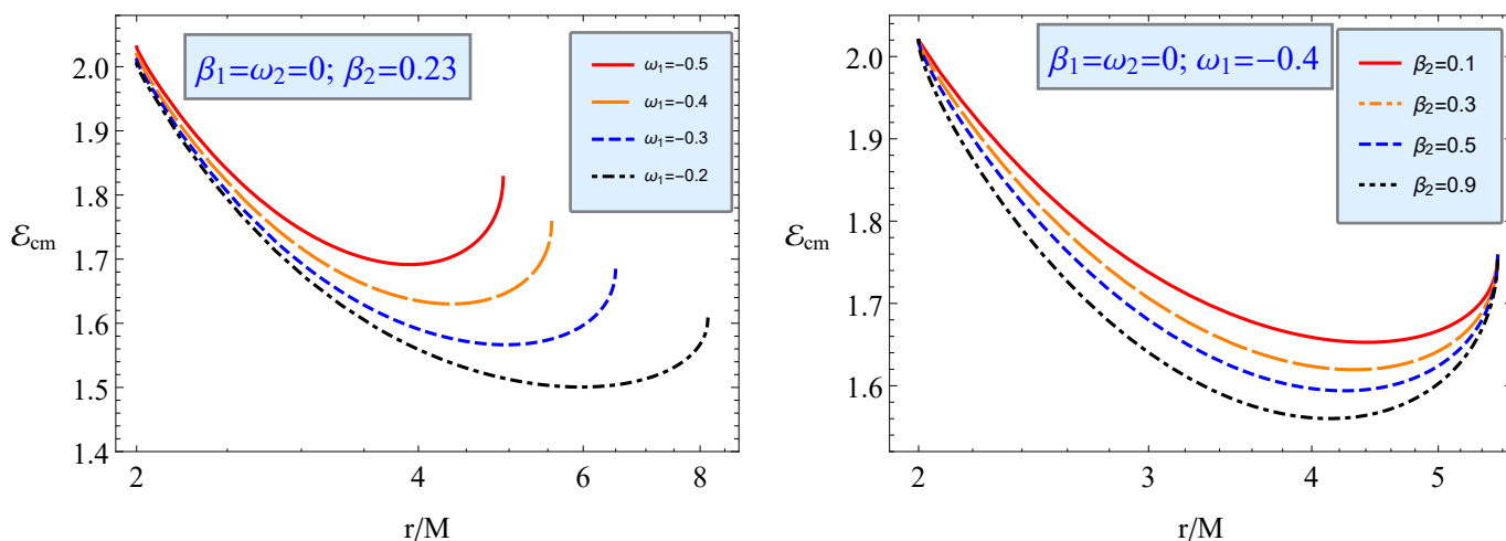
Figure 12. The same as Figure 9 but for the collisions of negatively charged particles with non-dipole-positive magnetized particles with no charge.
