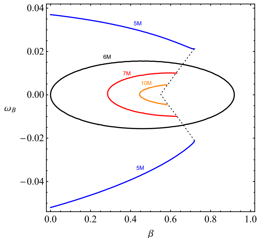
Figure 4. Possible values of parameters \omega_B and \beta for a ISCO radius between 5 and 10 M.
