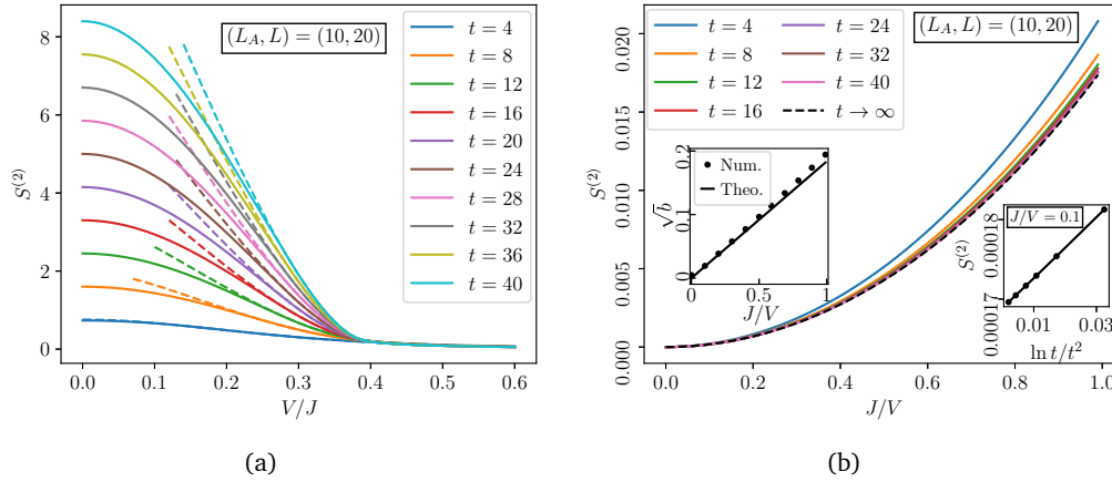
Figure 5: (a) The S^{(2)} obtained from Type 2(D/QA/QB) saddles as a function of V/J for V < 0.6J at various times. For a given value of V and t , the solid and dashed lines, if both exist, correspond to the Type 2(D) (i.e. replica diagonal) and Type 2(QA/QB) (i.e. replica quasi-diagonal) saddle, respectively; otherwise only Type 2(D) saddle solution exists for this value of V . Note the Type 1 saddle solutions are not shown in (a). (b) The Type 2(D) saddle S^{(2)} as a function of J/V for J \leq V . Long time behavior converges to a J^2/V^2 scaling form. The left inset shows that the coefficient b in front of a \log t/t^2 correction term fits well with the theoretically proposed value (see Eq. (31) and below); the right inset shows the linear S^{(2)} - \log t/t^2 scaling behavior at small J/V .
