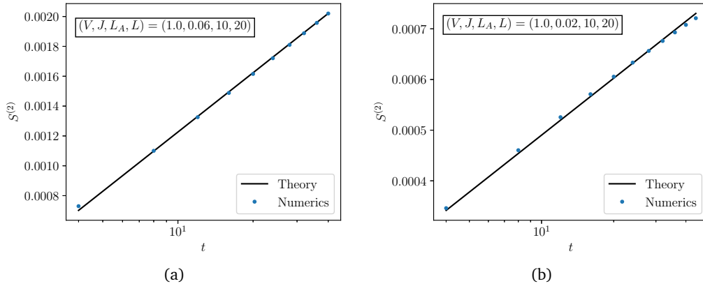
Figure 11: (a) S^{(2)} as a function of \log t in the (4,4) model in the J/V \ll 1 limit. The theory result is drawn from Eq. (49) with proper cutoff parameter \epsilon . (b) The same plot in the (2,2) model in the J/V \ll 1 limit. The theory result is drawn from Eq. (50) with proper cutoff parameter \epsilon .
