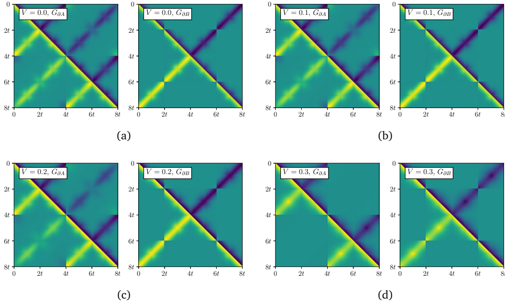
Figure 6: Green's function profile on the subsystem boundary \partial A and \partial B for various V at t = 8 . Initial condition Type 2(QA) is applied. As V increases, the saddle point solution gradually changes from a replica quasi-diagonal solution to a replica diagonal solution.
