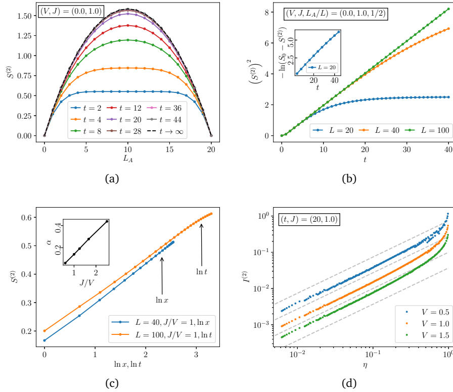
Figure 10: (a) Subsystem scaling of S^{(2)} at V = 0 . The t \rightarrow \infty curve is plotted from the analytical result Eqs. (32)–(33). (b) S^{(2)} as a function of time at V = 0 . An early time scaling S^{(2)} \propto \sqrt{t} can be observed in large enough systems. The inset shows that late time S^{(2)} exponentially saturates to S_0 = \frac{L}{4}(3 \log 2 - 2 \log(\sqrt{2} + 1)) . (c) Subsystem scaling of S^{(2)} in the intermediate regime V/J \sim 1 . S^{(2)} scales linearly with both \log x ( x \equiv \log[L \sin(\pi L_A/L)/\pi] ) with very close slopes \alpha . The inset shows \alpha scales linearly with J/V . (d) Mutual information I^{(2)} as a function of subsystem cross-ratio \eta at various V/J .
