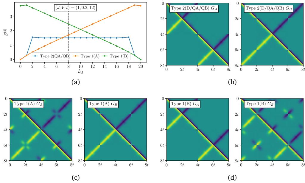
Figure 4: (a) Subsystem scaling of S^{(2)} obtained from different saddle point solutions: Type 2(QA/QB) saddle, Type 1(A) saddle, and Type 1(B) saddle. (b)–(d) The Green's function profile in the subsystem bulks \hat{A} and \hat{B} for L_A = 8 (the dashed line in (a)) corresponding to (b) the Type 2(D/QA/QB) saddles, (c) the Type 1(A) saddle, and (d) the Type 1(B) saddle.
