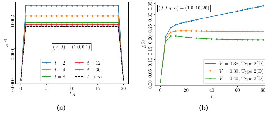
Figure 7: (a) The result for S^{(2)} vs L_A at different times at J = 0.1 . (b) The Type 2 saddle around the transition point.
