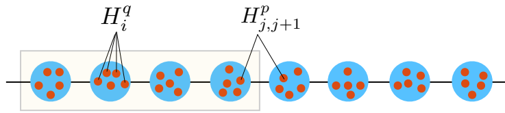
Figure 1: The cartoon for the non-Hermitian SYK model. The H_i^q represents the intra-cluster SYK model and the H_{j,j+1}^p represents the inter-cluster SYK coupling term. We compute Rényi entropy of a single interval in the box.
