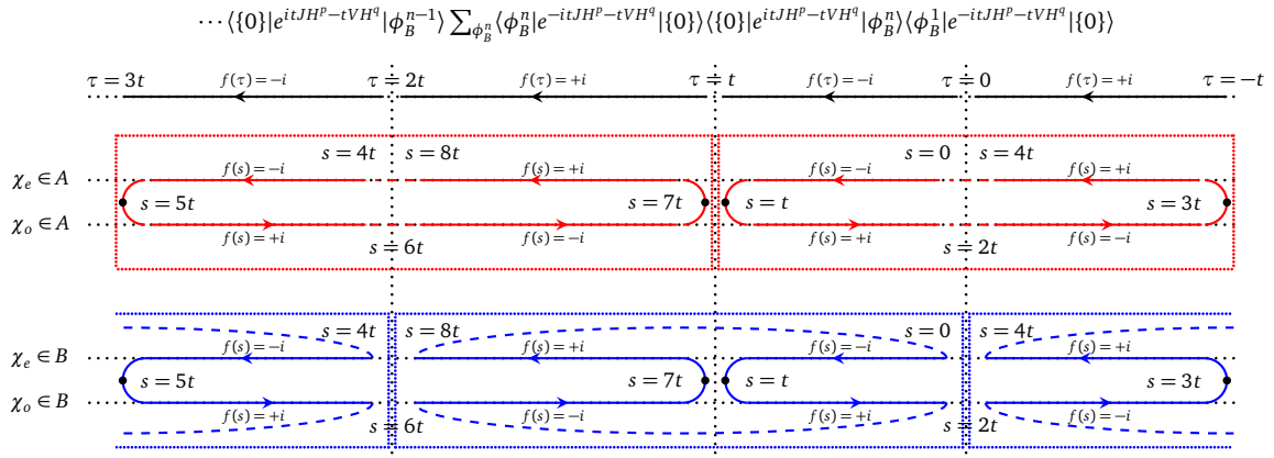
Figure 2: Time contour \mathcal{C} (solid red and blue lines) parameterized by s on the domain s \in [0, 4nt) used in Eq. (14), which combines the n replicas. The boundary conditions are shown by the dashed lines. The contour inside a blue box defines the Majorana fields of subsystem B in one replica, while the contour inside a red box defines the Majorana fields shifted by the twist field (See Appendix B). f(s) = \pm i indicates the direction of the real-time evolution (forward/backward) on the contour for \chi(s) . The original time parameterization by \tau \in [0, 2nt] is also shown (solid black line) for comparison (See Appendix A).
