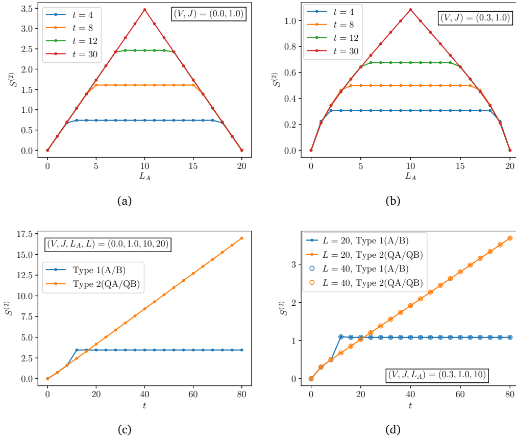
Figure 3: (a) Subsystem scaling of S^{(2)} at various t with V = 0 . (b) Subsystem scaling of S^{(2)} at various t with V = 0.3 . (c) Time dependence of the two saddle solutions at V = 0 , obtained by using numerical initial conditions Type 1(A/B) and Type 2 (QA/QB), respectively. (d) Time dependence of the two saddle point solutions at V = 0.3 . The result from two system sizes L = 20 and L = 40 shows there is no observable finite size effect.
