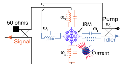
Fig. 4. Schematic representation of the JPC. The Josephson parametric amplifier (JPC) contains a Josephson ring modulator (JRM) consisting of four Josephson junctions, and four large Josephson junctions inside the ring act as a shunt inductance for the JRM (41). Two microwave resonators are coupled to the JRM forming idler and signal resonators with resonance frequencies \omega_1 and \omega_S , respectively. These resonators are capacitively coupled to the input and output ports. To use the JPC in the three-wave mixing condition, the device is biased using an external magnetic field and pumped at frequency \omega_p = \omega_1 + \omega_S . Two broadband 180° hybrids are used to feed-in and feed-out the pump, idler, and signal. In this configuration, the second port of the signal is terminated using a 50-ohm cold termination.
