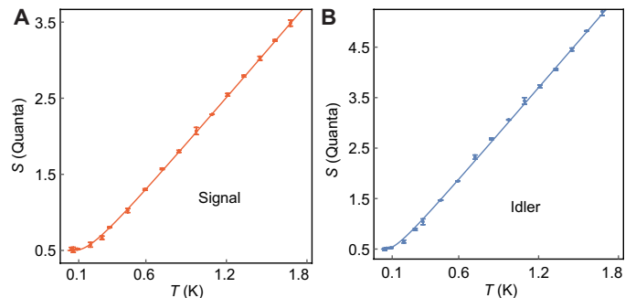
Fig. 5. System noise calibration. Calibration of signal (A) and idler (B) output channels. The measured noise density in units of quanta, S_i = N_i / (\hbar \omega_i B G_i) - n_{\text{add},i} is shown as a function of the temperature T of the 50-ohm load. The error bars indicate the SD obtained from three measurements with 576,000 quadrature pairs each. The solid lines are fits to Eq. 5 in units of quanta, which yields the system gain and noise with the standard errors (95% confidence interval) as stated in section Results.
