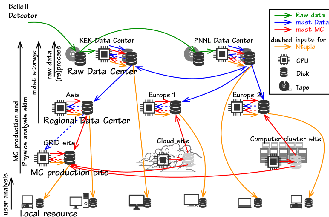
Figure 1. The Belle II computing model.
