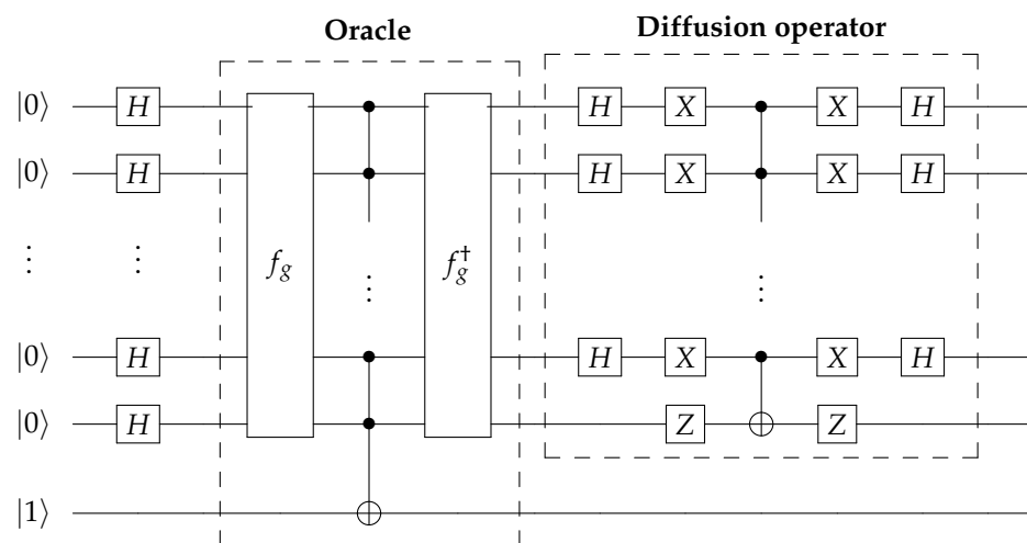
Figure 3. Grover's algorithm with f_g : \{0, 1\}^n \leftarrow \{0, 1\}^n in oracle. † indicates reversible gates.
