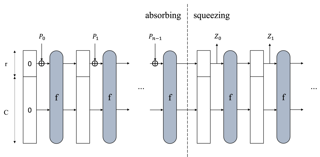
Figure 2. Operation process for SHA3 hash function. ( r : block size, c : capacity, f : Keccak-f[1600]).
