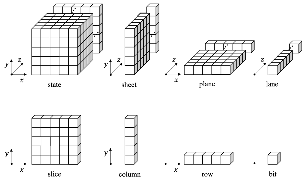
Figure 4. Each part of the three-dimensional bit array matrix state in Keccak-f[1600].
