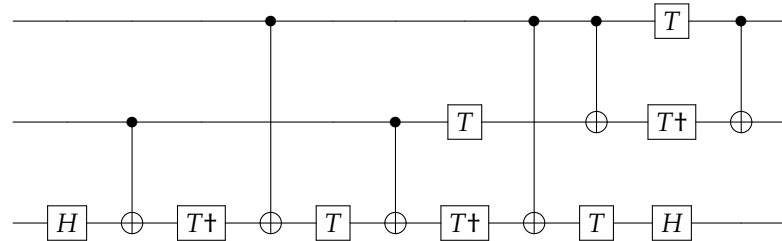
Figure 1. Decomposed Toffoli gate. † indicates reversible gates.
