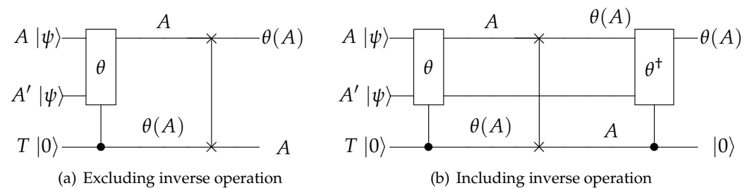
Figure 5. Quantum circuit for \theta . ( T : temporary qubits).
