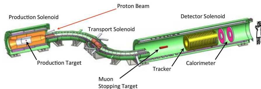
Figure 2. The Mu2e apparatus, one of two under-construction realizations of the MELC experimental concept for muon conversion searches. The full experiment is split into a production section housing the production target, a transport section that sign selects the muons of interest, and a detector section that includes a muon stopping target and detectors optimized to observe the conversion electron signal. More details can be found in the text. Image produced by the Mu2e Collaboration.
