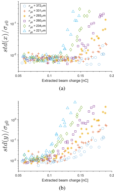
Figure 3: Beam jitters as a function of beam charge and vertical beam size measured at low beam charge in the SLS booster-to-ring transfer line.
