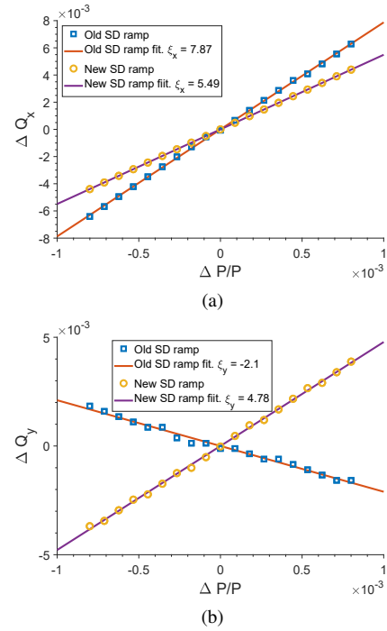
Figure 4: Chromaticity measurements at the end of the booster ramp with the old and new magnetic ramps for the SD sextupole family. The modified ramp leads to a change in chromaticity [\xi_x, \xi_y] = (+7.9, -2.1) \Rightarrow (+5.5, +4.8) .
