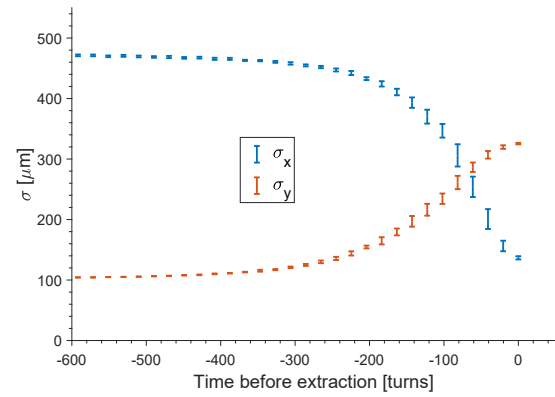
Figure 2: Beam size measurement for various extraction kicker delays on a screen monitor in the SLS booster-to-ring transfer line after applying the vertical beam size minimization.
