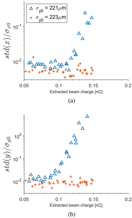
Figure 5: Beam jitters as a function of beam charge before (blue triangles) and after (red crosses) chromaticity correction.
