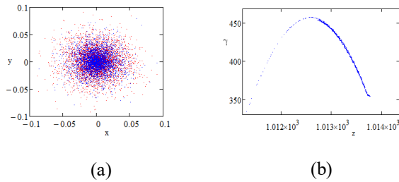
Figure 6: Beam cross section (the initial distribution is shown in red, at the output - in blue) (a) and the phase portrait on the phase plane ( \gamma , z ) (b).
