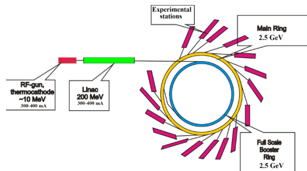
Figure 1: Planned scheme of the accelerator complex.
