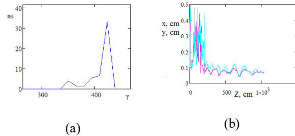
Figure 7: The energy spectrum (a) and beam envelope at injection phase -0.75.
