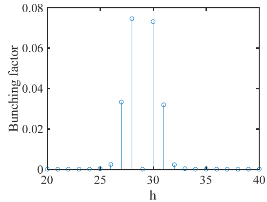
Figure 3: The bunching factor at different harmonics with A_1 = 1.5, A_2 = 1.5, B_1 = 23.2, B_2 = 0.8 .
