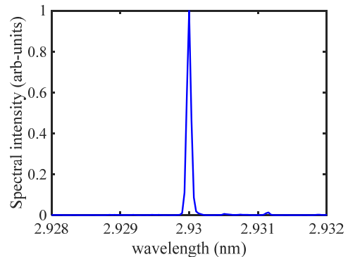
Figure 7: The final spectrum of the proposed technique.
