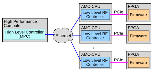
Figure 3: Communication infrastructure for a High Level Controller, running on a remote computer.
