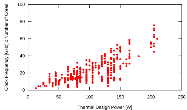
Figure 1: CPU Performance, represented by the product of clock frequency and number of cores, versus thermal design power (TDP) of various CPUs from the Intel Xeon family.
