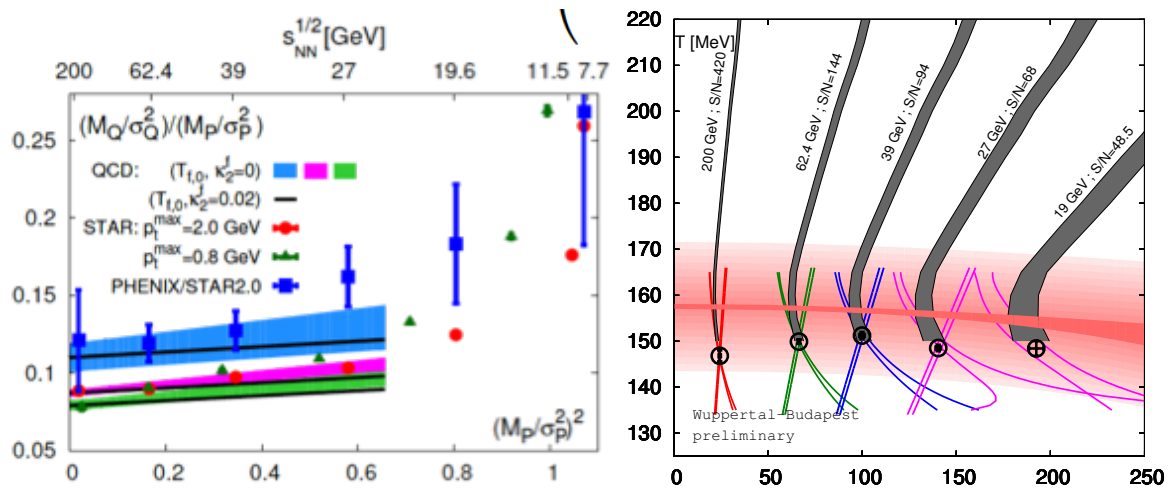
Figure 4. Left: From Ref. [47]: the ratio of ratios of \chi_1/\chi_2 for net electric charge and net-proton fluctuations measured by the STAR and PHENIX Collaborations [45, 46, 48, 49]. Right: Preliminary results of the WB collaboration. The colored full and dashed lines are the contours at constant mean/variance ratios of the net electric charge from lattice simulations. The contours that correspond to STAR data intersect in the freeze-out points of Ref. [31]. The red band is the QCD phase diagram shown in Fig. 3. Also shown are the isentropic contours that match the chemical freeze-out data [14, 15].
