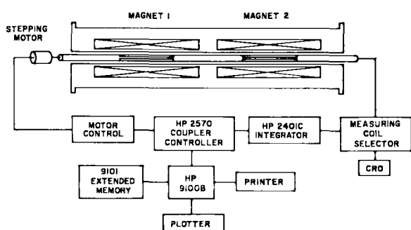
Fig. 6. Block diagram of automatic harmonic analysis apparatus.
