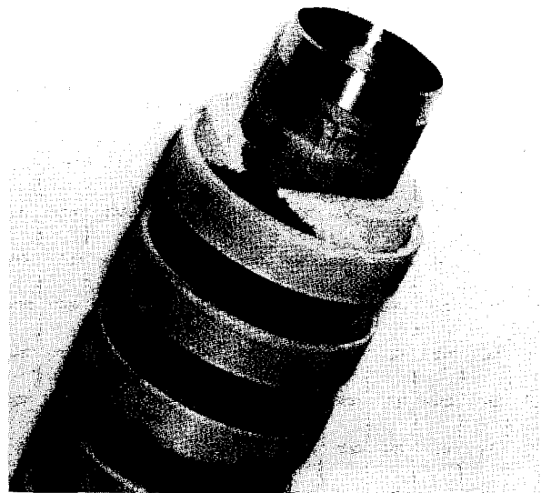
Fig. 1. End configuration of ISA dipole. The 30 and 50 correction windings are built into the central tube.
