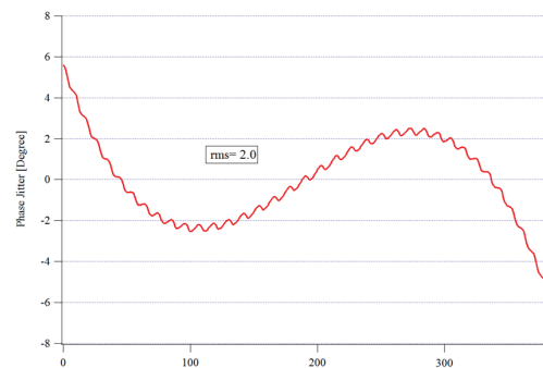
Figure 3: Calculated phase jitter when the undulator girder is deformed by 30 \mu\text{m} in parabolic shape. The girder is expected to be flat at the tuning gap and deforms when gap is changed from the tuning gap.
