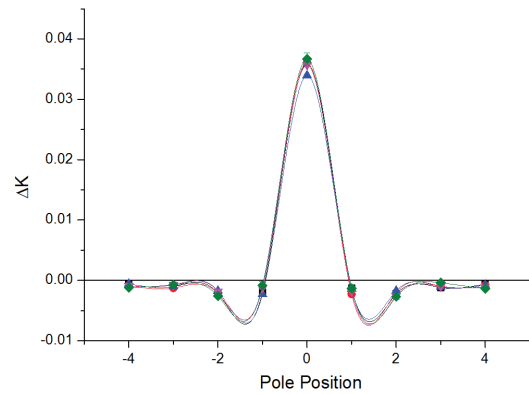
Figure 1: The measured local K changes due to a 100 \mu\text{m} pole correction at the 9.5 mm tuning gap. The abscissa denotes the distance to the pole: 0 is the tuned pole itself, \pm 1 the two next neighbouring poles etc.
