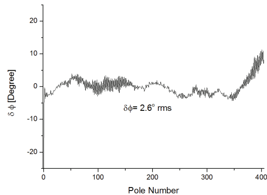
Figure 2: Optical phase error at the working gap of 9.5 mm. The rms phase jitter is 2.6 degree which is within the specification of 7.0 degree.
