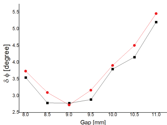
Figure 4: Optical phase change with the gap. The change in optical phase error mostly comes from the girder deformations. Two independent measurements are shown to express the measurement accuracy of the optical phase error.
