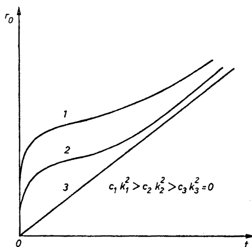
Fig. 6. The radius of a circle of indefinite temperature as a function of time
