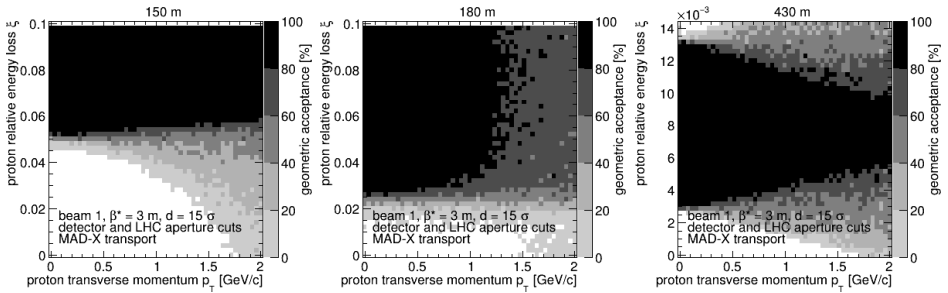
Fig. 4. Geometrical acceptance for three possible detector locations. Considered limitations: shape of the beam chamber, detector geometry and detector–beam distance. Please note a different vertical scale on the right plot.
