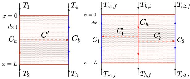
Figure 2: Two-(left) and three-way (right) heat exchanger.
