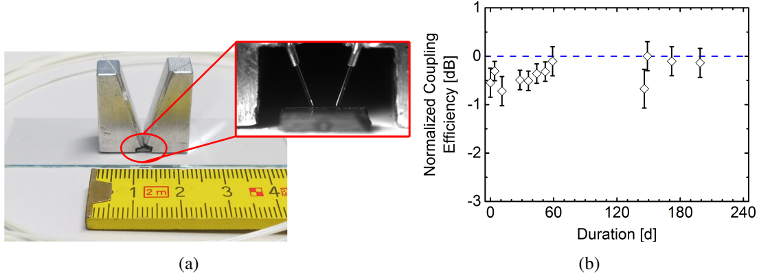
Figure 4. Setup and result of a preliminary fiber-to-chip coupling arrangement. Photograph of the assembly, with a close-up of the fibers aligned towards the grating couplers of a PIC (a). Long-term coupling efficiency normalized to the highest coupling value (b). The total insertion loss of the PIC test structure is 16 dB.
