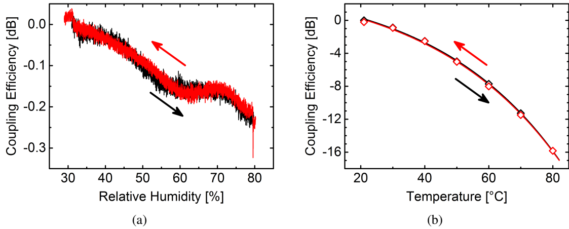
Figure 5. Relative coupling efficiency of the preliminary fiber-to-chip coupling arrangement as a function of ambient humidity (a) and temperature (b). The black curves represent the measured efficiency during the continuous increase of humidity or temperature, respectively, while the red curve is obtained during the decrease.
