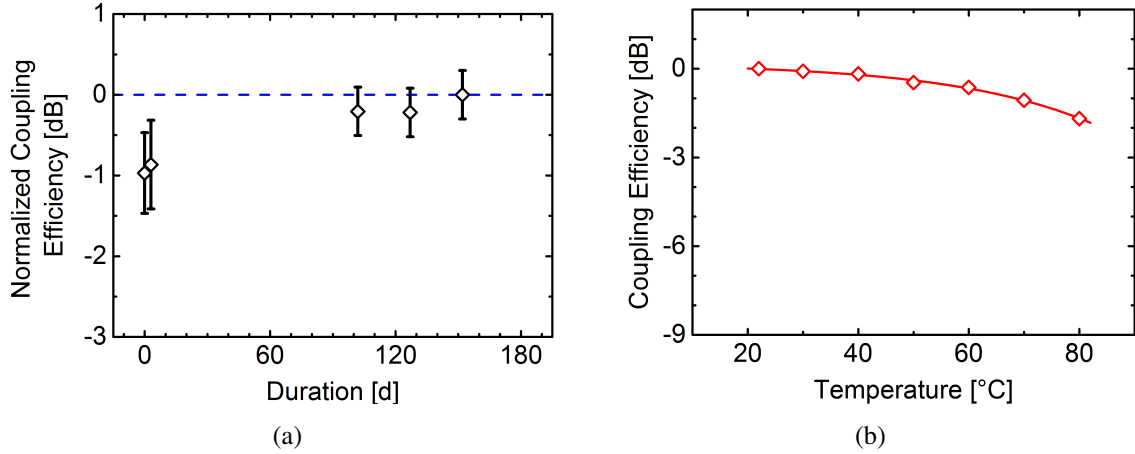
Figure 7. Measurement results of the planar fiber-to-chip coupling arrangement. Long-term coupling efficiency normalized to the highest coupling value (a). Relative coupling efficiency as a function of the ambient temperature (b). The total insertion loss of the PIC test structure is 13 dB.
