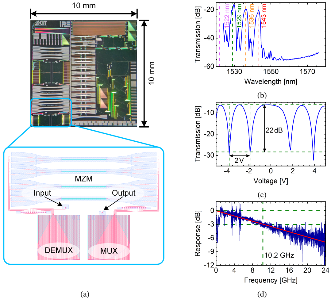
Figure 2. Microscope image of a photonic chip with three transmitter units one underneath the other on the left-hand side and an excerpt of the mask layout for a detailed view (a). Transmission spectrum of the entire transmitter unit (b). Steady-state transmission characteristic (c) and electrical-optical-electrical (EOE) response (d) of one of the integrated MZM.
