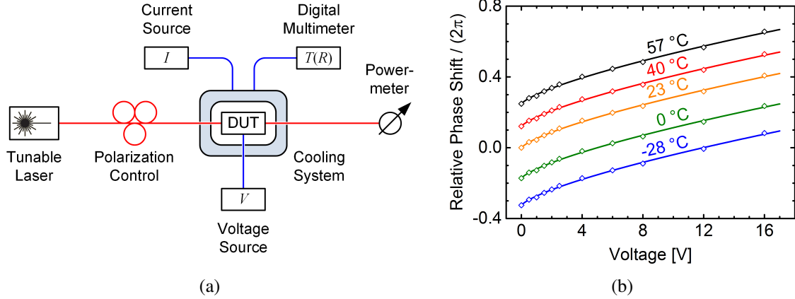
Figure 3. Sketch of the temperature characterization setup (a). Steady-state modulation efficiency represented by the relative phase shift as a function of bias voltage at different temperatures. All values are normalized to the phase at 0 V and room temperature (b). The systematic error in the order of less than 0.1 is suppressed for clarity.
