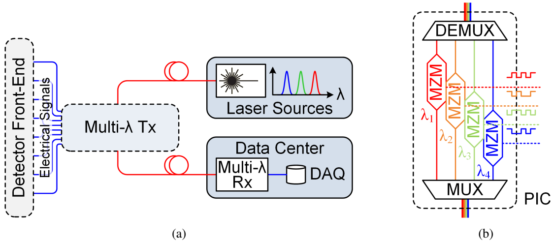
Figure 1. Schematic of the envisioned optical data transmission for HEP detectors. An off-detector laser source generates multiple optical carriers on which the on-detector transmitter encodes electrical signals from the detector front-end (a). Detailed schematic of the integrated four-channel transmitter (b).
