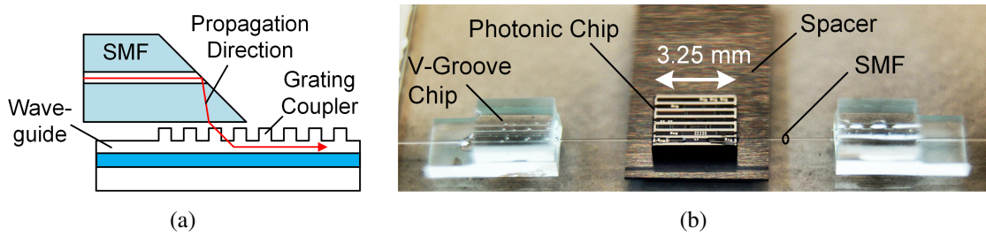
Figure 6. Functional principle (a) and a photograph (b) of a fiber-to-chip coupling arrangement with angle-polished fibers to provide for a planar arrangement.
