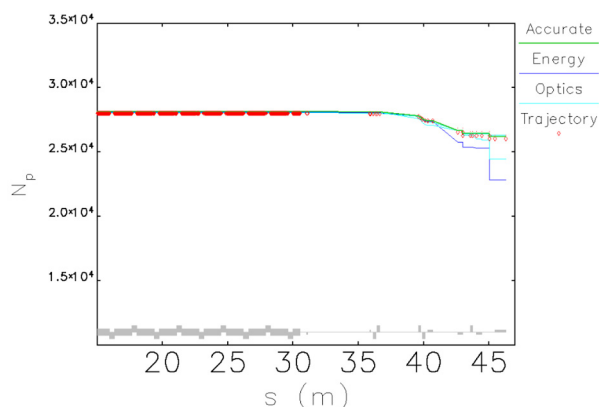
Figure 4: Beam losses in the electron injection channel.
