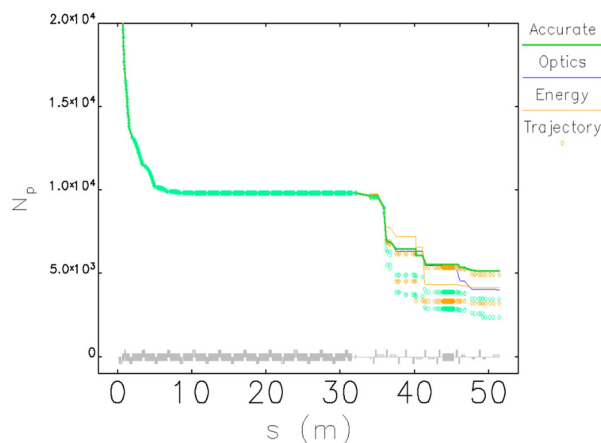
Figure 3: Beam losses in the positron injection channel. Thick green line is for the best optimized beam transportation with no errors.
