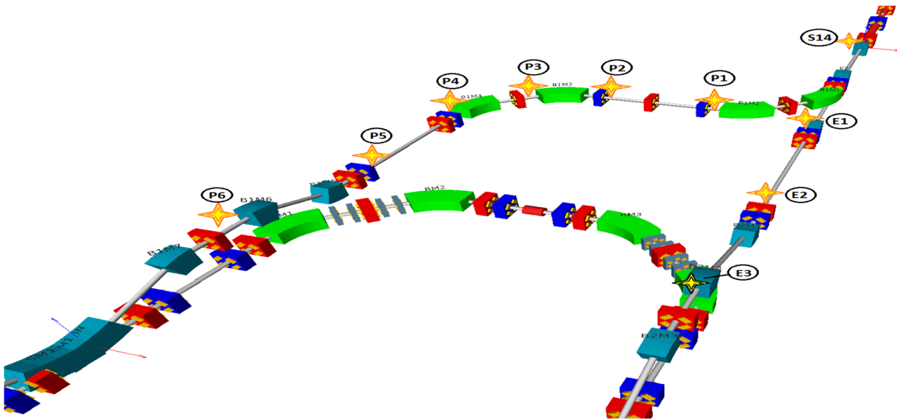
Figure 2: Possible placement of the monitors. The locations which are suitable to place the new BPMs indicated with yellow stars. Letter 'P' assigned for the positron injection channel, letter 'E' - for electron injection channel. Monitor named 'S14' is located at the last accelerating section of Preinjector.
